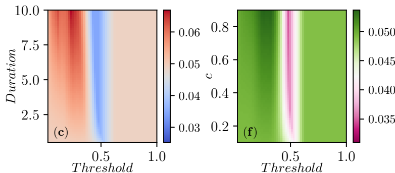
Figure 8: Contour plots of the peak prevalence, I_{peak} , that is the maximum value achieved by I(t) = \frac{1}{N} \sum_i I_i(t) during the time-course of the epidemic. Control strategies and setup the same as in Figure 5.
