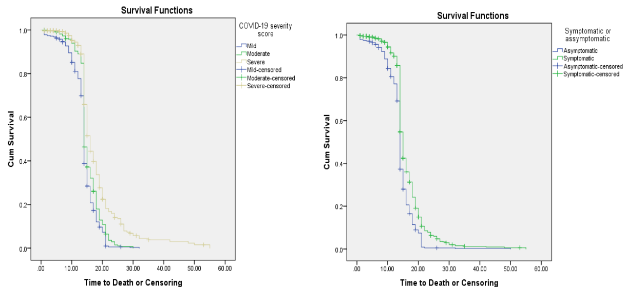
Figure 2: Survival functions for COVID severity and Presence of symptom by time
