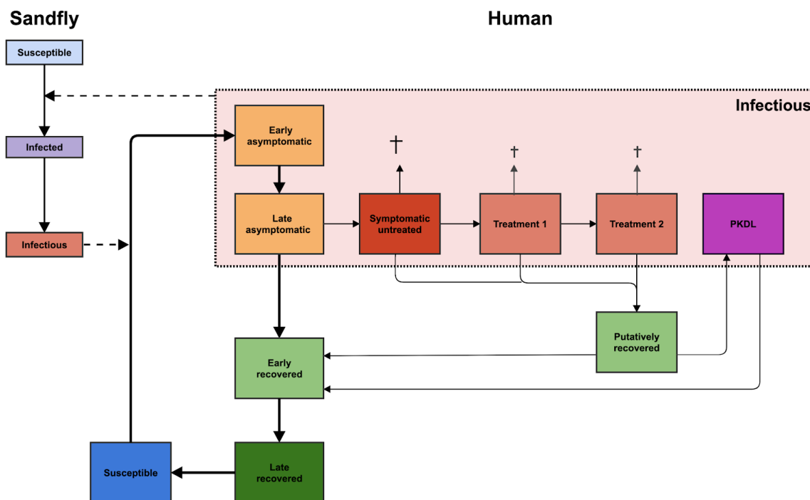
Figure S1. Schematic presentation of the structure of model E1 and the related model E0. For model E1, asymptomatic individuals (yellow compartments) are the main contributors to transmission. Model E0 has the same structure as model E1, but asymptomatic individuals do not contribute to transmission. Both models have different durations of infection stages from fitting to data, which are listed below in Chapter 3 Model parameters.
