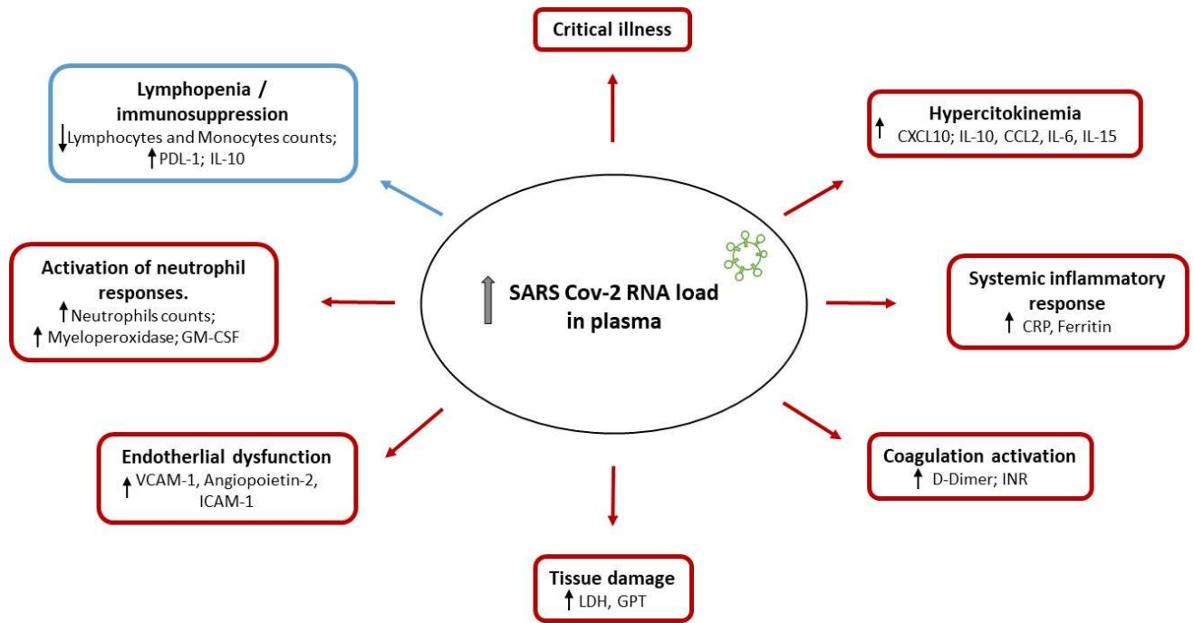
610 Figure 5: Integrative model depicting the correlations found between the 611 indicators of host dysregulated responses and SARS-CoV-2 RNA load in plasma.
