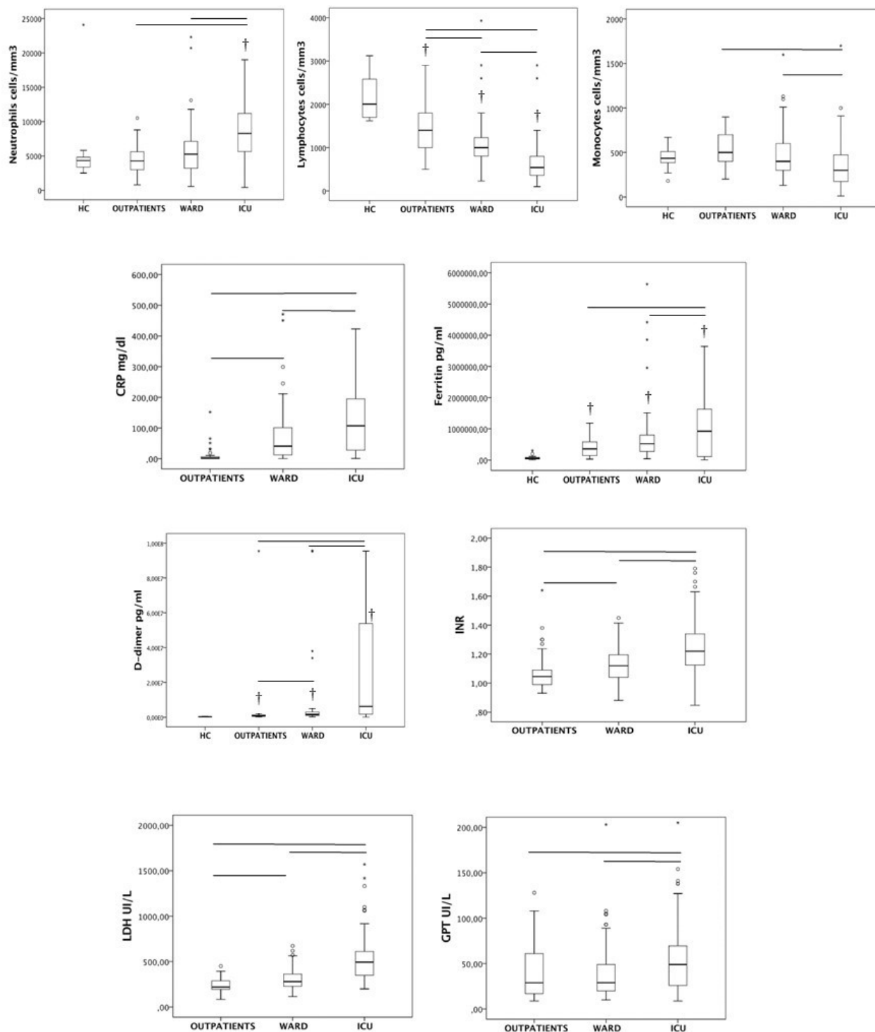
606 Figure 4: Levels of laboratory parameters indicating host dysregulated response 607 across groups. † indicates significant difference with the healthy control and the bars 608 significant differences between the other groups.
