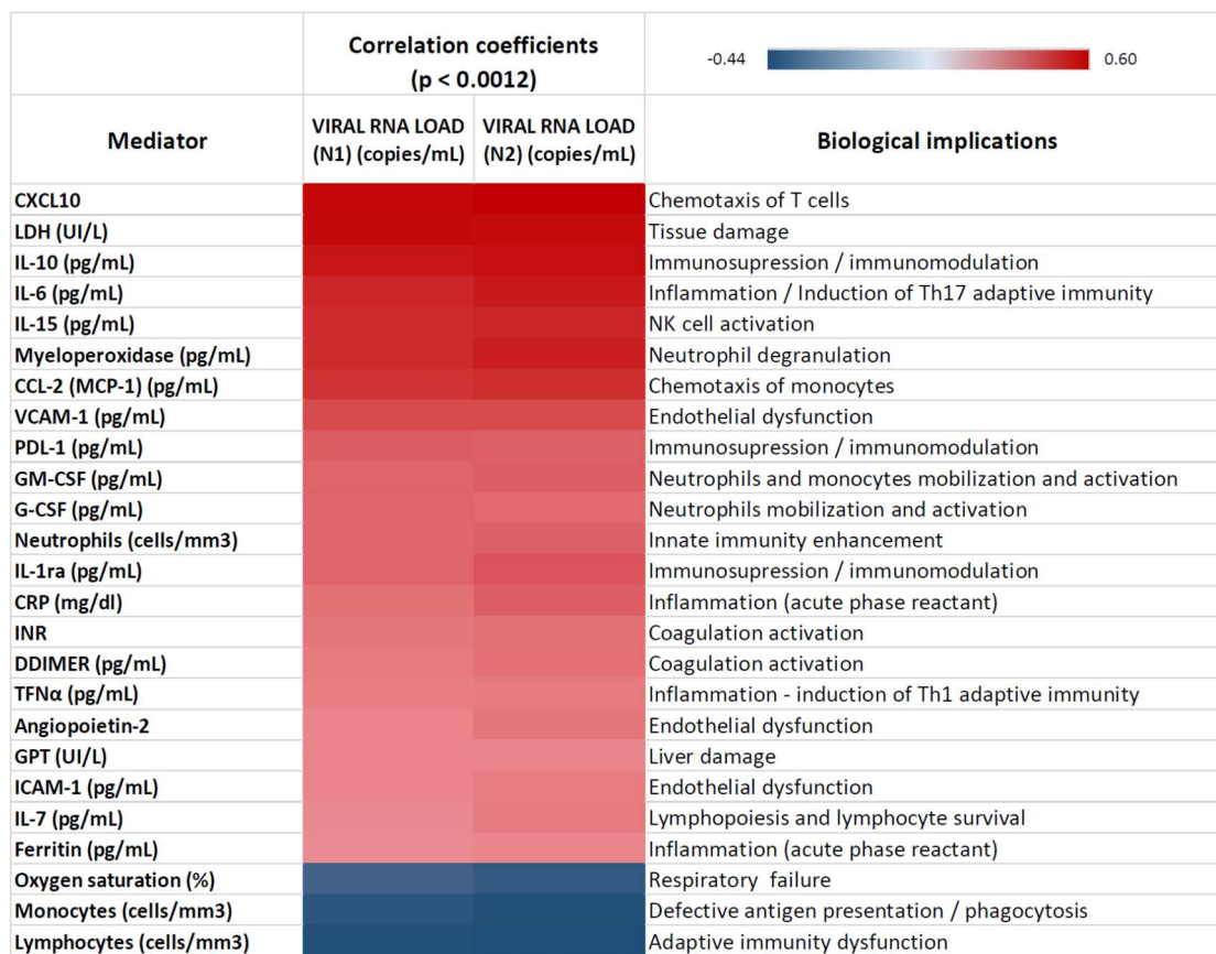
590 Figure 2. Heat map representing the Spearman correlation coefficients between 591 viral RNA load in plasma targeting the N1 and the N2 regions and representative 592 indicators of host dysregulated response.
