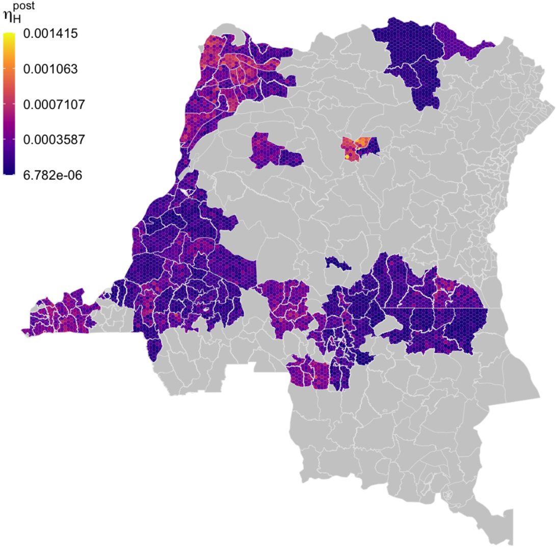
Figure S2.3: Within health zone posterior distribution of \eta_H^{\text{post}} , treatment rate from stage 1, 1998 onwards. fill colours are a randomly sampled from the posterior distribution for the health zone.
