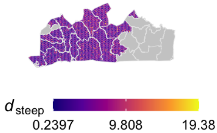
Figure S2.14: Within health zone posterior distribution of d_{\text{steep}} , the speed of improvement in passive detection rate, for the former province of Bas Congo, fill colours are randomly sampled from the posterior distribution for the health zone.
