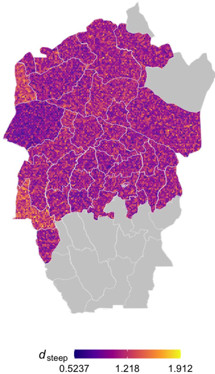
Figure S2.11: Within health zone posterior distribution of d_{\text{steep}} , the speed of improvement in passive detection rate, for the former province of Bandundu, fill colours are randomly sampled from the posterior distribution for the health zone.
