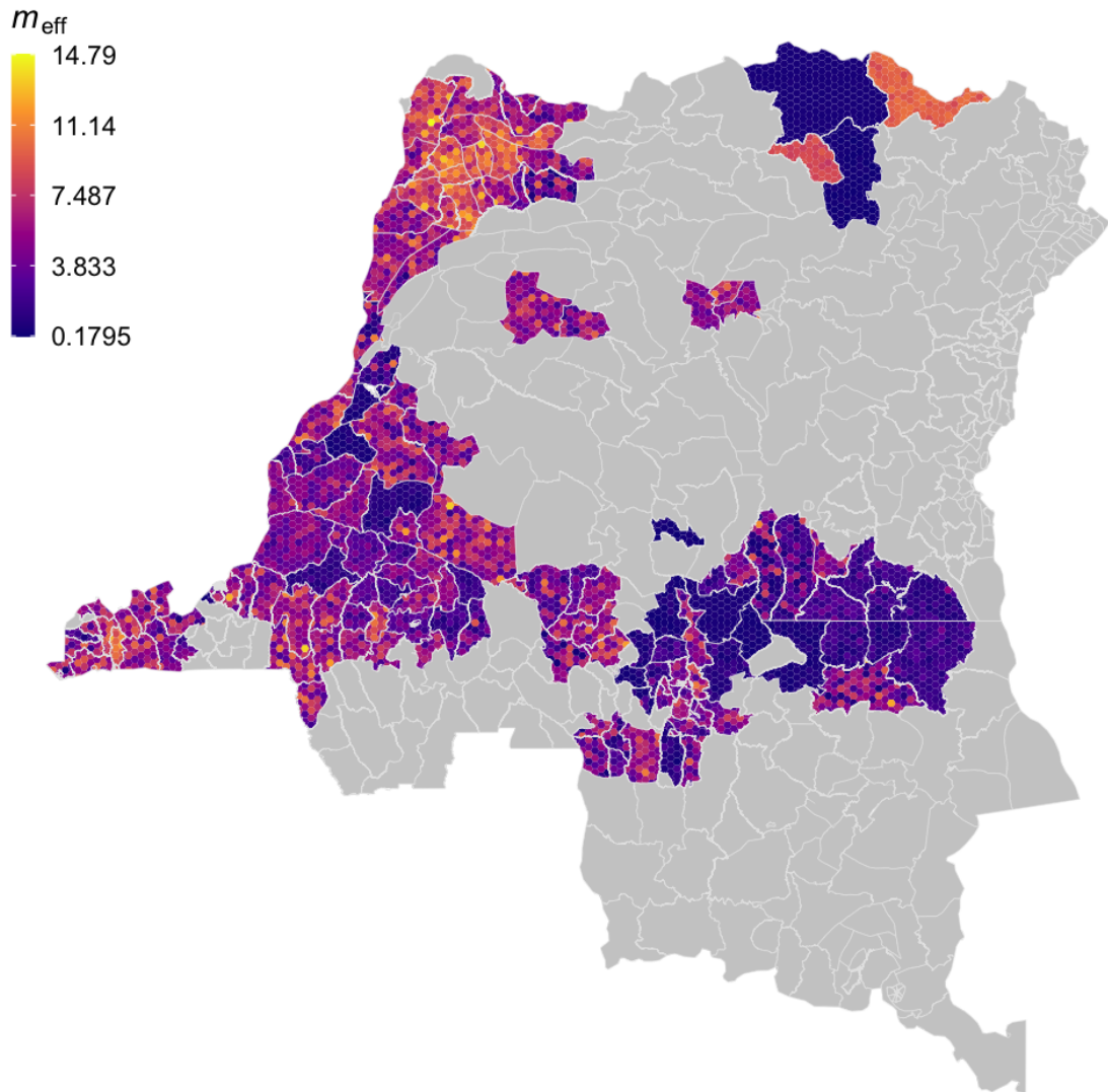
Figure S2.8: Within health zone posterior distribution of m_{\text{eff}} ; the effective, relative density of tsetse to humans. Fill colours are determined by randomly sampled values from the posterior distribution of m_{\text{eff}} from the analysis of the health zone.
