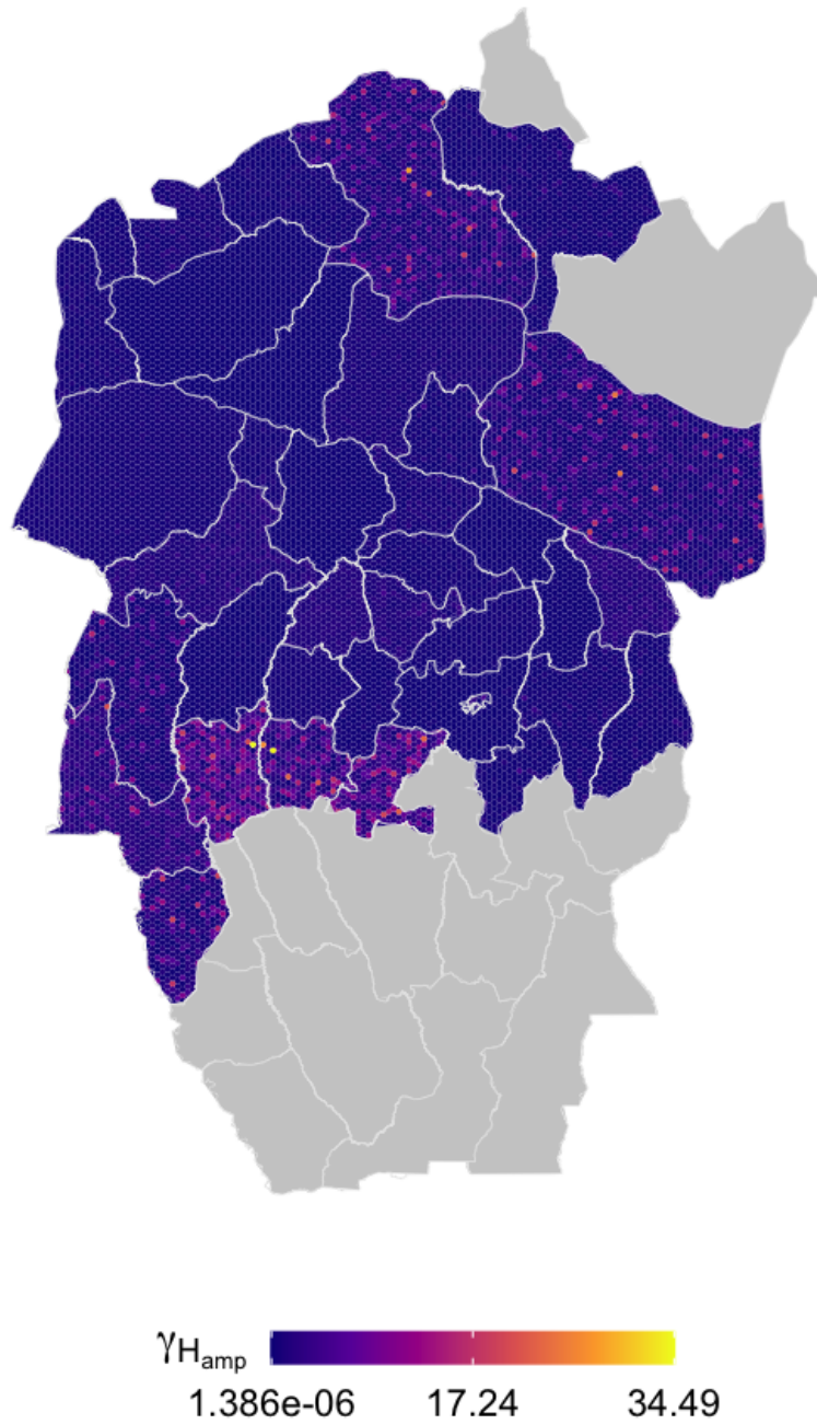
Figure S2.13: Within health zone posterior distribution of \gamma_{H_{amp}} , the relative improvement in passive stage 2 detection rate, for the former province of Bandundu, fill colours are randomly sampled from the posterior distribution for the health zone.
