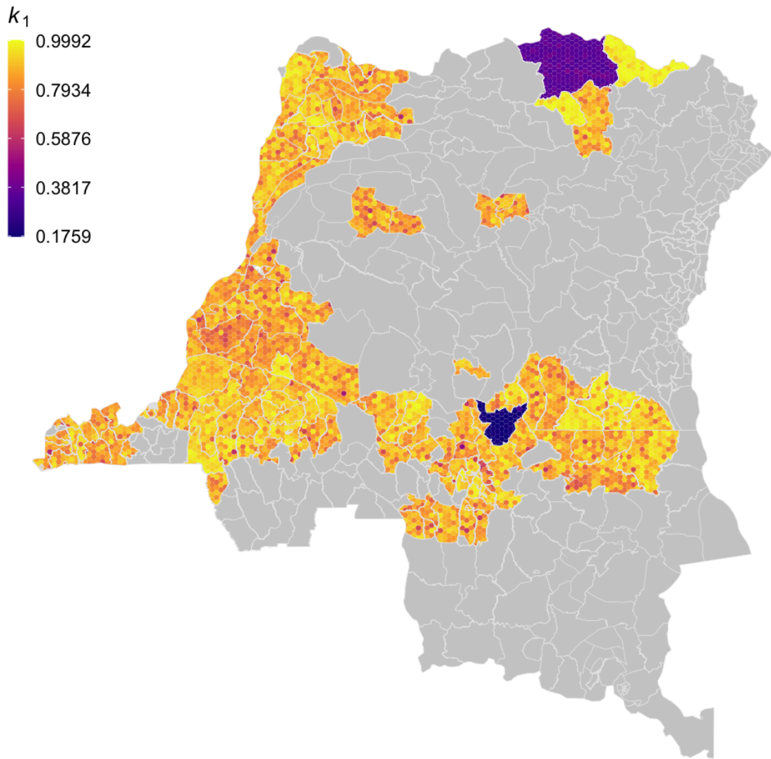
Figure S2.7: Within health zone posterior distribution of k_1 , the proportion of low-risk people. The fill colours are randomly sampled from the posterior distribution for the health zone.
