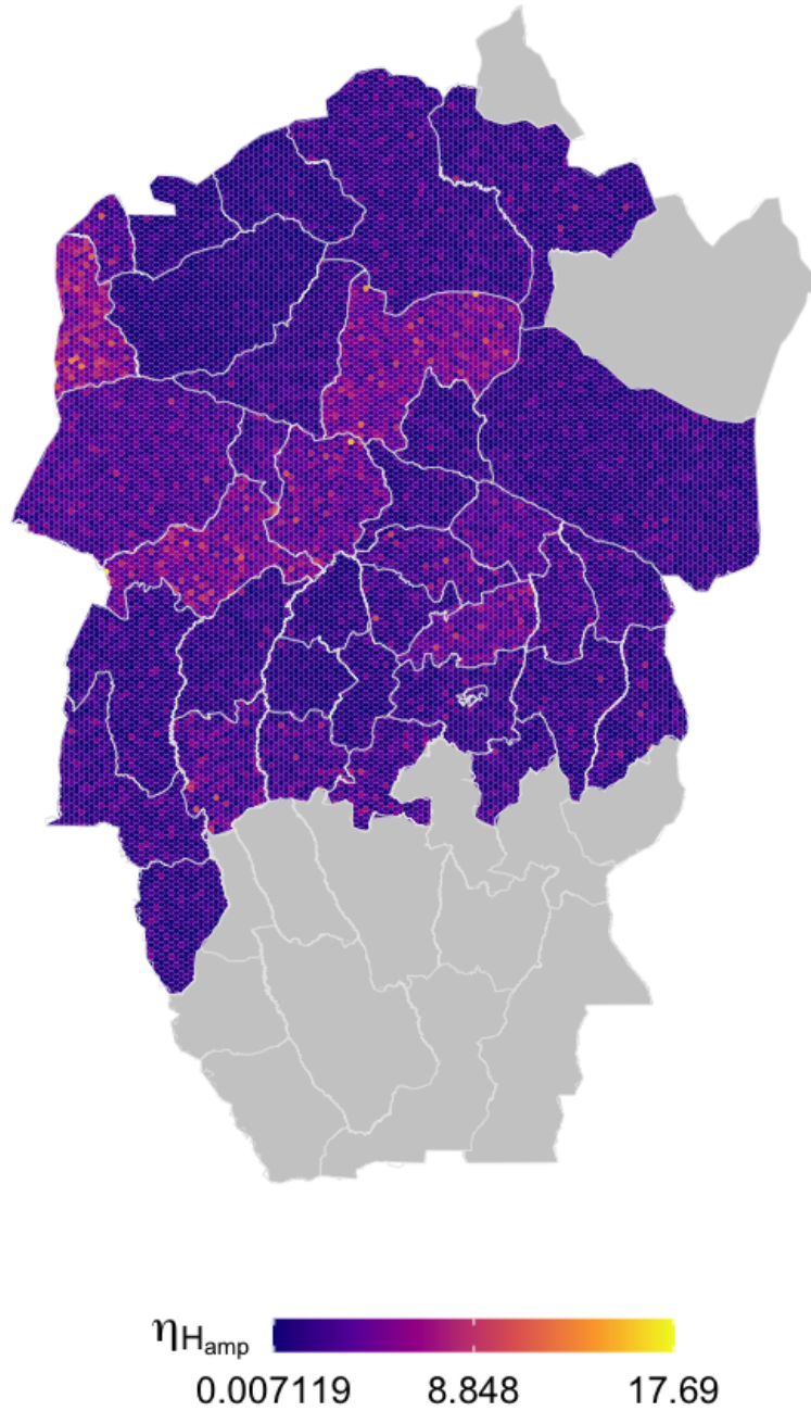
Figure S2.12: Within health zone posterior distribution of \eta_{H_{amp}} , the relative improvement in passive stage 1 detection rate, for the former province of Bandundu, fill colours are randomly sampled from the posterior distribution for the health zone.
