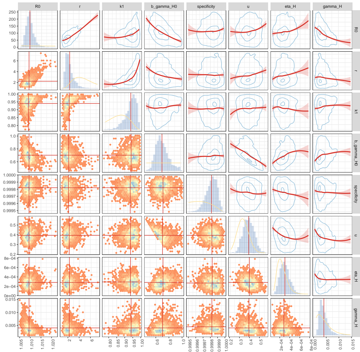
Figure S2.2: Joint posterior distributions for Tandala health zone in the former Equateur province.
