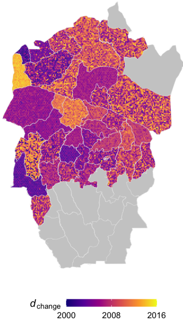
Figure S2.10: Within health zone posterior distribution of d_{\text{change}} , the midpoint year for passive improvement, for the former province of Bandundu. Fill colours are randomly sampled from the posterior distribution for the health zone.
