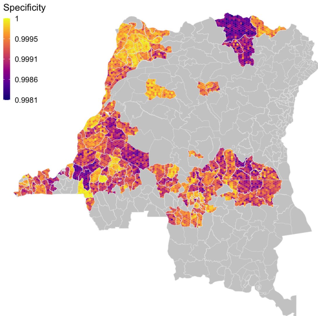
Figure S2.5: Within health zone posterior distribution of the specificity of the diagnostic algorithm, fill colours are a randomly sampled from the posterior distribution for the health zone.
