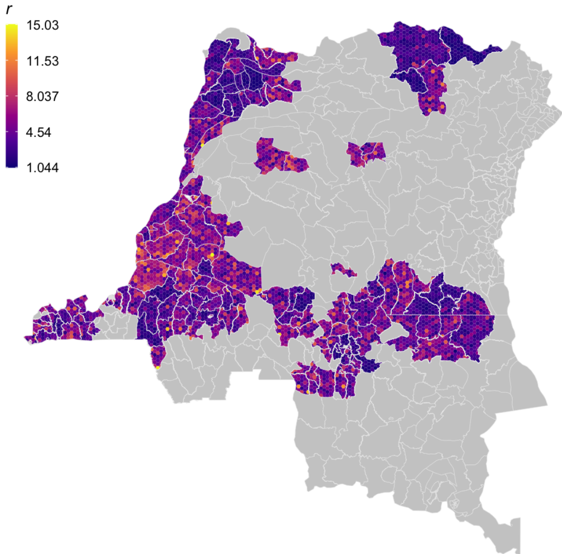
Figure S2.9: Within health zone posterior distribution of r , the relative bites taken on high-risk humans. Fill colours are determined by randomly sampled values from the posterior distribution of r from the analysis of the health zone.
