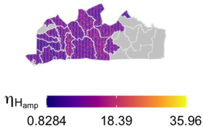
Figure S2.15: Within health zone posterior distribution of \eta_{H_{\text{amp}}} , the relative improvement in passive stage 1 detection rate, for the former province of Bas Congo, fill colours are randomly sampled from the posterior distribution for the health zone.
