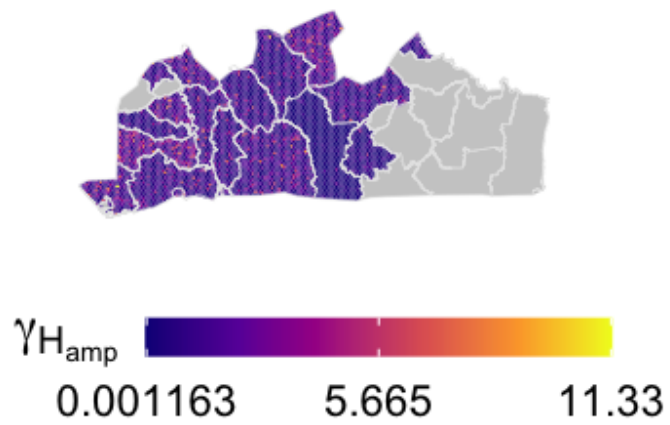
Figure S2.16: Within health zone posterior distribution of \gamma_{H_{amp}} , the relative improvement in passive stage 2 detection rate, for the former province of Bas Congo, fill colours are randomly sampled from the posterior distribution for the health zone.
