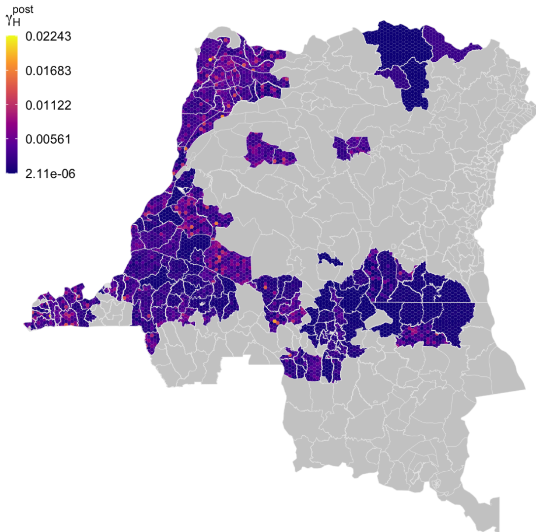
Figure S2.4: Within health zone posterior distribution of \gamma_H^{\text{post}} , the exit rate from stage 2 (treatment or death), 1998 onwards. The fill colours are a randomly sampled from the posterior distribution for the health zone.
