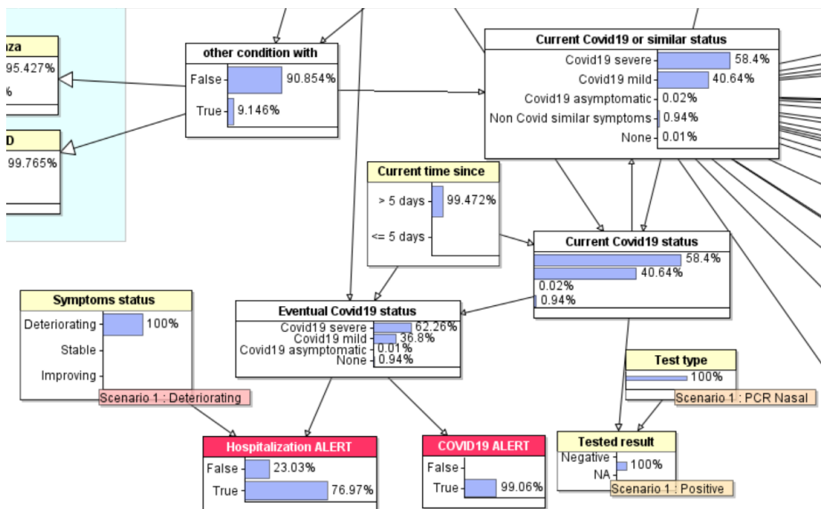
Fig. 8. Posterior probabilities of COVID-19 status nodes for observations from case study 1, with 'test type' observed.
