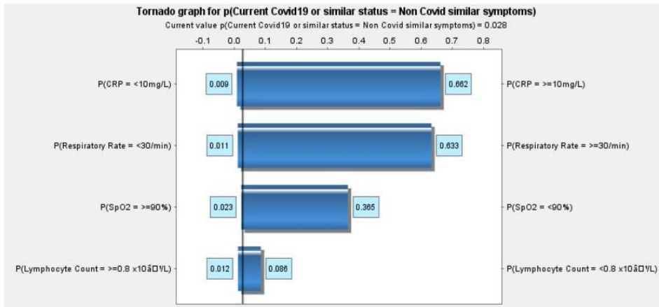
Fig. 6. Tornado graph representing the hierarchy of laboratory finding sensitivities to non-COVID infection.
