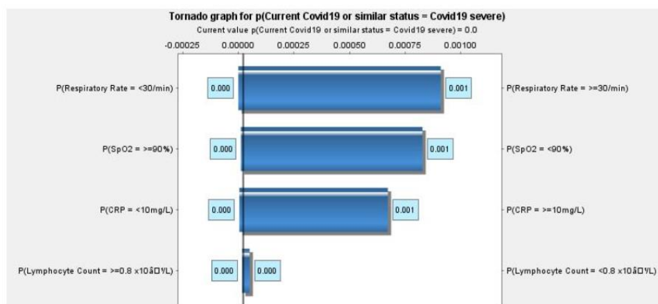
Fig. 5. Tornado graph representing the hierarchy of laboratory finding sensitivities to severe COVID-19 infection.
