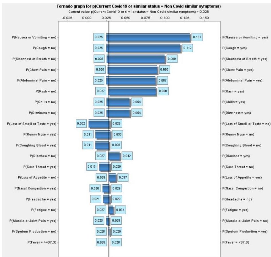
Fig. 4. Tornado graph representing the hierarchy of symptom sensitivities to non-COVID infection.
