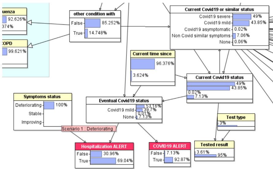
Fig. 7. Posterior probabilities of COVID-19 status nodes for observations from case study 1, with 'test type' not yet observed.
