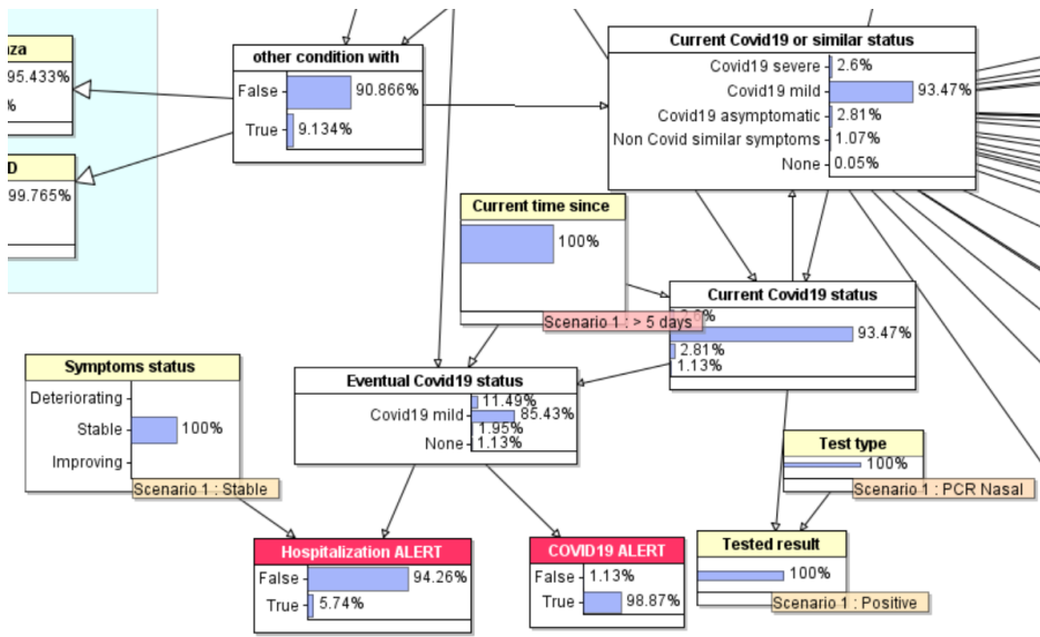
Fig. 9. Posterior probabilities of COVID-19 status nodes after respiratory recovery and during rash presentation, for case study 1.
