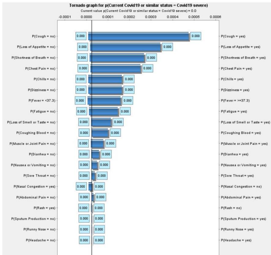
Fig. 3. Tornado graph representing the hierarchy of symptom sensitivities to severe COVID-19 infection.
