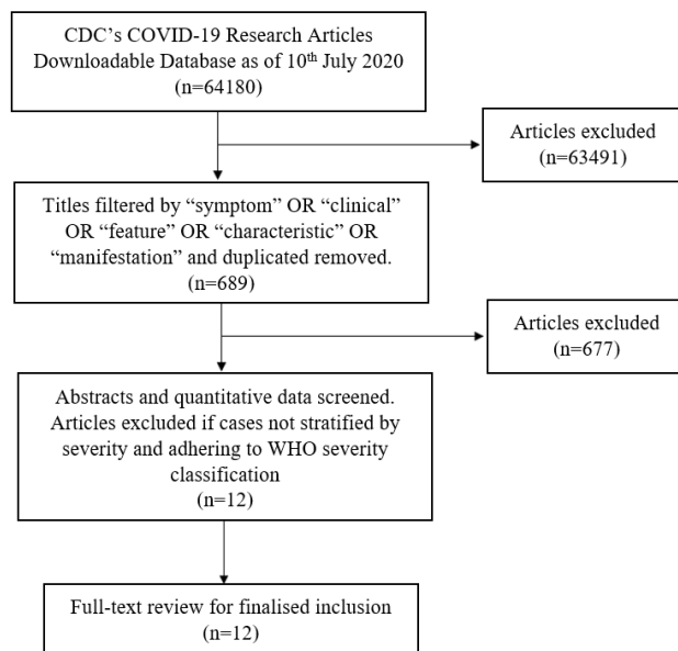
Fig. 1. Flowchart describing the inclusion criteria for the systematic review.
