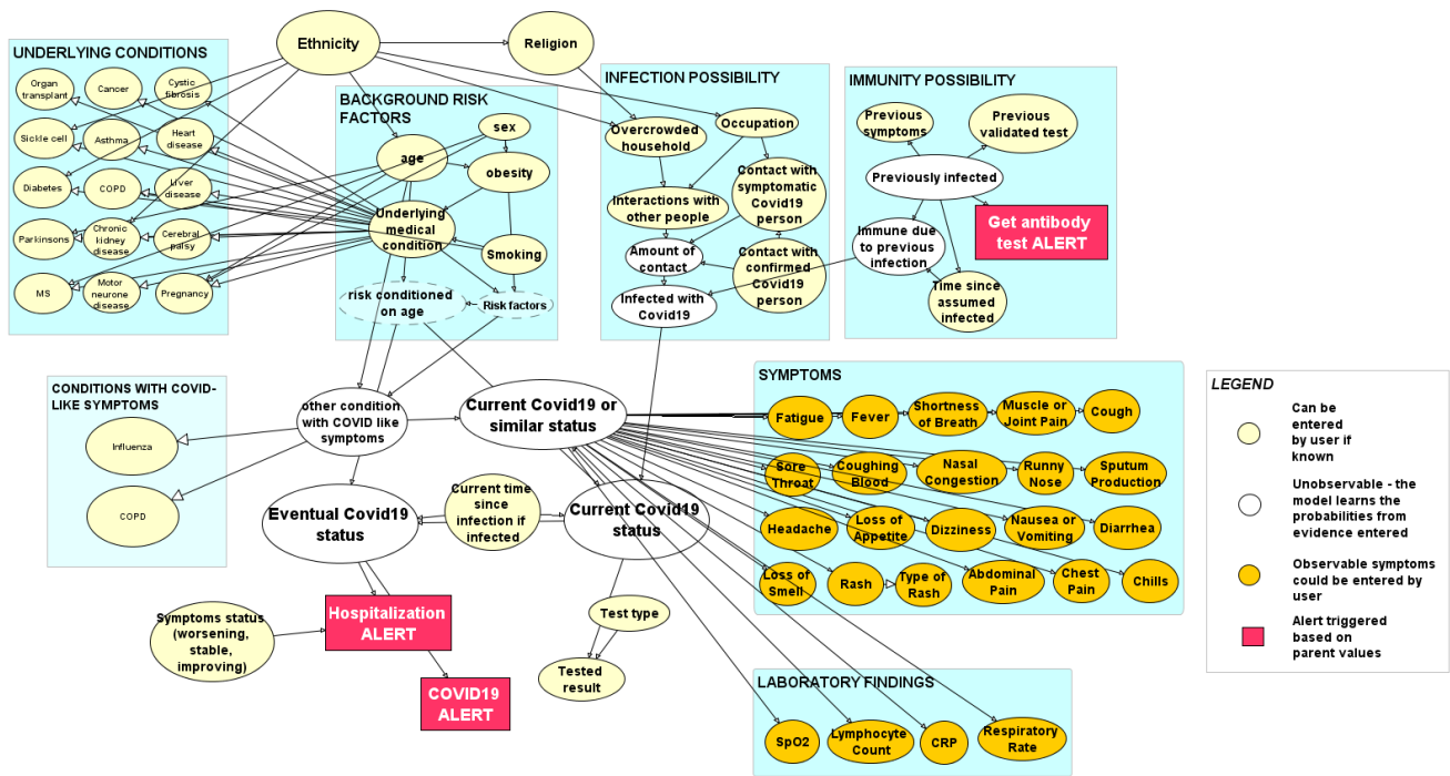
Fig. 2. Complete structure of proposed Bayesian network.
