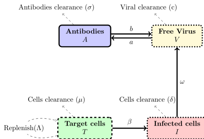
Figure 1: Graphical illustration of the flow in the model (1)-(5).
