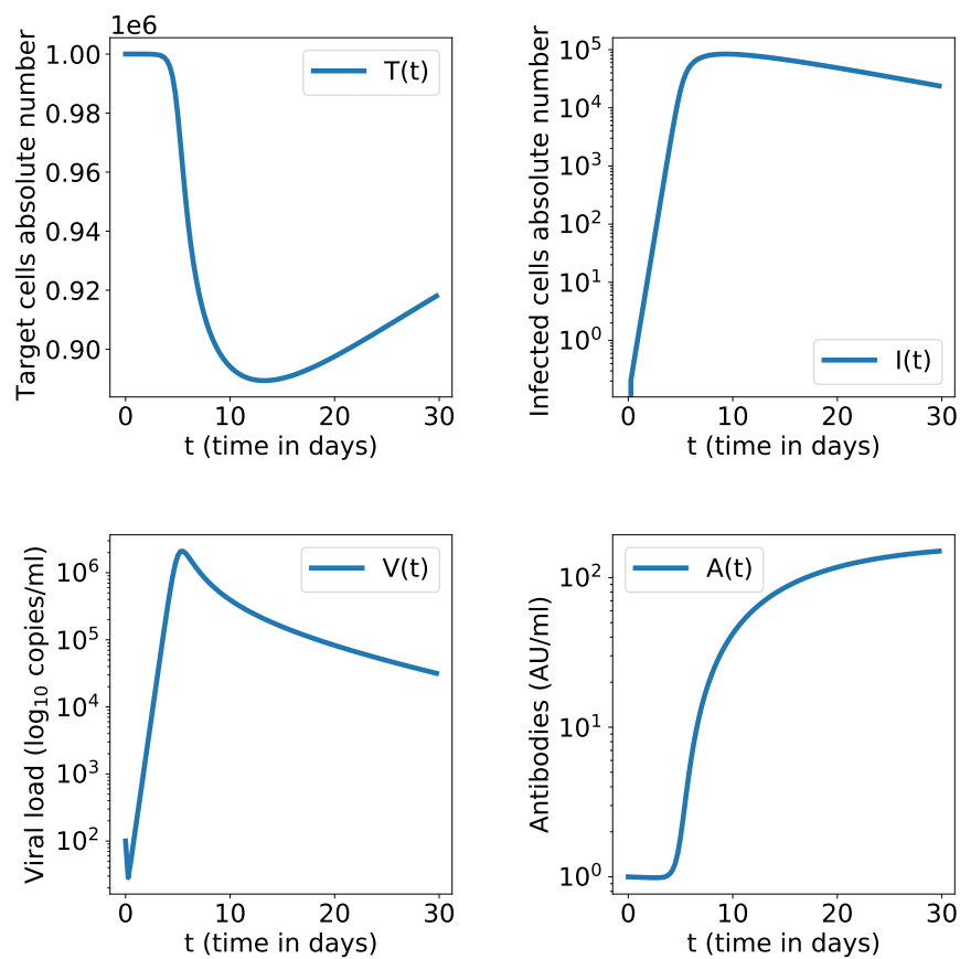
Figure 2: Numerical simulation of the first infection without ADE for model (1)-(4) and parameters in table 1.
