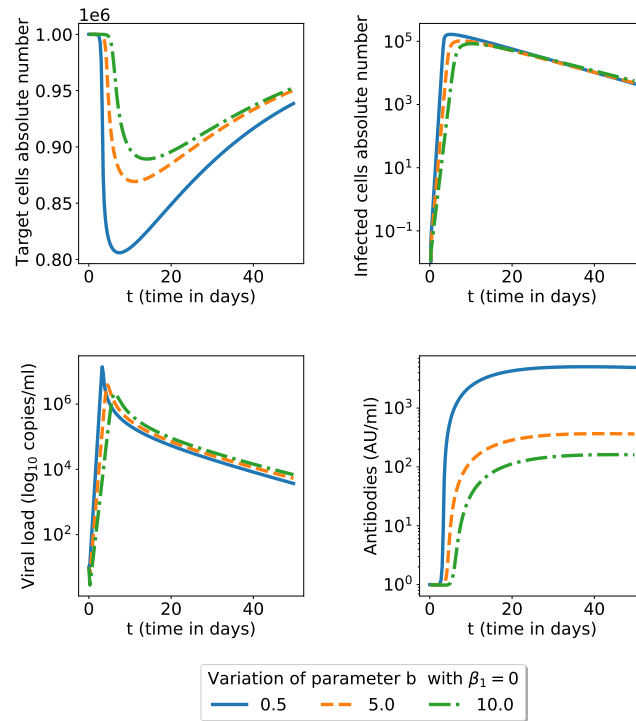
Figure 6: Initial infection for three possible values of the b parameter; the model is that in equations (1)-(4) and all other parameters have the nominal values in the table 1. We show here a zoom for the initial 50 days (see figure 7 for a longer time span).
