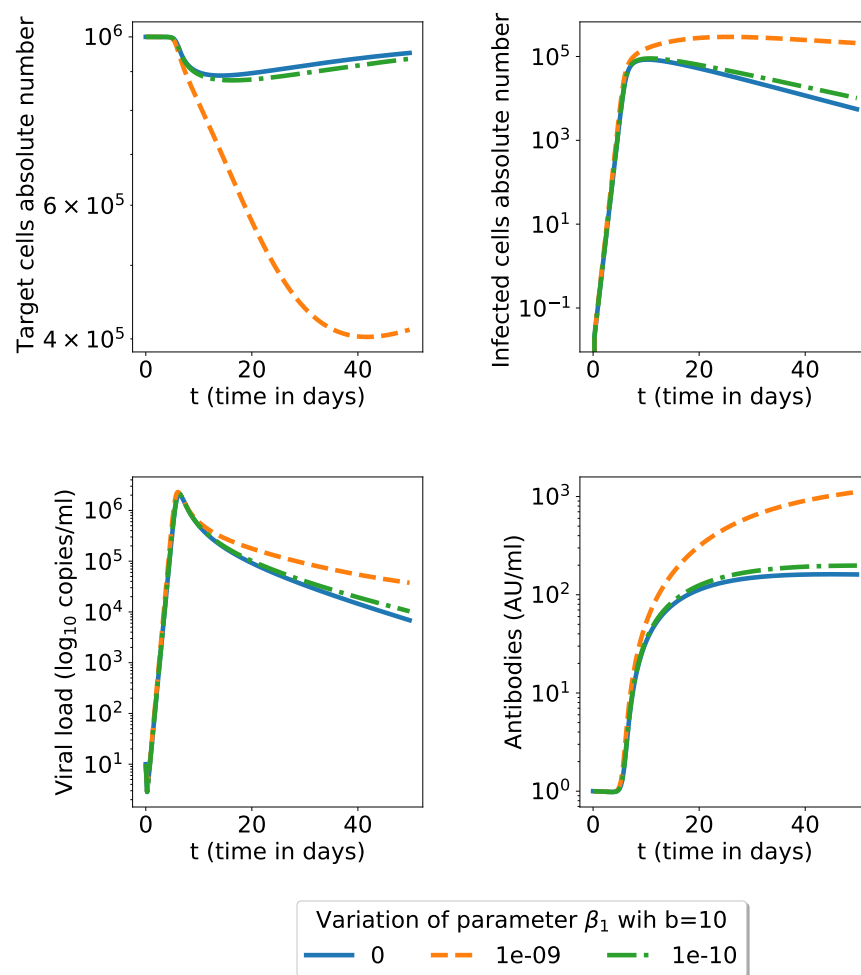
Figure 4: The effect of the ADE parameter \beta_1 (the model (1)-(4)). The secondary infection has fixed neutralizing antibodies capacity b but we investigate several \beta_1 (ADE) parameter values; for all other parameters we use the nominal values given in table 1.
