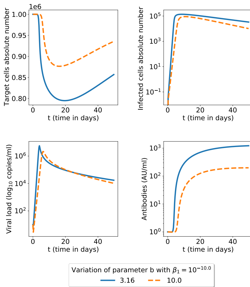
Figure 5: The effect of the neutralizing b parameter. The secondary infection has lower neutralizing antibodies capacity b = 3.16 . We fixed ADE parameter \beta_1 and considered all other parameters of the model (1)-(4) at their nominal values in table 1.
