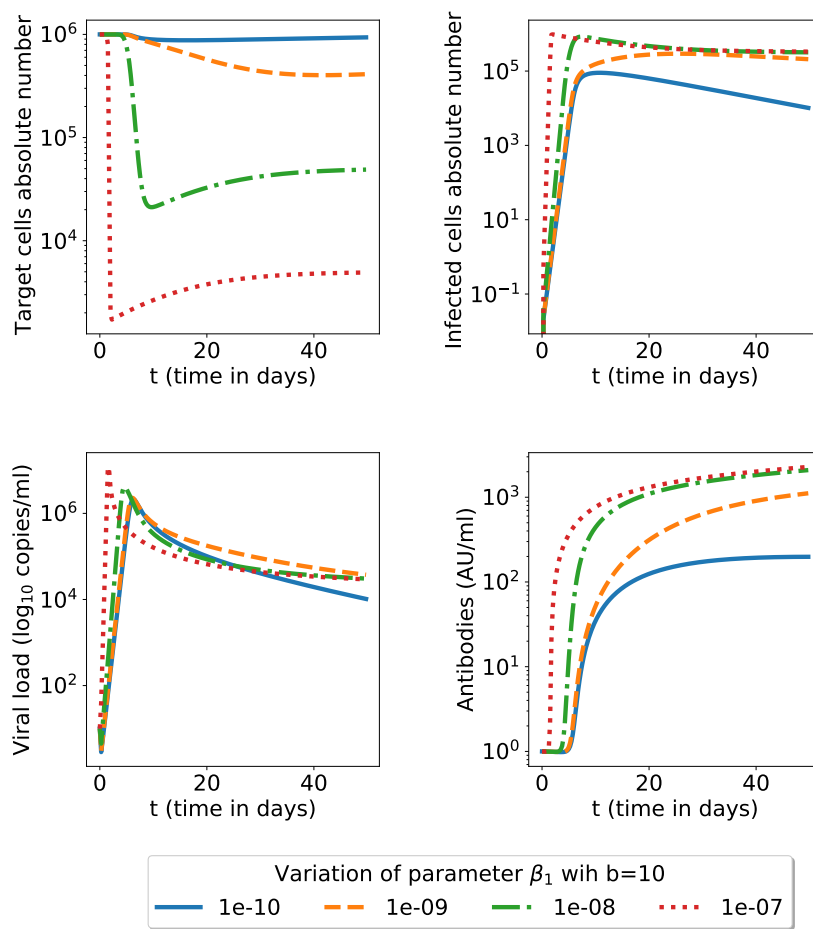
Figure 8: Secondary infection with ADE mechanism present for several values of the \beta_1 parameter; the model is that in equations (1)-(4) and all other parameters have the nominal values in the table 1. We show here a zoom for the initial 50 days (see figure 9 for a longer time span).
