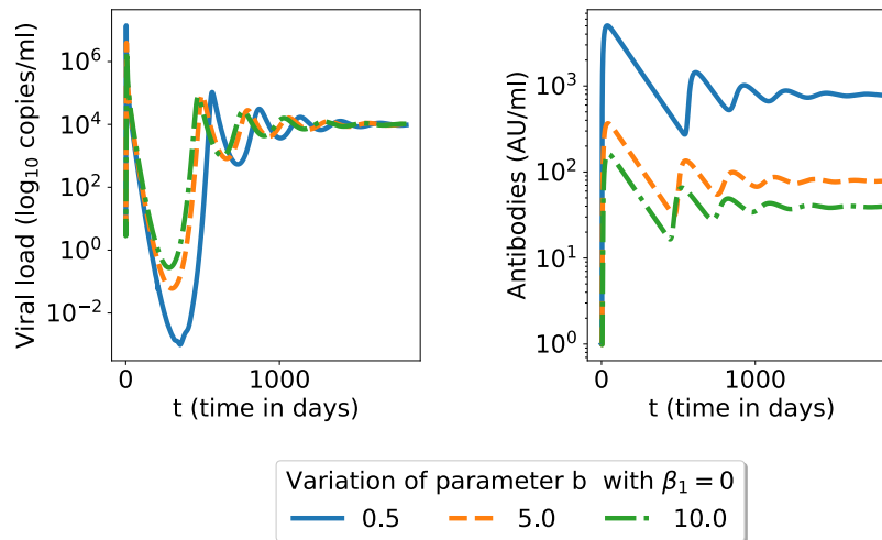
Figure 7: Simulation in 6 for a longer time span.
