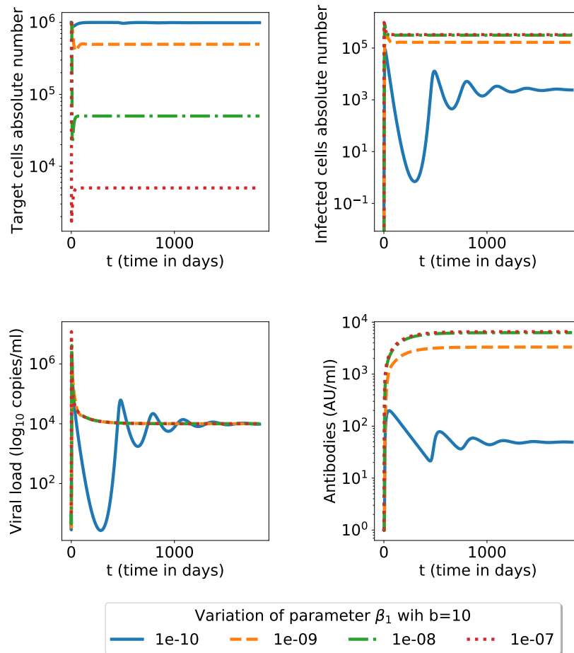
Figure 9: Simulation in 8 for a longer time span
