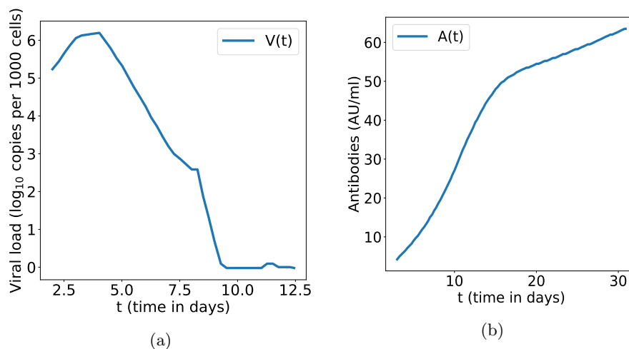
Figure 3: 3a : Clinically observed typical variation of SARS-CoV-2 viral load in nasopharyngeal swab normalised using cell quantification. Data taken from [32, figure 3 page 703]. 3b : Typical time variations for IgG. Data taken from [36, figure 2 page 1085].
