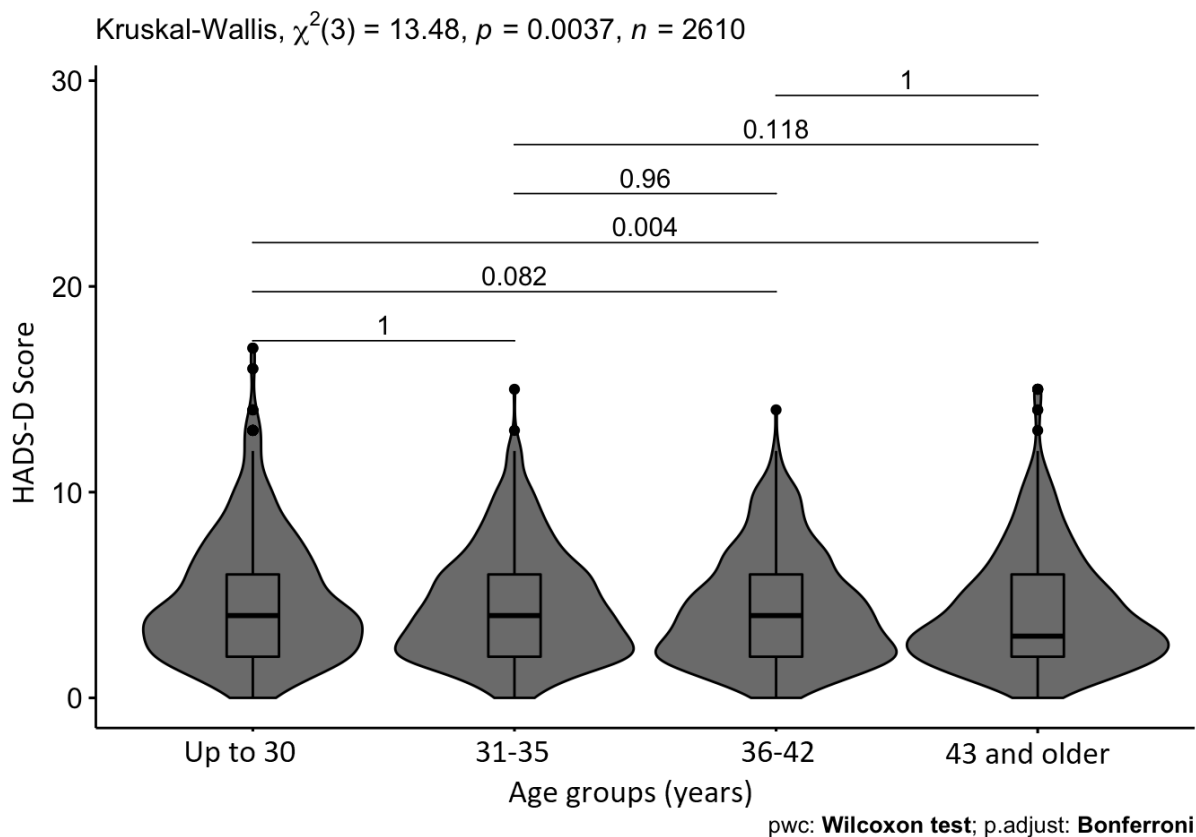
Fig. 1. Box-plots and violin-plots of differences between age groups
