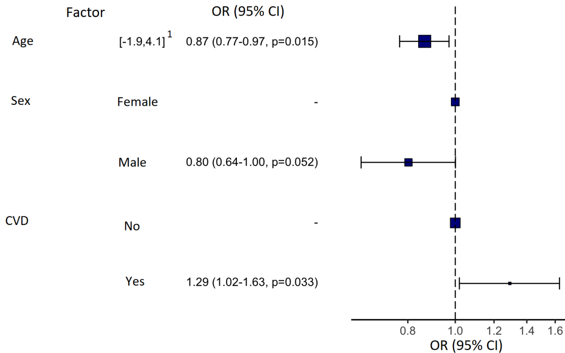
Fig. 2. Results of binary logistic regression for assessing the risk of having symptoms of clinical or subclinical depression according to HADS-D
