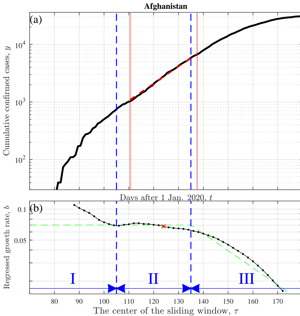
Figure S1. (a) Cumulative confirmed cases y as a function of time t and (b) its growth rate b against the regression time parameter \tau , for Afghanistan as an example. The growth rate b (black line in (b)) is regressed according to the model y = ae^{b(t-\tau)} in a 28day-wide sliding window centering at \tau=88, 90, \dots, 172 , where a represents the model initial confirmed cases (namely, the regressed y value at \tau ). The growth of confirmed cases could be divided into three stages: Phases I, II and III, separated largely by the vertical dashed blue lines. In Phase II, the growth is stable ( 0.060 < b < 0.075 ) whereas in the other two, b decreases by more than 0.04. In Phases II and III but not in Phase I, the realistic growth is largely consistent with the ideal evolution that is sketched as the green line in (b) according to, e.g. 1,2 . We attribute the discrepancy in Phase I to an insufficient test capability at early stage. In both panels, the red symbols denote the regression associated with the least-constrained growth rate, namely, the maximum b at a > 2500 (see "Methods"). Note that the conclusions of the current work are qualitative not subject to the window size here, learn from the same analyses but with different window sizes from 16 to 60 days (not displayed here).
