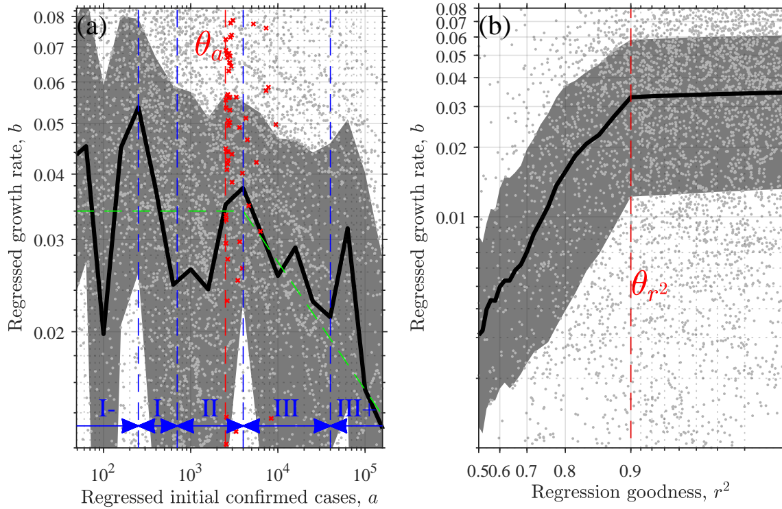
Figure S2. The growth rate b of the confirmed cases against (a) the regressed initial confirmed cases a and (b) the goodness r^2 of the exponential regression as instanced in Figure S1. In each panel, one dot corresponds to one sliding step of the regression; and the bold black solid line and gray shadow illustrate the median and the interquartile range, respectively. In (a), the blue lines suggest different stages of the evolution of the outbreak, whereas the green line sketches the ideal evolution according to, e.g. 2 . The stages I, II and III, corresponding to Phases I, II and III in Figure S1, which are characterized by insufficient test capability, least artificial constrains, and intense artificial controllers, respectively. Different from the stages I and III, the stages I- and III+ are not associated with rapid decreases in b . The stage I- is attributable to that the growth, at an early stage and with a small number of infections, does not follow the exponential law well but is susceptible to uncertainties, while the stage III+ might reflect the second wave of the outbreak occurred in some countries, e.g., 3 , after relaxing artificial controllers. In (a), the minima at a=100 and 10000 might be signatures of data manipulation, e.g., 4 , that governments might try to "control" the infection cases to cross the orders of magnitude. In (a), the red crosses denote the least-constrained growth rate b_m , each of which represents one country. The red lines display two threshold values, \theta_a = 2500 in (a) and \theta_{r^2} = 0.9 in (b). See "Methods" for the details.
