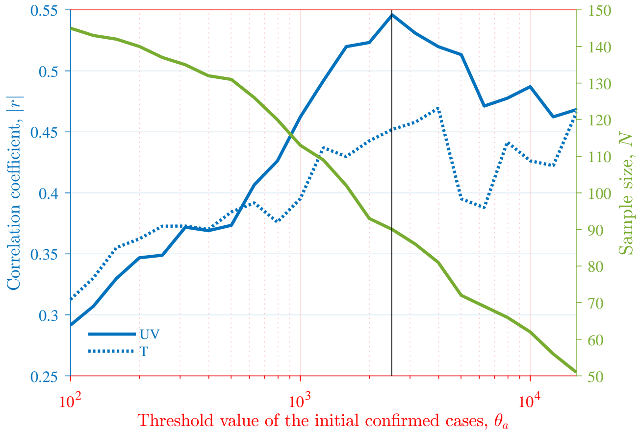
Figure S3. The absolute correlation coefficients |r| and valid sampling size N as a function of the threshold value \theta_a defined in Figure S2. \theta_a is the single-parameter of the optimization for determining the least-constrained growth rate. The black line represents solution of the optimization. See "Methods" for the details.
