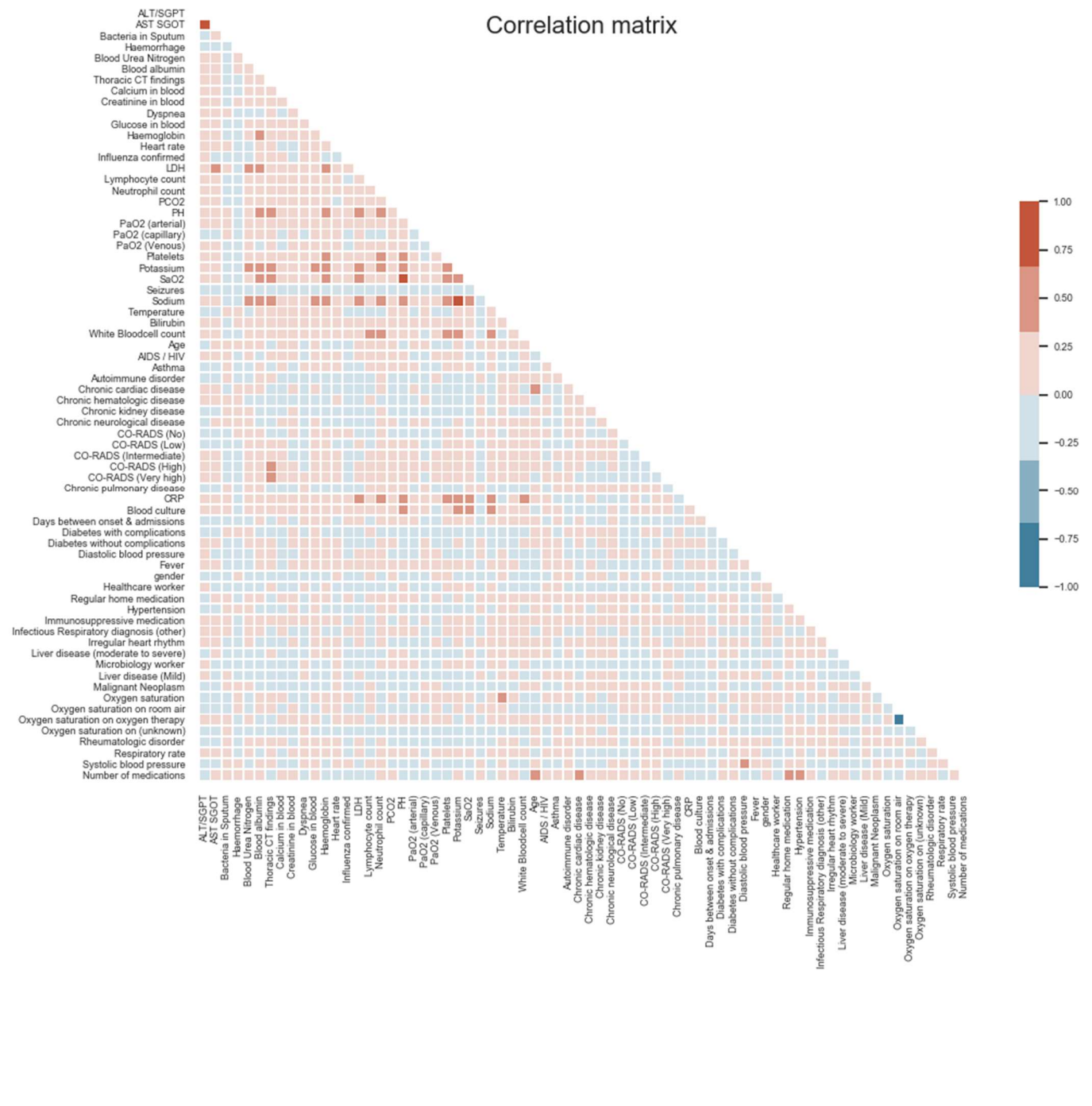
Supplementary figure 1 – Pearson correlation matrix of all features. No troublesome collinearity was seen.
