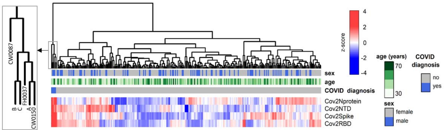
Supplemental Figure 4. Hierarchical clustering analysis according to antibodies against SARS-CoV-2 antigens. This figure combines data from 276 study participants plus the three COVID-19 convalescent sera. Colour scale represents antibody detection as a z-score.
