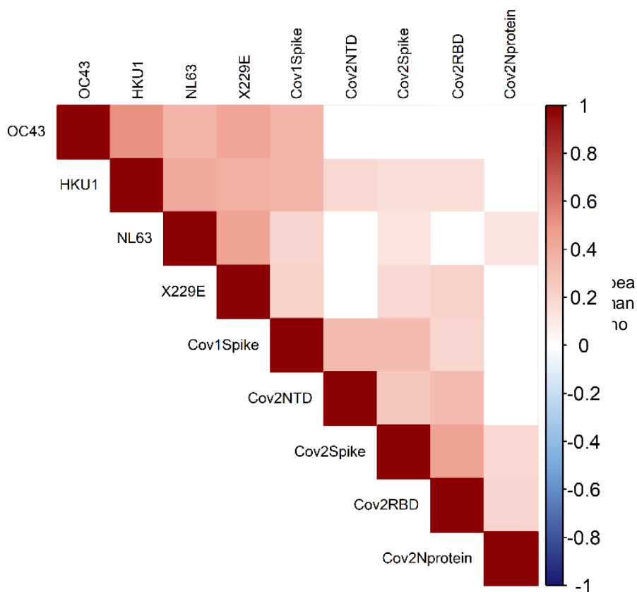
Figure 2. Correlations among SARS-CoV-2 and circulating coronaviruses antibody levels.
