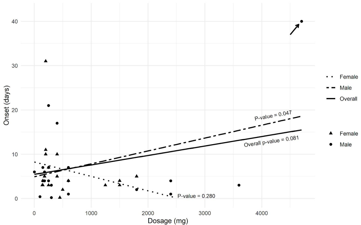
Figure S1: Distribution of drug dosage and the onset of psychiatric side effects with all case-reports. Arrow: highlighting the individual who took high drug dosage (4,700mg). P-value: result of linear regression.
