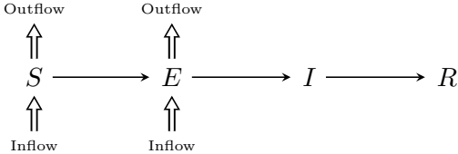
Figure S1: Flowchart of the human mobility flow-augmented stochastic SEIR model.
