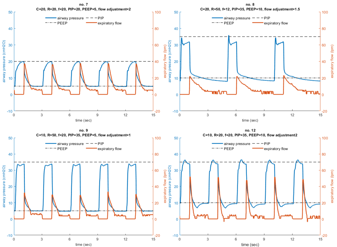
Fig. 5. Performance results of the ISO 80601-2-80-2018 pressure controlled ventilator standard tests with an intended delivered tidal volume of 300 mL. For each configuration the following parameters are listed: the test number (from table 201.105 in the ISO standard), the compliance (C, mL/cm H 2 O), linear resistance (R, cm H 2 O/L/s), respiratory frequency (breaths/min), peak inspiratory pressure (PIP, cm H 2 O), positive end-expiratory pressure (PEEP, cm H 2 O), and flow adjustment setting. PIP is reached in every test condition.
