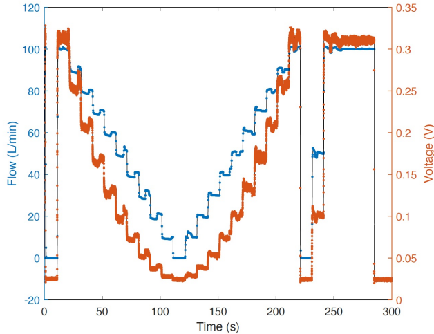
Figure S1. Calibration of the Flow Sensor. Flow introduced in steps of 10 L/min ranging from 10 L/min to 100 L/min. Blue points represent the flow measured by the mass flow controller and orange points represent the voltage recorded from the Diite sensor.
