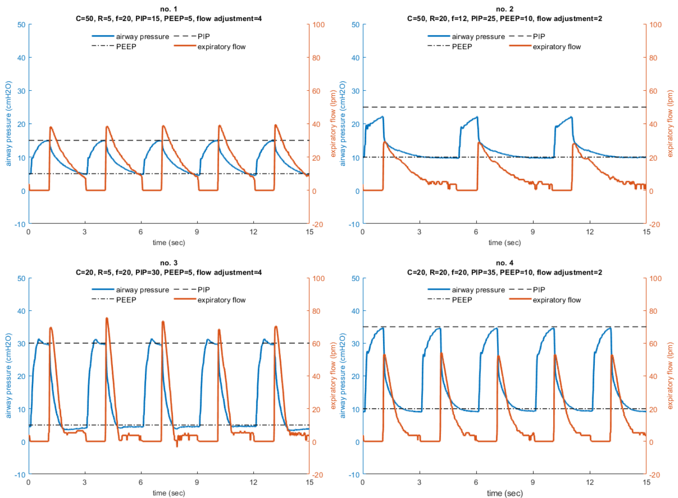
Fig. 4. Performance results of the ISO 80601-2-80-2018 pressure controlled ventilator standard tests with an intended delivered tidal volume of 500 mL. For each configuration the following parameters are listed: the test number (from table 201.105 in the ISO standard), the compliance (C, mL/cm H 2 O), linear resistance (R, cm H 2 O/L/s), respiratory frequency (f, breaths/min), peak inspiratory pressure (PIP, cm H 2 O), positive end-expiratory pressure (PEEP, cm H 2 O), and flow adjustment setting. PIP is reached in every test condition except for case 2, which is approximately 2.4 cm H 2 O below the set point.
