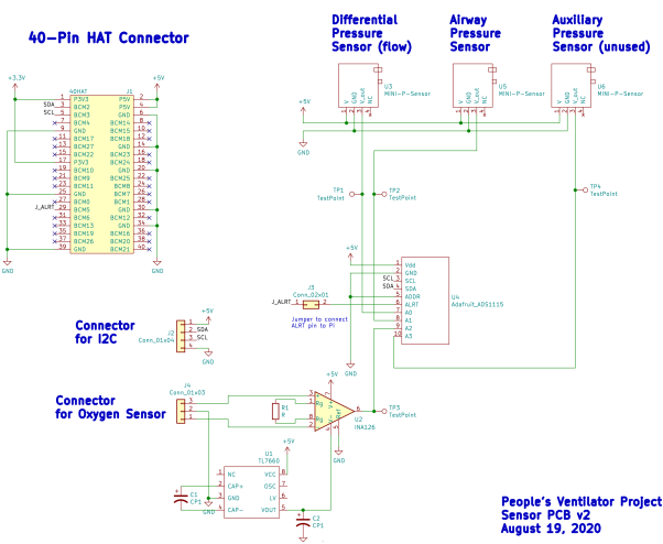
Figure S7. Sensor PCB schematic.
