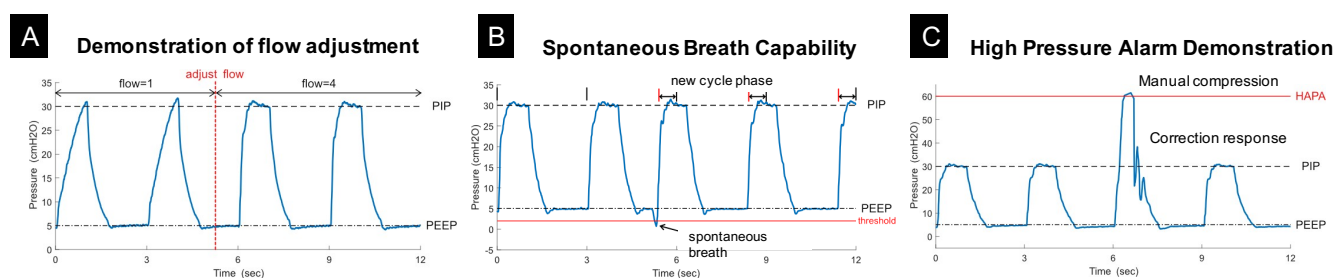
Fig. 3. Demonstration of waveform tuning via flow adjustment. If necessary, the operator can increase the flow setting through the system GUI to decrease the pressure ramp time. Test settings: compliance C=20 mL/cm H 2 O, airway resistance R=20 cm H 2 O/L/s, PIP=30 cm H 2 O, PEEP=5 cm H 2 O.
