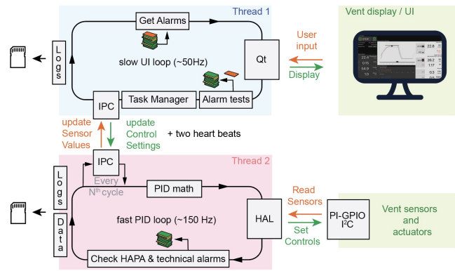
Fig. 8. Overview of the software architecture. The user interface (UI) is controlled by a UI thread, that communicates with a second, faster, thread that implements the PID logic, by xml-rpc. The control loop is connected to hardware via the hardware abstraction layer (HAL). Both threads check for alarms; lower priority in the UI thread, and high priority in the controller thread, like HAPA (high airway pressure alert). The stack of cards illustrates a shared alarm-manager, which intelligently manages alarms, but keeping track of the various types, and sorting by importance. The individual processes add to this stack.
