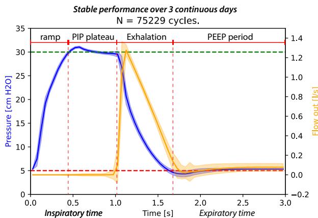
Fig. 2. Overlaid pressure control breath cycle waveforms for airway pressure and flow out over 70,000+ cycles. Test settings: compliance C=20 mL/cm H2O, airway resistance R=20 cm H2O/L/s, PIP=30 cm H2O, PEEP=5 cm H2O.
