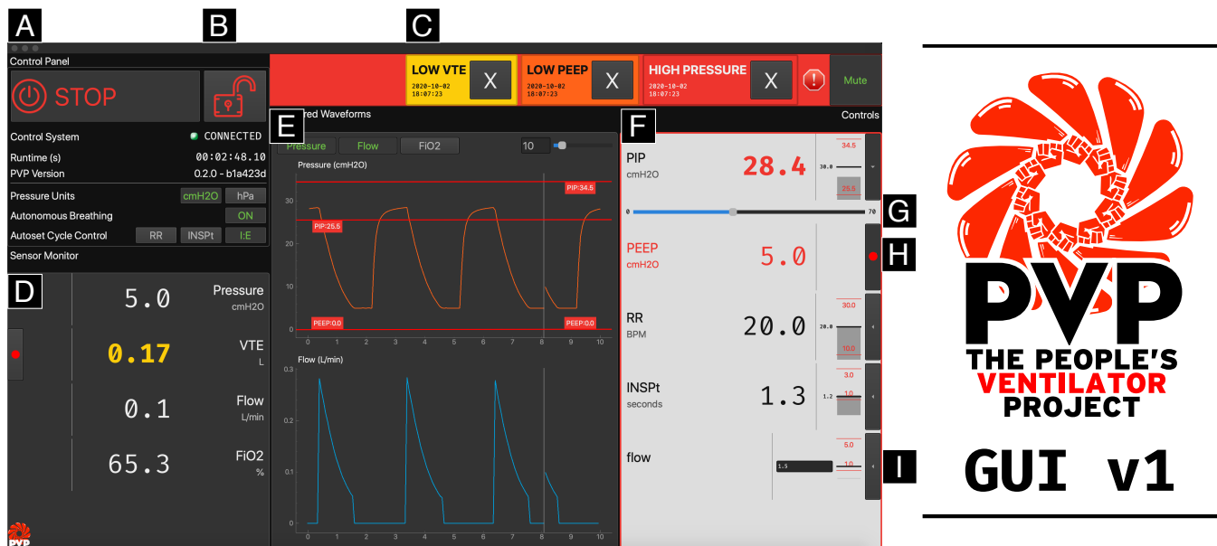
Fig. 9. PVP1 GUI Design: The PVP1 GUI is composed of modular components to provide a uniform interaction syntax but also allow reconfiguration for different ventilation modes and hardware configurations. The GUI is broadly segmented into three columns: system monitoring components on the left (A, D), waveform plots of sensor values in the center (E), and ventilation controls on the right (F). A control panel (A) controls and displays basic system operating status. To prevent accidental changes, controls are locked (B) by default (but are unlocked in this figure). Beneath the control panel, a series of widgets in a "Monitor" column (D) display the values of sensors that are not used to control ventilation. The same widgets are to populate the rightmost "Control" column (F) to set the operating parameters of the ventilator. Ventilator control settings can be input with the touchscreen or mouse (with a slider, G), with the keyboard (in a text-entry box, I), or by recording recent sensor values (with a "record" button, H). By using a unified system of components across the whole interface, we can accommodate diverse hardware configurations (eg. rather than setting a computer-controlled PEEP valve and set alarm thresholds by recording sensed values) and alarm conditions (VTE is a derived sensor value rather than a control value, but needs to have patient-calibrated alarm thresholds) while maintaining a consistent interaction syntax. Alarm thresholds are automatically calculated as some multiple of the set value (eg. a HAPA alarm is 115% of set PIP). Alarm thresholds are represented numerically and graphically in both the relevant control widget and waveform plot (red horizontal lines in E and F). Alarms are displayed as "Alarm Cards" (C) color coded and ordered by alarm severity. Color codes are also reflected in the relevant displayed parameter (eg. yellow displayed VTE value in D to match the low-severity LOW VTE alarm in C), allowing clinicians to quickly identify and attend to the cause of an alarm. Screenshot of actual GUI running PVP's built in stimulation mode.
