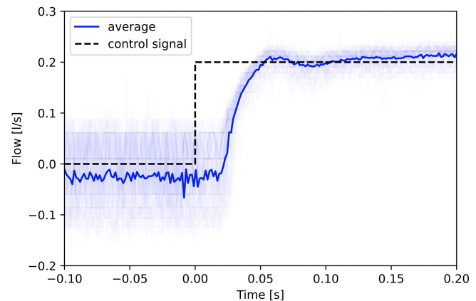
Figure S4. Measurements of the delay caused by the inspiratory valve. At time zero, the control signal to open the valve was sent and we monitored flow through the system. The thin blue lines illustrate 100 consecutive individual trials, the drawn blue line is the average, and the dashed line illustrates the control signal. 50% of the maximum flow was reached after 32 ms, 90% were reached after 53 ms.
