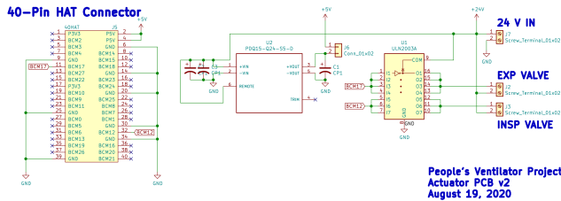
Figure S6. Actuator PCB schematic.
