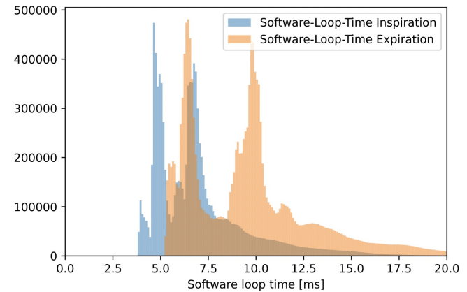
Figure S3. Histograms of the software-loop-time. Measurements of the software loop-time during inspiration (blue) and expiration (orange) over ca. 62h of breathing. Median inspiration loop time is 6.6 ms, median expiration loop time is 9.5 ms. Notice multiple peaks, depending on the addition of sensor readings, every one of which contributes \approx 2.5 ms. The mechanical valves are a factor of \approx 5 slower than the software
