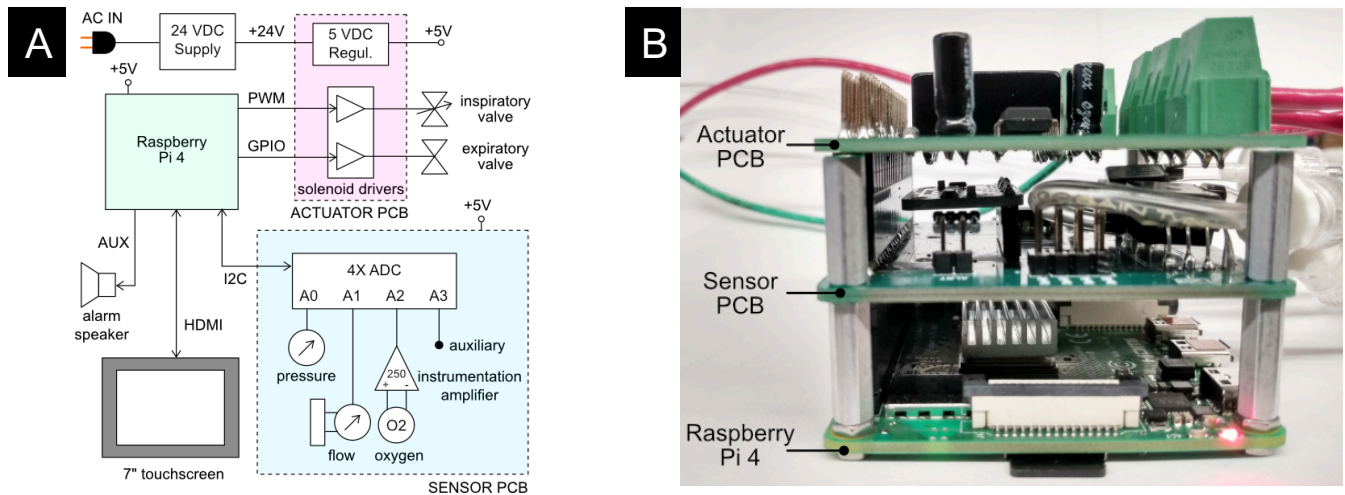
Fig. 7. Overview of PVP1 electronics. A) Block diagram. System power is supplied by AC through an uninterruptible power supply (UPS) regulated to 24 VDC by a switched-mode power supply, to be used to drive the valves. This DC is further regulated to 5 VDC to supply power to the Raspberry Pi and associated sensors. The sensor PCB coordinates the inputs of the pressure and oxygen sensors. The actuator PCB amplifies control signals from the Pi to drive the valve solenoids. I/O is provided by a 7" touchscreen and an alarm speaker. B) Photograph of the modular system electronics. Two modular PCB 'hats' stack onto the Raspberry Pi via 40-pin stackable headers: the sensor PCB and the actuator PCB.
