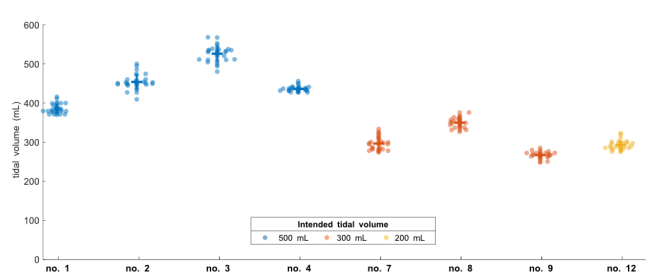
Fig. 6. Tidal volume performance for the ISO 80601-2-80-2018 pressure controlled ventilator standard tests, averaged across 30 breath cycles for each condition.
