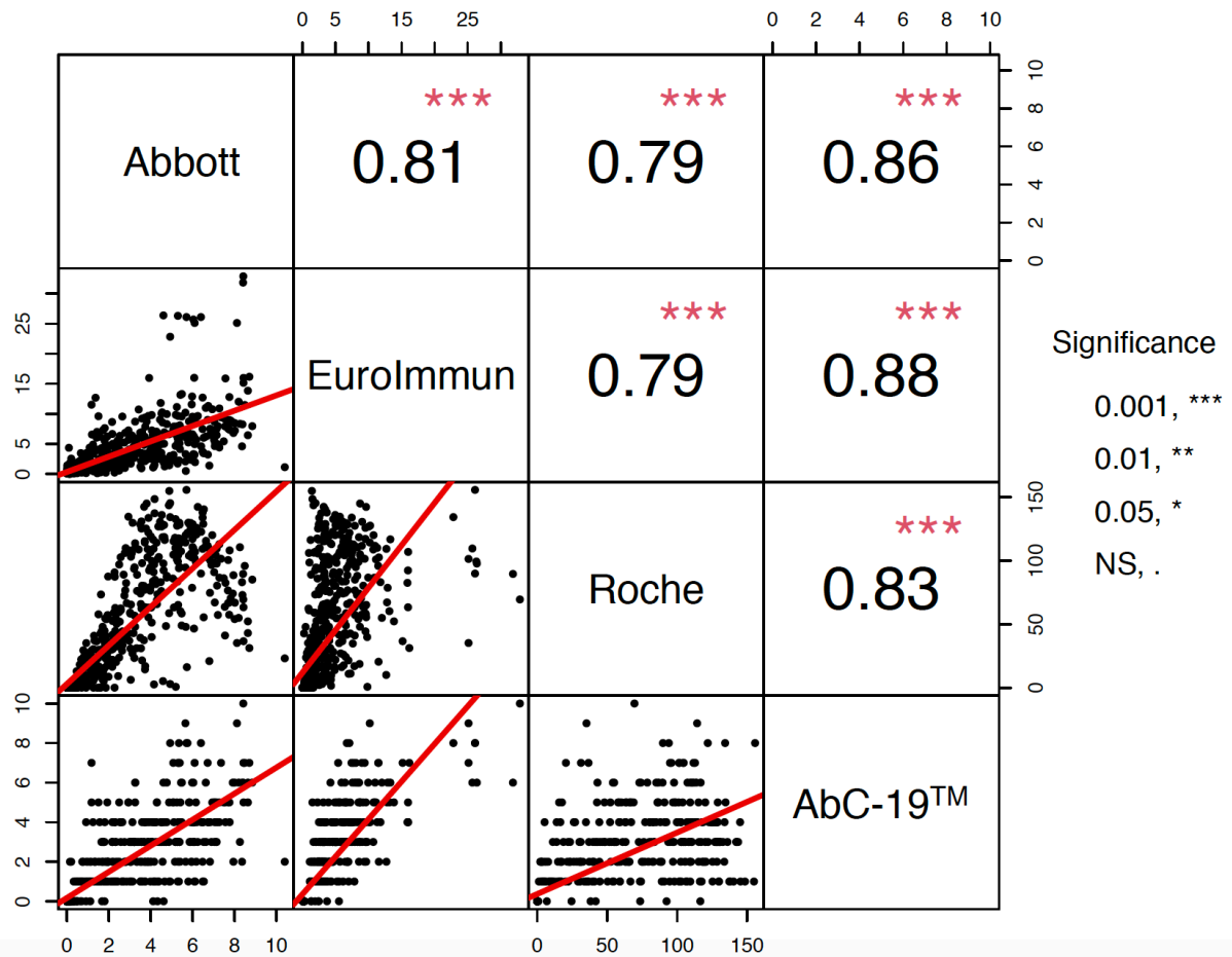
Figure S5: Correlation matrix between Abbott, EuroImmun, Roche and AbC-19 quantitative output values for SARS-CoV-2 antibody levels. Strong correlations are observed between all immunoassays. The level of significance was set at p < 0.05 . All immunoassays were significantly correlated p < 0.001 .
