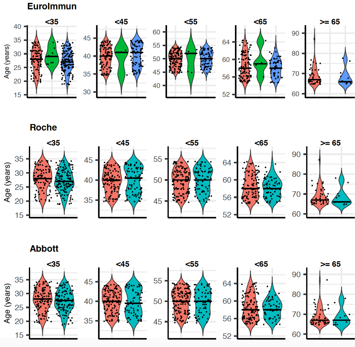
Figure S4: Age violin plots separated into age groups (where age data available) for samples included in correlation analysis.
