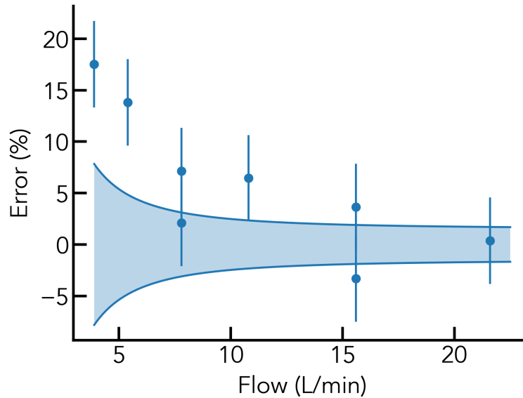
Figure 7: Error vs. Measured flow taking the mean of inhaled and exhaled breaths (10 trials each, 20 total measurements per condition)
