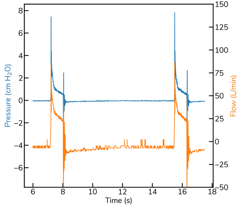
Figure 5: Pressure and derived flow over two sample breaths given by a Bird Mark 7 to a simple test lung, as recorded by the Honeywell differential pressure sensor.
