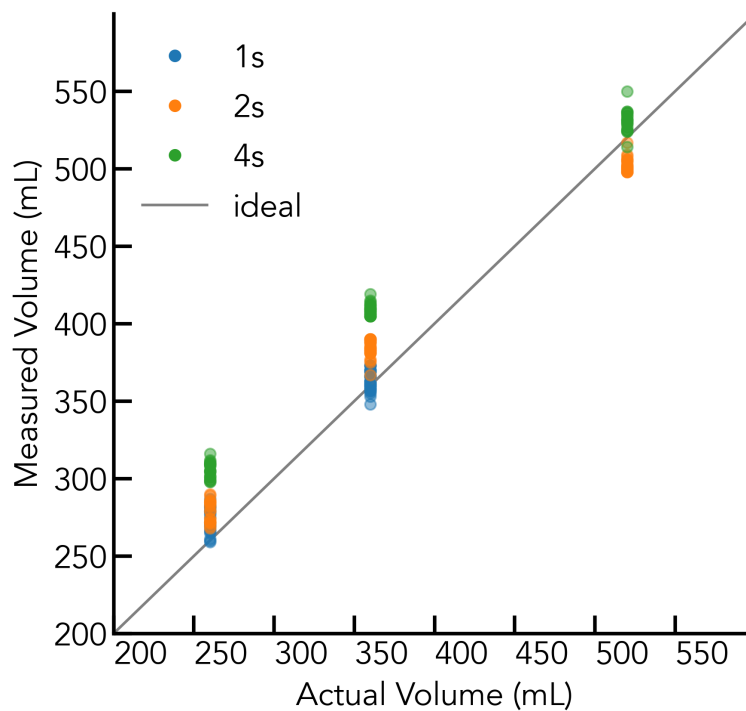
Figure 6: Measured volume from syringe experiments using 1s, 2s, and 4s flow durations. Error increases at lower flows, with a maximum error of MAX at the lowest volume/flow rate (3.75L/min), much lower than typical flow for an adult ventilator. Syringe plunges were performed visually, and the error increases with decreasing flow. Expected maximum error from device alone is 6% at the lowest flow, and the mean of the lowest-flow measurements are 10% away from the mean of the highest-flow measurements in the same condition.
