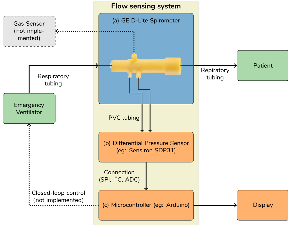
Figure 1: Overview of flow sensing system and integration in a clinical setting. The D-Lite spirometer fits into sections of standard 22 mm ventilator tubing (with an adapter at the smaller end). The dynamic pressure drop is sensed across the two oppositely-directed terminals by a pressure sensor (e.g. the Sensiron SDP31), and this information is sent to a central processing unit (e.g. an Arduino). This information can then be displayed or used in closed-loop feedback.
