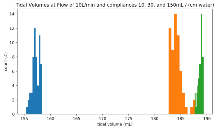
Figure S2: Histogram of measured tidal volumes of Stanford rapid-response ventilator at compliances of 10, 30, and 150 mL/cmH 2 O at the lowest flow characterized (10 L/min). The intra-compliance variability was <2% min/max with standard deviation <0.5%
