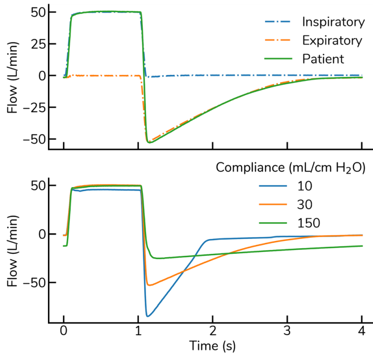
Figure 4: Flow vs. time over a single 4-second breath cycle for the Stanford Rapid Response ventilator. Data was obtained from 138 breaths and averaged into a single plot (top). Test lung compliance was varied at a fixed flow, and the resultant flow profiles are plotted versus time (bottom).
