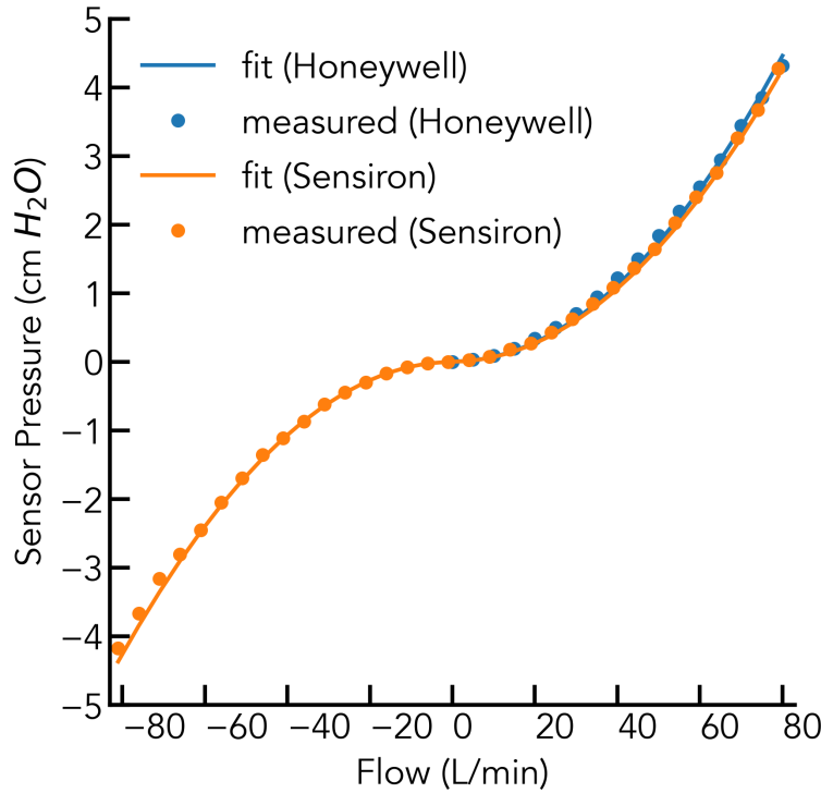
Figure 3: Pressure vs. flow for the D-Lite spirometer as measured by Alicat mass flow meter. Honeywell data is corrected for zero offset prior to fitting to quadratic. Uncertainty in flow is <3 L/min at all flows, and uncertainty in pressure is <0.01 cmH 2
