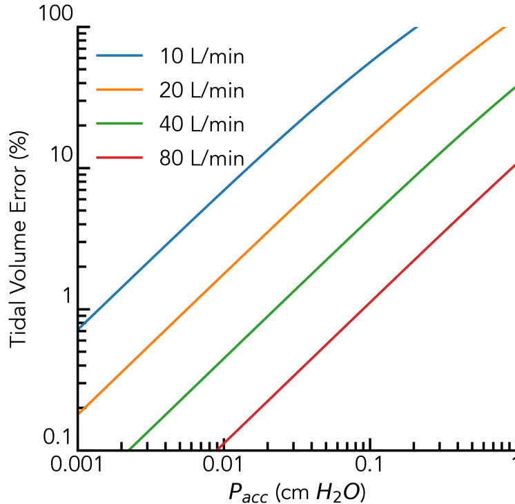
Figure 2: Tidal volume error vs. pressure sensor absolute accuracy at varying flows. Each curve corresponds to a different instantaneous flow (in which case the results are exact), or average flow over a sensing period, in which case they are approximate. The Sensiron SDP31 has an absolute accuracy of 0.001 cmH 2 O, while the Honeywell SSCMRRN060MDSA5 has an accuracy of 0.01 cmH 2 O. Note that the error increases with worsening accuracy and lower flow
