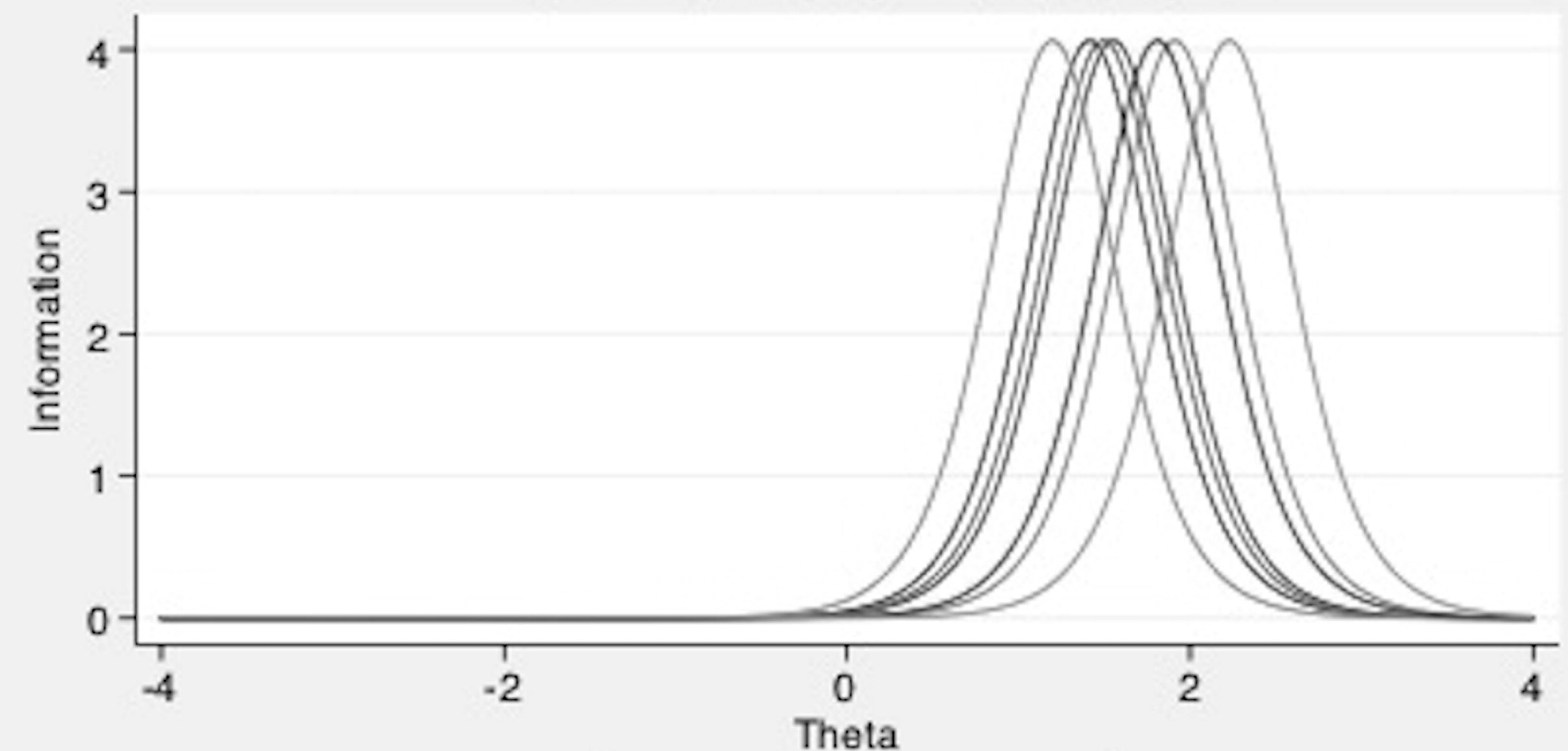
Item Information Functions
