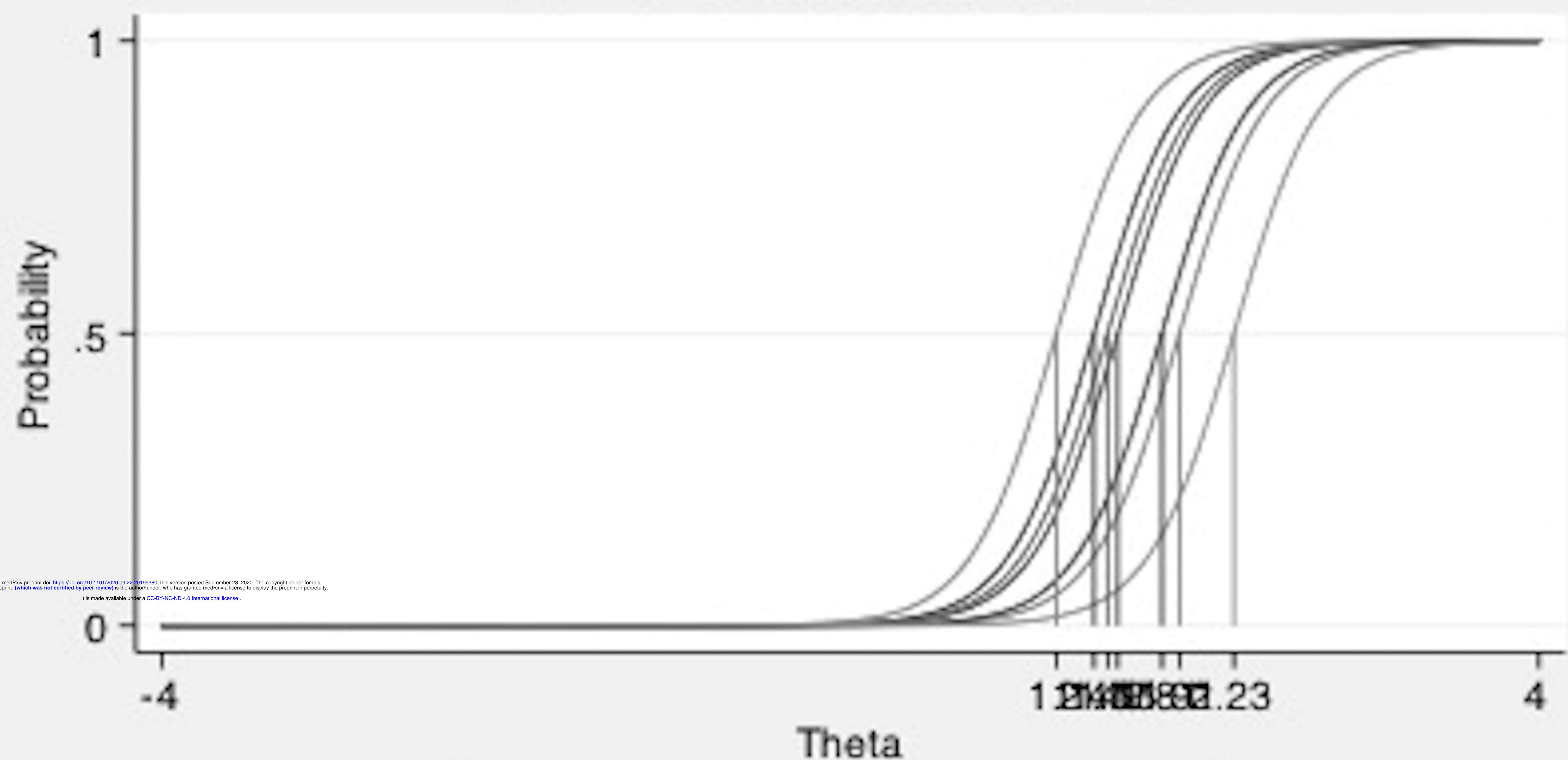
Item Characteristic Curves
