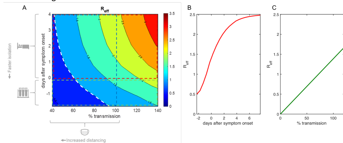
Figure 8: Rapid testing and transmission reduction are both needed to bring outbreaks under control. A. Effective reproductive number ( R_{eff} ) as a function of timeliness of isolation and percent transmission. B. Effective reproductive number ( R_{eff} ) versus timeliness of isolation for 100% of baseline transmission indicates nonlinear effect on increased ( R_{eff} ). C. Effective reproductive number ( R_{eff} ) versus percent transmission indicates that R_{eff} scales linearly with the amount of transmission reduction.
