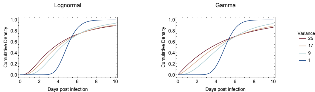
Figure 2: A schematic showing the impact of functional form and variance on the timing of onward transmission. The plots show cumulative generation time distributions, i.e. the proportion of transmission occurring within x days of infection. All distributions have a mean of 5 days.
