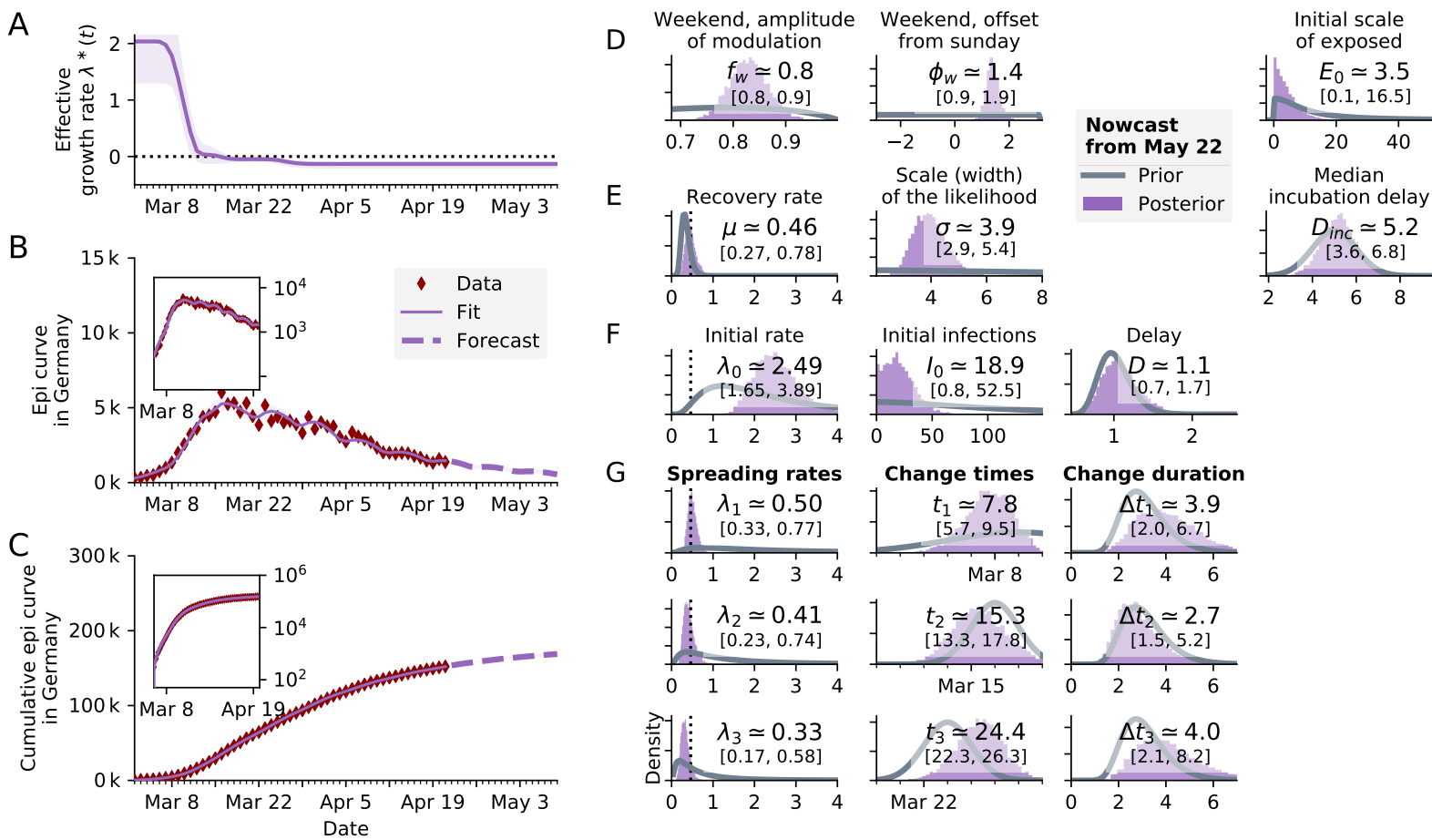
FIG. 19. SEIR-like model using the onset of symptoms (unsmoothed Nowcast from May 22 [16]) of the RKI data for inference. The median of the lognormal prior of the delay between infectious and onset of symptoms has been set to 1 day (right-most panel F). A : Time-dependent model estimate of the effective spreading rate \lambda^*(t) . Note : Due to different model dynamics, \lambda^*(t) can only be compared qualitatively between SEIR and SIR models. The numeric values of the rates ( \mu , \lambda etc.) differ between models because they reflect the duration a person remains in a given compartment. Note : We currently do not (yet) incorporate the uncertainties that are introduced by nowcasting, compared to using the reported cases. This leads to over-confident parameter estimates, including the effective spreading rate \lambda^*(t) ; the shown uncertainties are underestimated. B : Comparison of daily new reported cases and the model (purple solid line for median fit with 95% credible intervals, dashed line for median forecast with 95% CI); inset same data in log-lin scale. C : Comparison of total reported cases and the model (same representation as in B). D–G : Priors (gray lines) and posteriors (purple histograms) of all model parameters; inset values indicate the median and 95% credible intervals of the posteriors.
