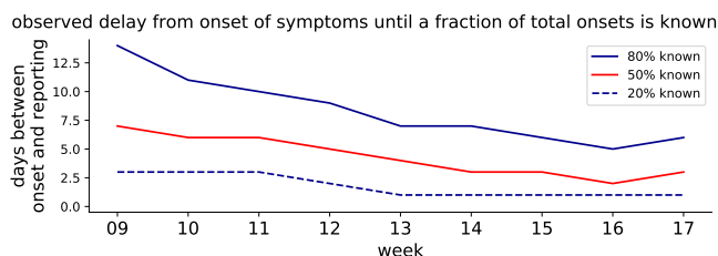
FIG. 13. The reporting delay decreases from week 9 to week 14. Grouped by week, the delay between onset of symptoms and the reporting of 20%, 50%, 80% fractions of all known onsets is shown (cf. dots in Fig. 12).
