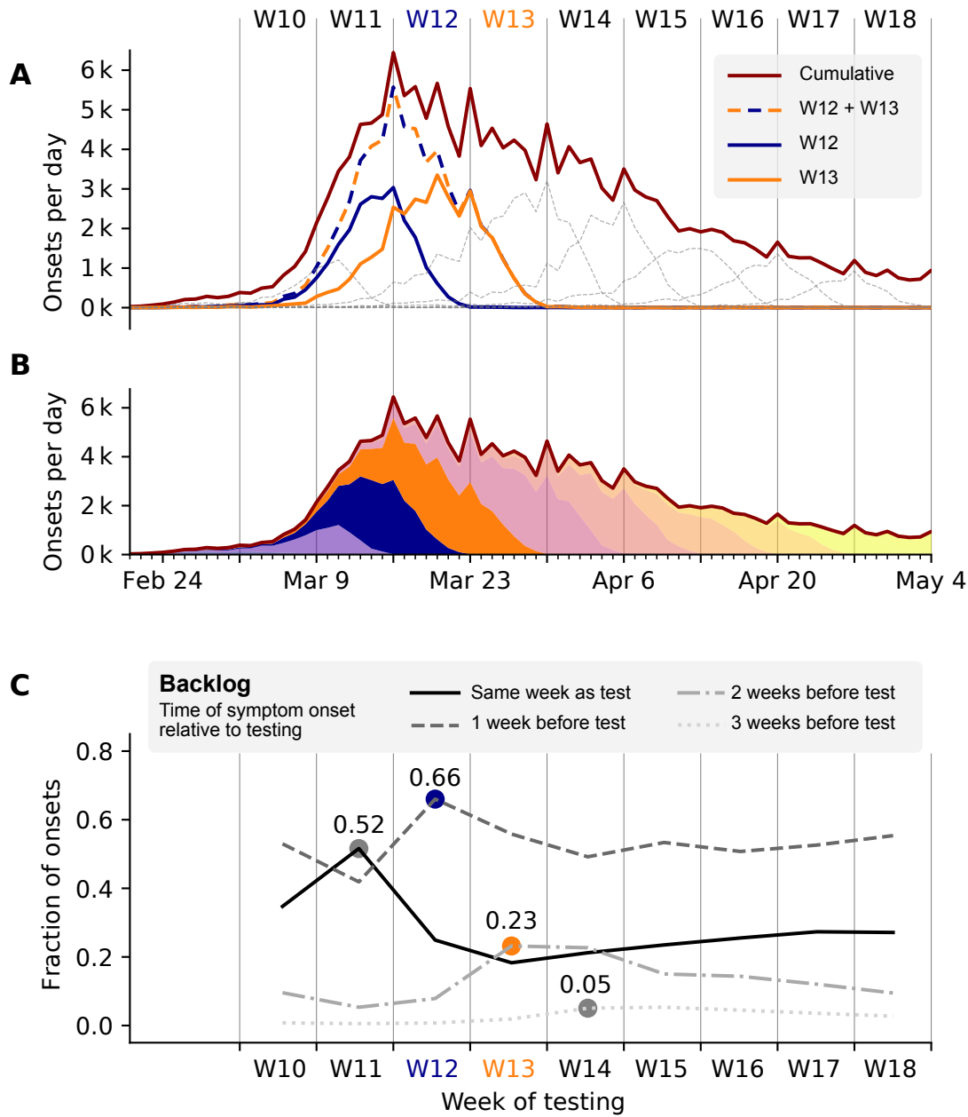
FIG. 14. Testing in one week confirms onsets of symptoms that occur up to 4 weeks earlier. The extend of this effect is analyzed based on the RKI database through decomposition by allocation of onsets of symptoms to weeks of testing. It is assumed that the delay between the time of testing and Meldedatum is 1 day. Tue-Mon Meldedatum is taken as a proxy for Mon-Sun testing. A Onsets of symptoms per day curves allocated to weeks of testing, weeks 12 and 13 are highlighted. Most known onsets around the peak of the epi curve in week 11 are confirmed by the testing in weeks 12 and 13. B stacked decomposition of the epi curve into weeks of testing. C To reveal crucial information about week-to-week change in the number of total onsets based on one week of testing, the shape of the distributions of onsets of symptoms confirmed by that week of testing is characterized. The fraction of onsets in the same week and each preceding week out of the total onsets confirmed by the week of testing is calculated. This indicates, the portion of a week's positive tests confirming onsets in the same week or in preceding weeks (max. 3 weeks earlier). The evolution of these 4 values is plotted by the week of testing. The peak of the epi curve can be tracked through testing results of weeks 11 to 14 as a maximum in the same-week/n-weeks earlier fraction of onsets confirmed in those respective weeks: 52% of all cases confirmed through testing in week 11 had onset of symptoms in the same week. Even more notable: 66% of positive tests in week 12 are linked to onsets 1 week earlier: in week 11. For comparison, see Fig. ??
