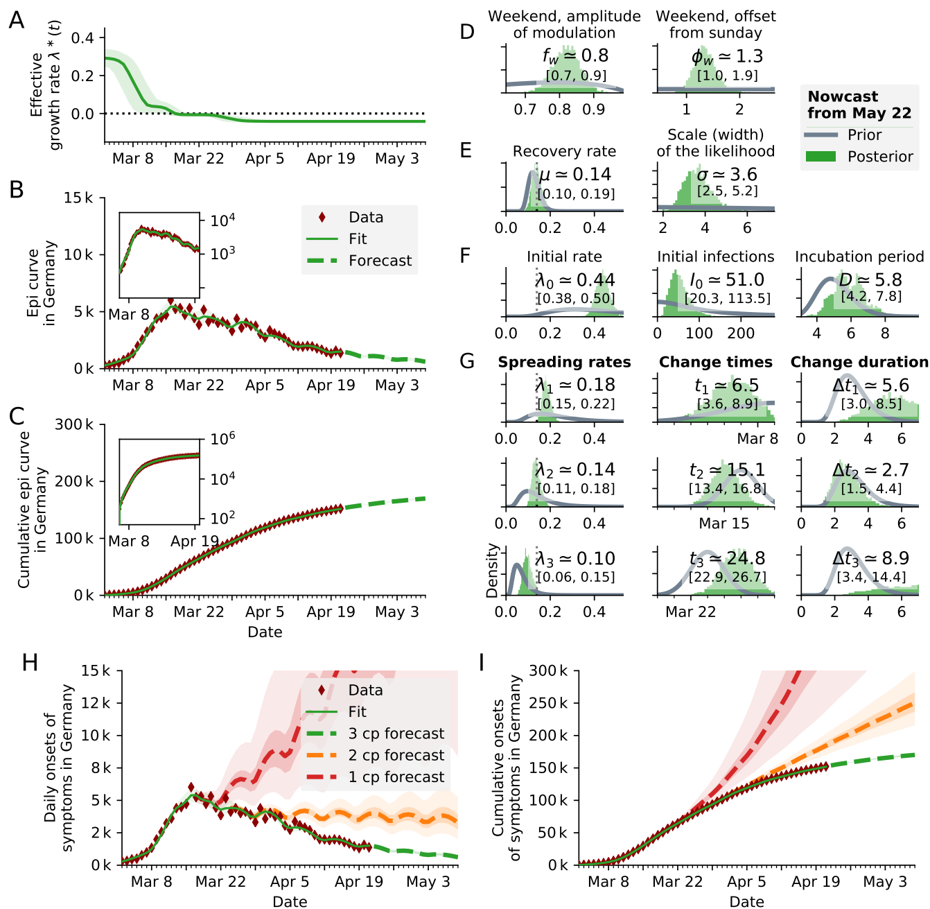
FIG. 17. SIR model using the onset of symptoms (unsmoothed Nowcast from May 22 [16]) of the RKI data for inference. The median of the lognormal prior of the delay between infection and onset of symptoms has been set to 5 days (right-most panel F). A: Time-dependent model estimate of the effective spreading rate \lambda^*(t) . Note: We currently do not (yet) incorporate the uncertainties that are introduced by nowcasting, compared to using the reported cases. This leads to over-confident parameter estimates, including the effective spreading rate \lambda^*(t) ; the shown uncertainties are underestimated. B: Comparison of daily new reported cases and the model (green solid line for median fit with 95% credible intervals, dashed line for median forecast with 95% CI); inset: same data in log-lin scale. Note: We currently do not (yet) incorporate the uncertainties that are introduced by nowcasting, compared to using the reported cases. This leads to over-confident parameter estimates, including the effective spreading rate \lambda^*(t) ; the shown uncertainties are underestimated. C: Comparison of total reported cases and the model (same representation as in B). D–G: Priors (gray lines) and posteriors (green histograms) of all model parameters; inset values indicate the median and 95% credible intervals of the posteriors. H–I The fitted model with two alternative forecasts. We consider in addition one scenario where only one intervention happened (red) and one where two interventions happened (orange). Includes 50% and 95% CI.
