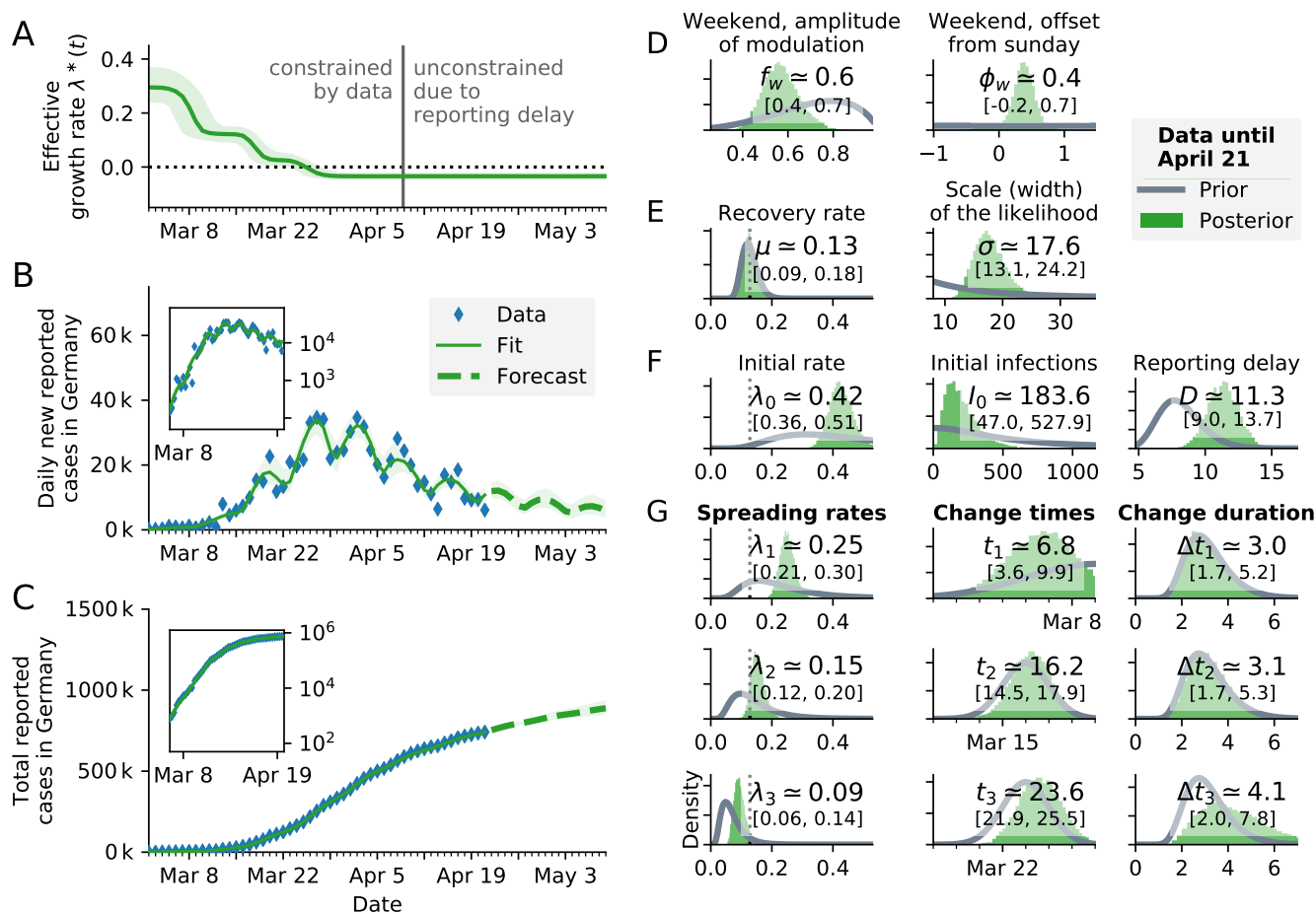
FIG. 20. SIR model with reported case number multiplied by 5, to account for an eventual factor five of unknown cases . Results are nearly identical to original non-multiplied plot (Fig 3. in [1]), showing that a constant underreporting has a negligible effect. The median inferred spreading rates \lambda are about 0.01 larger. A : Time-dependent model estimate of the effective spreading rate \lambda^*(t) . B : Comparison of daily new reported cases and the model (green solid line for median fit with 95% credible intervals, dashed line for median forecast with 95% CI); inset same data in log-lin scale. C : Comparison of total reported cases and the model (same representation as in B). D–G : Priors (gray lines) and posteriors (green histograms) of all model parameters; inset values indicate the median and 95% credible intervals of the posteriors.
