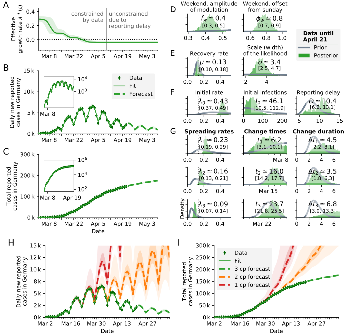
FIG. 15. SIR model (see Fig. 3 of [1]) using the reporting date (Meldedatum) of the RKI data for inference. A: Time-dependent model estimate of the effective spreading rate \lambda^*(t) . B: Comparison of daily new reported cases and the model (green solid line for median fit with 95% credible intervals, dashed line for median forecast with 95% CI); inset same data in log-linear scale. C: Comparison of total reported cases and the model (same representation as in B). D–G: Priors (gray lines) and posteriors (green histograms) of all model parameters; inset values indicate the median and 95% credible intervals of the posteriors. H–I: The fitted model with two alternative forecasts. We consider in addition one scenario where only one intervention happened (red) and one where two interventions happened (orange). Includes 50% and 95% CI.
