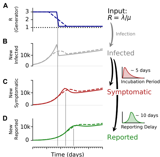
FIG. 2. A change-point in R can lead to a transient decrease in case numbers. To illustrate the effect of a change point, and the delays in observing symptomatic and reported cases, we consider an SIR model with a fast or slow decrease of R , and generate synthetic case numbers. A: The reproductive number R exhibits a change point from R = 3 to R = 1.15 , with a duration of either 1 day (solid) or 9 days (dashed). B: The number of new infections can show a transient decrease caused by the change point in R , even though the underlying dynamics are always in the exponentially growing regime of R > 1 . Such a decrease can be misinterpreted as R < 1 . The number of C new symptomatic cases, and D reported cases is generated by convolving the new infected with a log-normal incubation period (median 5 days) or reporting delay (median 10 days), respectively. Note that the convolution shifts and smooths the curve of the new infected. Nonetheless, the counter-intuitive effects of a transient decrease in case numbers caused by a change point, is still very well visible (See Fig. 4 for the challenges in estimating R around the change point.)
