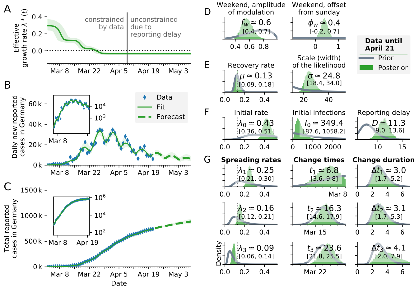
FIG. 21. SIR model with reported case number multiplied by 10, to account for an eventual factor 10 of unknown cases. Results are nearly identical to original non-multiplied plot (Fig 3. in [1]), showing that a constant under-reporting has a negligible effect, similar to Fig. 20. The median inferred spreading rates \lambda are 0.01-0.02 larger. A : Time-dependent model estimate of the effective spreading rate \lambda^*(t) . B : Comparison of daily new reported cases and the model (green solid line for median fit with 95% credible intervals, dashed line for median forecast with 95% CI); inset same data in log-lin scale. C : Comparison of total reported cases and the model (same representation as in B). D–G : Priors (gray lines) and posteriors (green histograms) of all model parameters; inset values indicate the median and 95% credible intervals of the posteriors.
