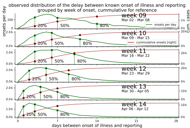
FIG. 12. The onsets of symptoms are confirmed by testing at a later and varying point in time, which accounts for most of the delay until all or the main fraction of known onset of symptoms ( IstErkrankungsbeginn in RKI-database) are reported. From the RKI data, the number of cases per delay between onset of illness and reporting (i.e. RefDatum and Meldedatum ) for cases with known onset of symptoms ( IstErkrankungsbeginn ) are counted for each week. The fraction of reported cases out of the total onsets up to a delay are highlighted for 20%, 50% and 80%. The cumulative number of cases reported up to each delay is displayed for reference.
