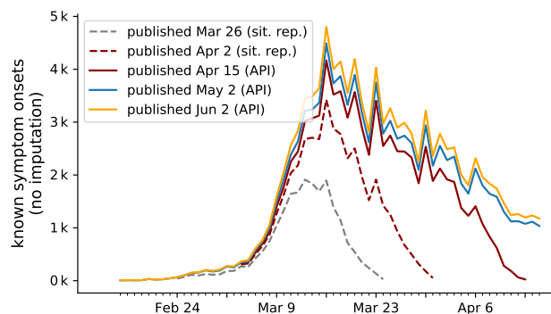
FIG. 10. The curve of known symptom onset continuously changes over time, as the date of onset of further reported cases is obtained. Because testing confirms the onset of symptoms in the past with varying delay, the curve not only grows at its tail but over a wide time period with each new publication. Known onsets are reproduced from the RKI’s daily situation reports (Mar 26 and Apr 2, read of from respective plots) and the publicly available RKI-database (Apr 15, May 2 and Jun 2). Unknown onsets of symptoms, which account for 40% of total number of cases, are not considered here. Hence the curve on display here is not the full epi curve.
