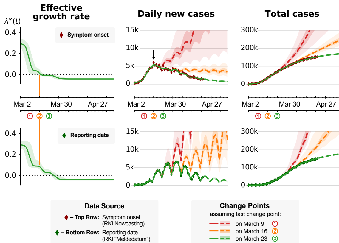
FIG. 8. Model-based inference is consistent when based on symptom onset (top) or reporting date (bottom). We repeated our SIR-model based inference (Fig. 3 in [1]) that used JHU data [15], now using the date of symptom onset (red diamonds, top) [16] and the reporting date (green diamonds, bottom) of daily new cases as reported by the RKI [17]. Note: We currently do not incorporate the uncertainties that are introduced by nowcasting (red diamonds, top), compared to using the reported cases. This leads to over-confident parameter estimates, including the effective spreading rate \lambda^*(t) ; the shown uncertainties are underestimated. Left: Effective growth rate \lambda^*(t) inferred by the model. Dates of the three main public interventions are indicated by colored circles and vertical lines. The values of \lambda^*(t) before and after all change points is consistent across both data sources. Note that, when the symptom onset is used, \lambda^*(t) drops to zero already after the second change point. Still, only after the third change point \lambda^*(t) becomes sufficiently negative to cause decreasing daily new case numbers. Center: Daily new case numbers. Dashed lines show inferred case numbers assuming that the last two (red) or the last one (orange) change points were excluded. The weekday-dependence in daily new reported cases is already accounted for when using symptom onsets (top). Center, Top: Although \lambda^*(t) already dropped to (slightly-below) zero as of the second change point, daily new cases do not decrease if the third change point is excluded (orange). Note the arrow: Due to the transient decrease in new cases after change points (cf. Fig. 4) as well as the delay between symptom onset and reporting (cf. Fig. 4), the peak that corresponds to maximum daily new infections is located already around March 16 (for symptom onsets); yet note again that this does not mean that new cases would have declined rapidly already after the second change point (see the orange curve). Right: Total, cumulative case numbers.
