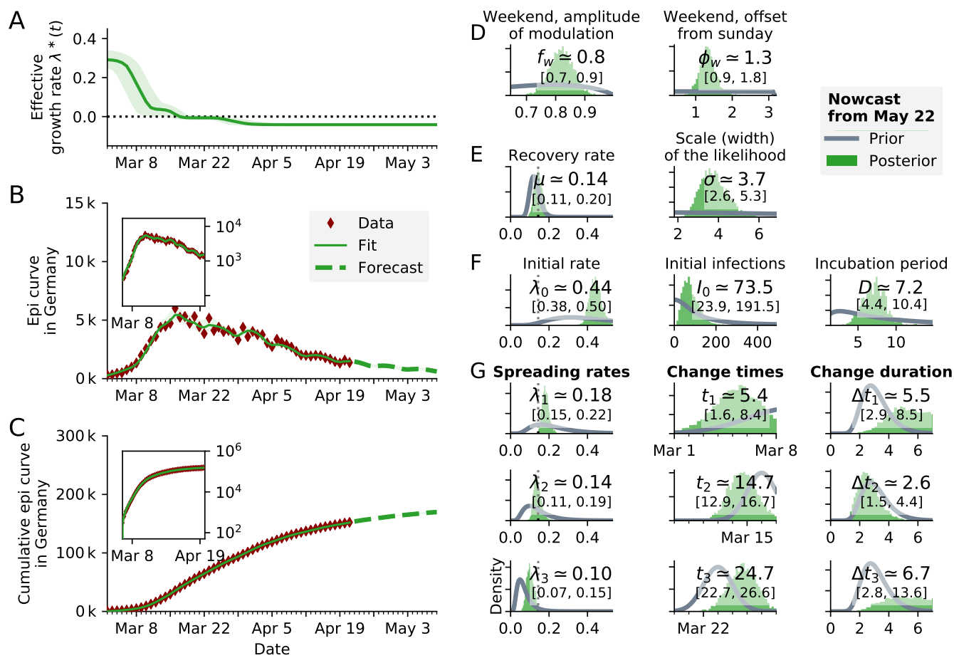
FIG. 18. SIR model using the onset of symptoms (unsmoothed Nowcast from May 22 [16]) of the RKI data for inference. The median of the lognormal prior of the delay between infection and onset of symptoms has been set to a relatively uninformative prior (right-most panel F). The posterior of the delay has as median 7.2 days, which is close to the expected incubation period of 5 days. A : Time-dependent model estimate of the effective spreading rate \lambda^*(t) . Note : We currently do not (yet) incorporate the uncertainties that are introduced by nowcasting, compared to using the reported cases. This leads to over-confident parameter estimates, including the effective spreading rate \lambda^*(t) ; the shown uncertainties are underestimated. B : Comparison of daily new reported cases and the model (green solid line for median fit with 95% credible intervals, dashed line for median forecast with 95% CI); inset same data in log-lin scale. C : Comparison of total reported cases and the model (same representation as in B). D–G : Priors (gray lines) and posteriors (green histograms) of all model parameters; inset values indicate the median and 95% credible intervals of the posteriors.
