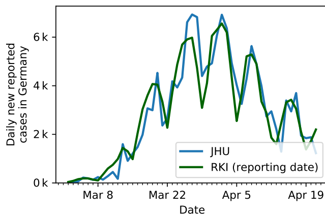
FIG. 9. Comparison of the German case numbers as published by the Johns Hopkins University (JHU) used in our previous publication [1], to the case number of the Robert Koch Institute (RKI).
