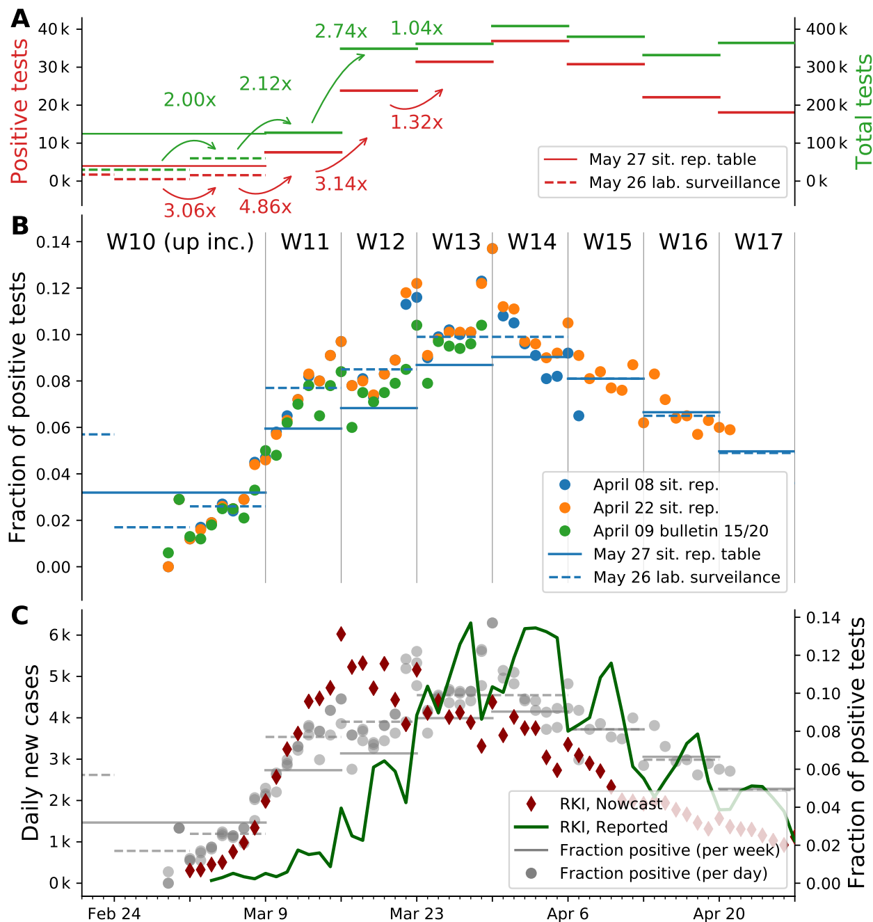
FIG. 11. Weeks 10 to 12 show strong growth in in the number of new cases, which was not limited by the early testing capacity. A: Comparison of number of positive test results with the number of tests performed for each week. Reproduced from Table 5 in [21] and extrapolated from [22]. Note: Numbers for week 10 and earlier are represented by a single data point in the first source and individually in the latter. The week-over-week increase uses available weekly data. B: Mid-term changes in the fraction of positive tests is more obvious in the daily data (points) than in the weekly (bars), especially in early March. Daily values are taken from situation reports [21, 23, 24] (full dataset) and the epi bulletin [22, 25] (ARS dataset). Weekly values, represented as horizontal lines, are taken from a situation report table and a weekly lab surveillance report (ARS dataset). Note: the latter represents a subset of all tests. Compared to the situation report, the ARS dataset lists weeks 8 to 10 individually. C: Overlay of Panel B with the number of cases reported per day by the RKI and the estimated epi curve (imputation and Nowcasting, as described in [19]). The fraction of positive tests correlates with the number of reported cases from week 13 onward, as the total number of tests reaches a constant level.
