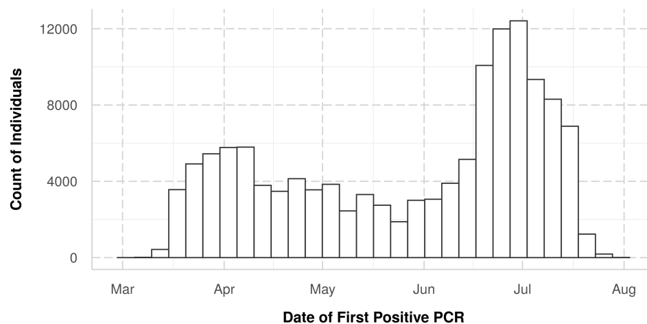
Figure 2. Counts of individuals with positive RT-PCR tests by date.
