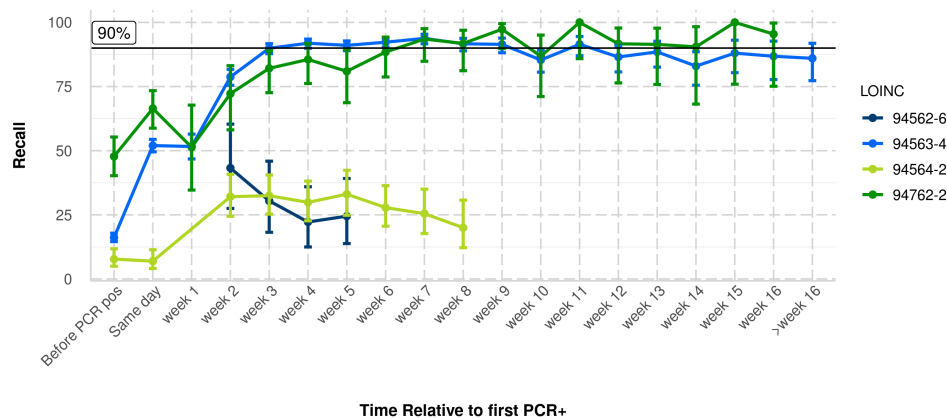
Figure 4. Estimated recall of serological tests by length of time from first positive RT-PCR test. Only groupings with > 10 positive results reported are shown.
