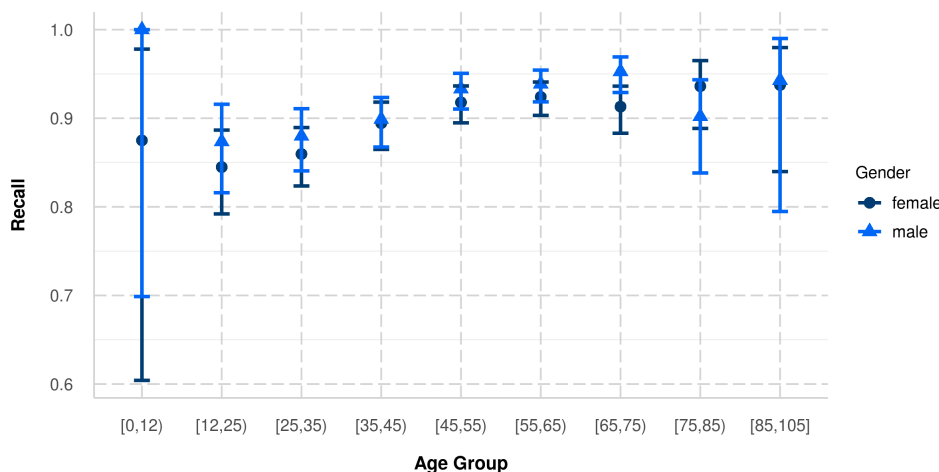
Figure 5. Estimated recall of serological tests by age and sex.
