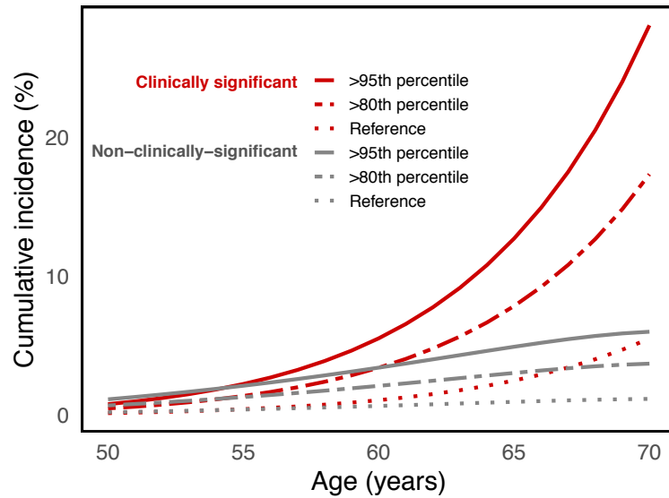
Figure 1. Cumulative incidence curves for PHS166. Risk-adjusted cumulative incidence curves for the upper 5 th percentile (>95 th percentile) and upper 20 th percentile (>80 th percentile) of PHS166 scores for clinically significant and non-clinically-significant prostate cancer.
