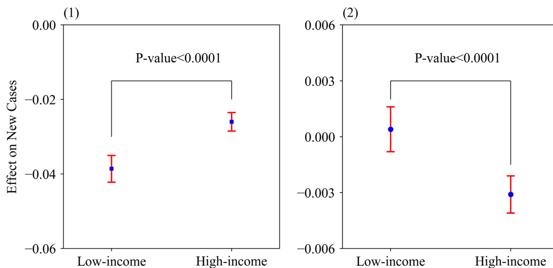
Figure 5. Temperature and Relative Humidity Effect on COVID-19 Transmission in High and Low-Income Regions.
