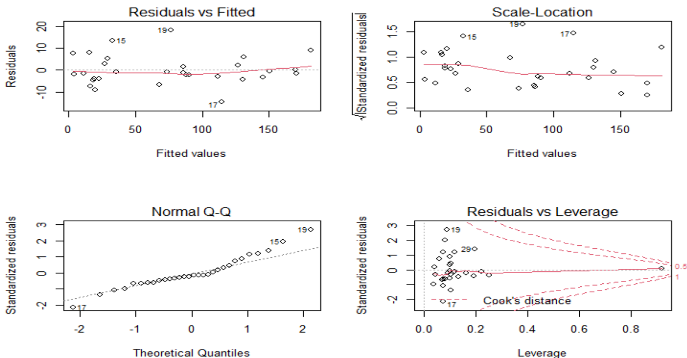
Figure 9: R-Output of Multiple Linear Regression Assumptions
