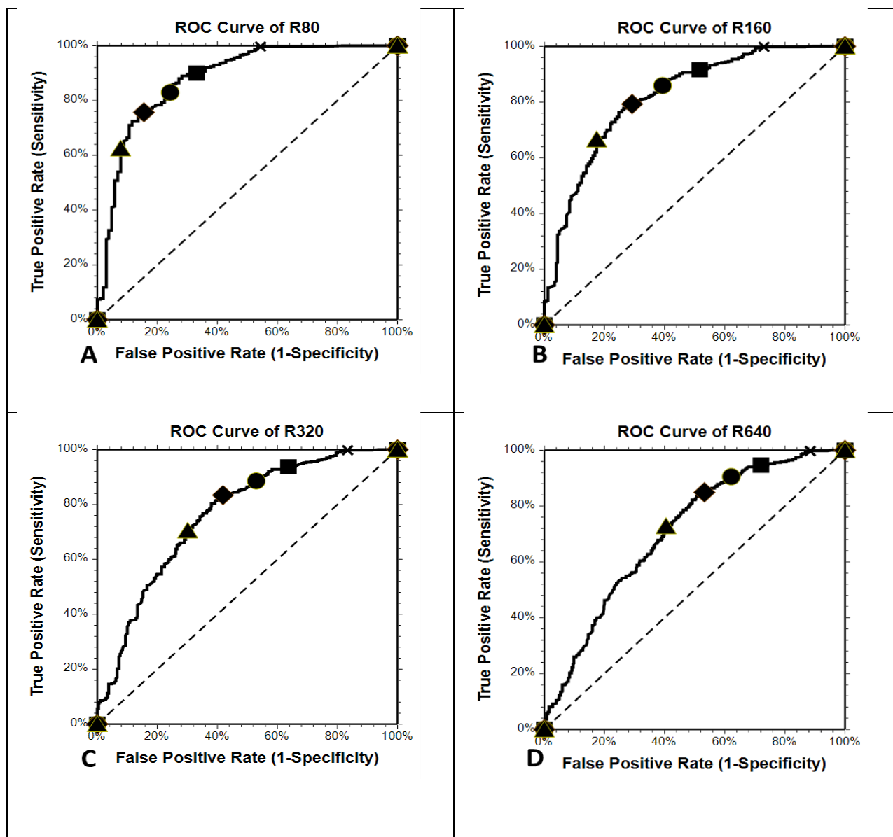
Figure 3. ROC Curves for Varied nAb Titer Thresholds. As the nAb titer increases the ability of the S/Co to predict the nAb titer decreases. ▲:S/CO=60 ◆:S/CO=30 ●:S/CO=20 ■:S/CO=10 X:S/CO=1.
