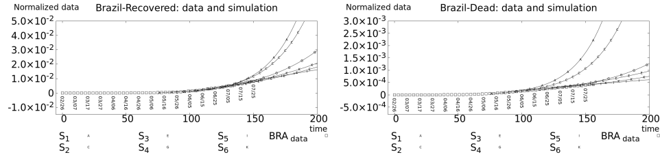
Figure 12: Brazil-Recovered(left)/Dead(right) reconstructed data from WHO Coronavirus Disease (COVID-19) Dashboard [4] and our simulations S_1, \dots, S_6 .
