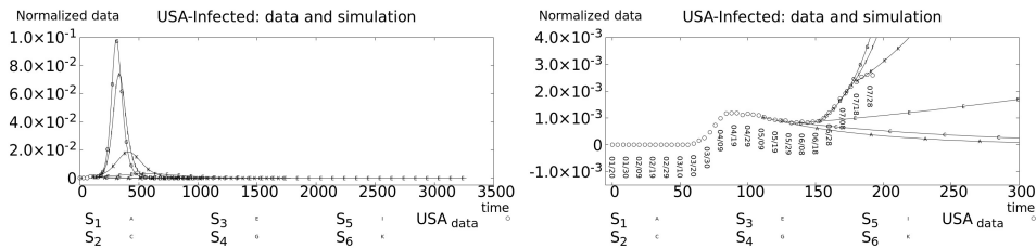
Figure 6: USA-Infected reconstructed data from WHO Coronavirus Disease (COVID-19) Dashboard [4] and simulations S_1, \dots, S_6 .
