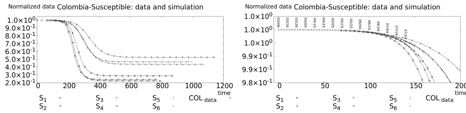
Figure 9: Colombia-Susceptible reconstructed data from WHO Coronavirus Disease (COVID-19) Dashboard [4] and simulations S_1, \dots, S_6 .
