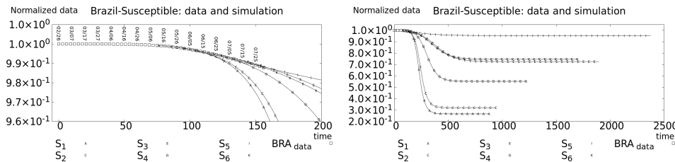
Figure 8: Brazil-Susceptible reconstructed data from WHO Coronavirus Disease (COVID-19) Dashboard [4] and simulations S_1, \dots, S_6 .
