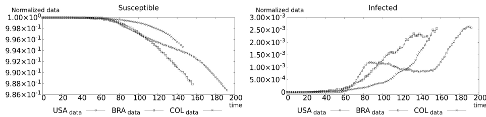
Figure 3: Susceptible (left), and infected (right) normalized data
