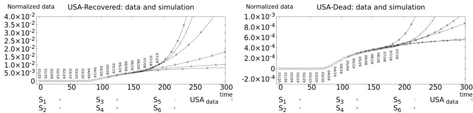
Figure 7: USA-Recovered(left)/Dead(right) reconstructed data from WHO Coronavirus Disease (COVID-19) Dashboard [4] and our simulations S_1, \dots, S_6 .
