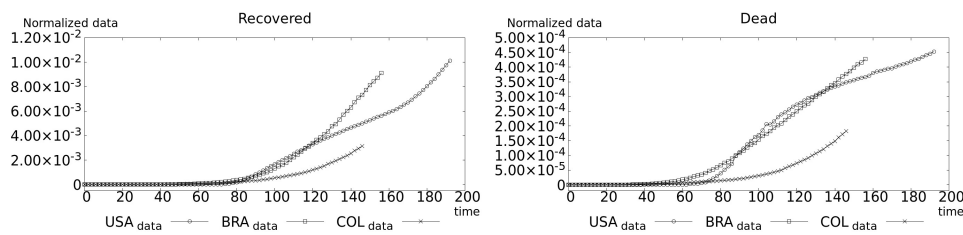
Figure 4: Recovered (left), and dead (right) normalized data
