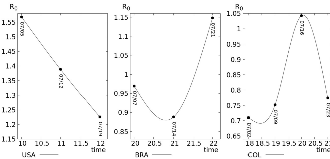
Figure 14: Basic reproduction number R_0 at the time.
