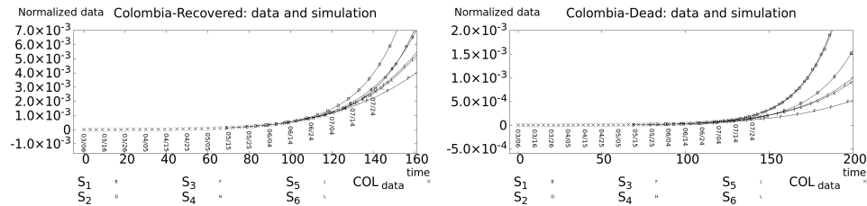
Figure 13: Colombia-Recovered(left)/Dead(right) reconstructed data from WHO Coronavirus Disease (COVID-19) Dashboard [4] and our simulations S_1, \dots, S_6 .
