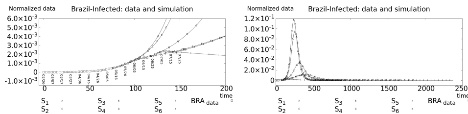
Figure 11: Brazil-Infected reconstructed data from WHO Coronavirus Disease (COVID-19) Dashboard [4] and simulations S_1, \dots, S_6 .
