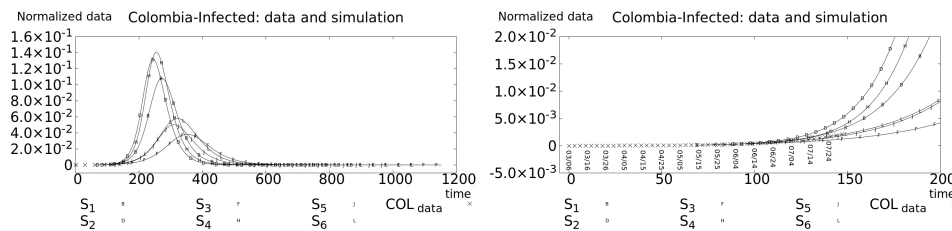
Figure 10: Colombia-Infected reconstructed data from WHO Coronavirus Disease (COVID-19) Dashboard [4] and simulations S_1, \dots, S_6 .
