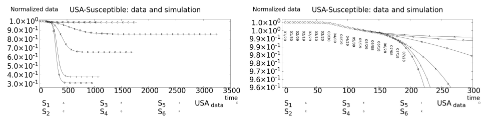
Figure 5: USA-Susceptible reconstructed data from WHO Coronavirus Disease (COVID-19) Dashboard [4] and simulations S_1, \dots, S_6 .
