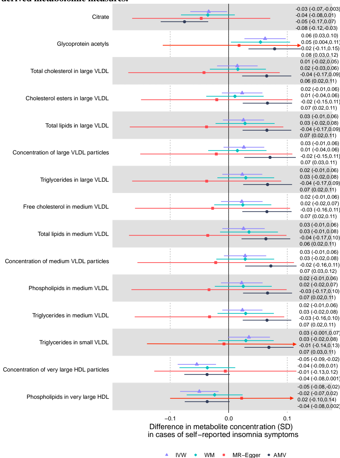
Figure shows inverse variance weighted (IVW) Mendelian randomization, Mendelian randomization sensitivity (weighted median (WM) and MR-Egger) and adjusted multivariable (AMV) regression analysis results. Results presented were selected on the basis of passing multiple testing threshold for either IVW or AMV ( p -values < 0.0029) The
