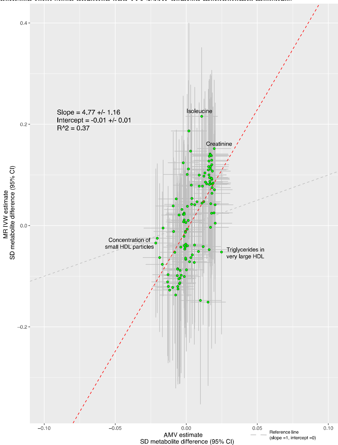
Figure 5: Comparison of the point estimates of the IVW Mendelian randomization and age-, sex- and BMI-adjusted multivariable regression analyses for the associations between total sleep duration and 112 NMR-derived metabolite measures
