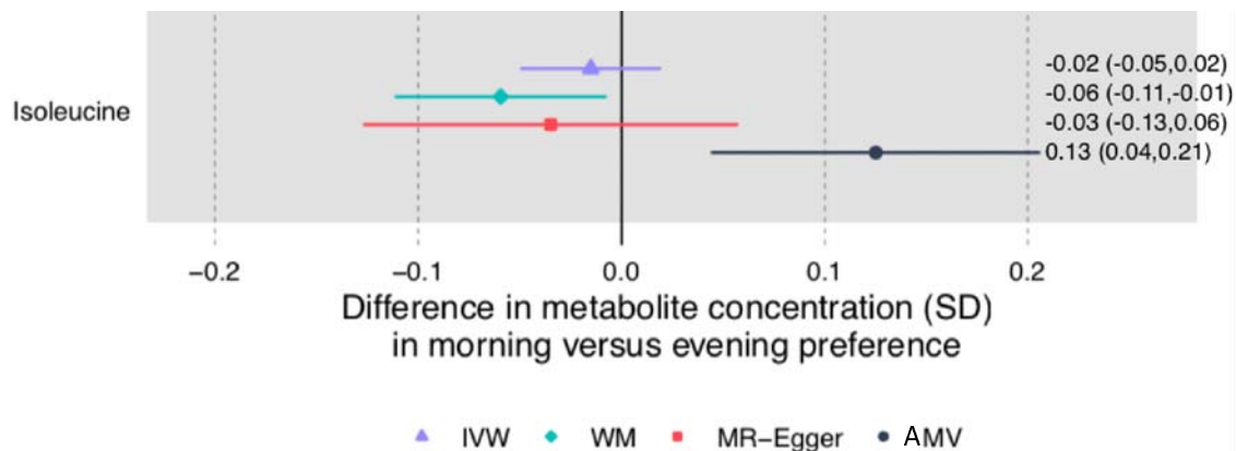
Figure 9: Mendelian randomization and age-, sex- and BMI-adjusted multivariable regression analyses results for selected associations of chronotype with NMR-derived metabolomic measures
