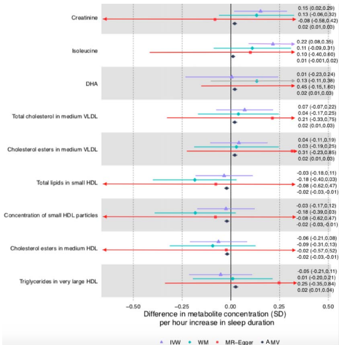
Figure shows inverse variance weighted (IVW) Mendelian randomization, Mendelian randomization sensitivity (weighted median (WM) and MR-Egger) and adjusted multivariable (AMV) regression analysis results. Results presented were selected on the basis of passing multiple testing threshold for either IVW or AMV ( p -values < 0.0029 ). The estimates are the difference in mean metabolite (in standard deviation units) per 1 hour greater total sleep duration. Abbreviations: AMV, adjusted (age, sex, BMI) multivariable regression; BMI, body mass index; DHA, 22:6, docosahexaenoic acid; HDL, high density lipoprotein; IVW MR, Inverse variance weighted Mendelian randomization; NMR, nuclear magnetic resonance; SD, Standard Error; WM, Weighted Median.
