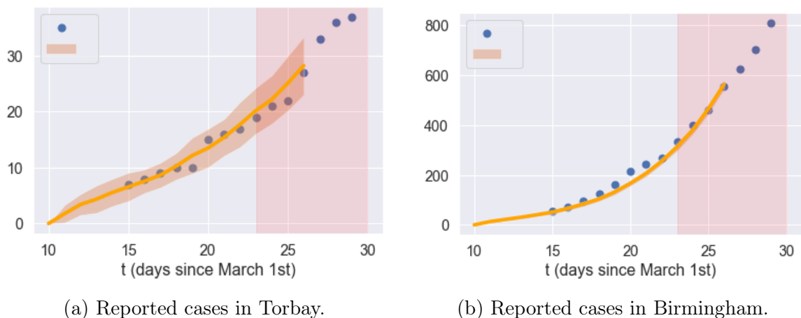
Figure 18: Dynamics of reported cases before lockdown in Torbay and Birmingham: data compared with heterogeneous model ( F ). Orange line: average of 1000 simulated scenarios; pink shade: lockdown period.
