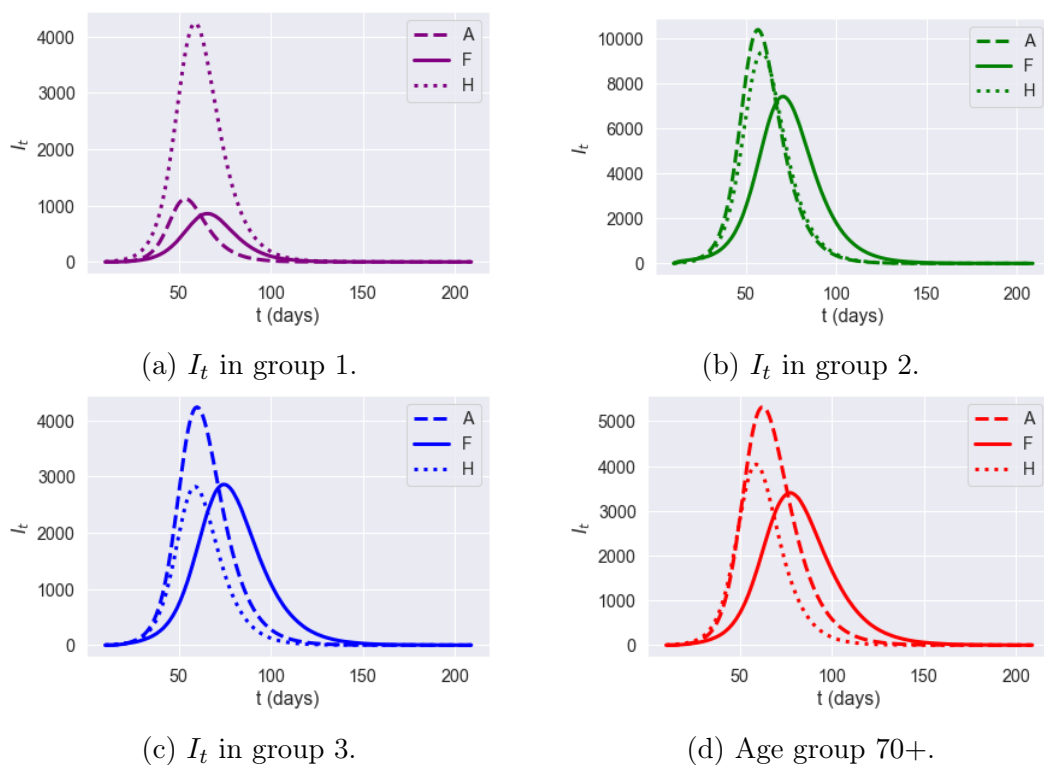
Figure 19: Dynamics of infections I_t in Torbay (UKK42): impact of model granularity.
