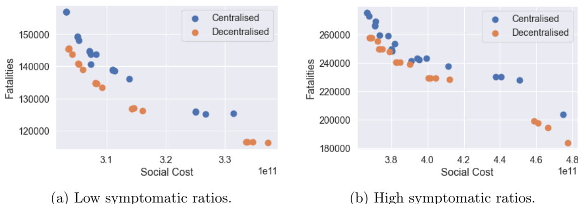
Figure 39: Efficiency analysis for centralised ( blue ) and decentralised ( orange ) adaptive mitigation policies. Outcomes are averaged across 100 simulated scenarios.
