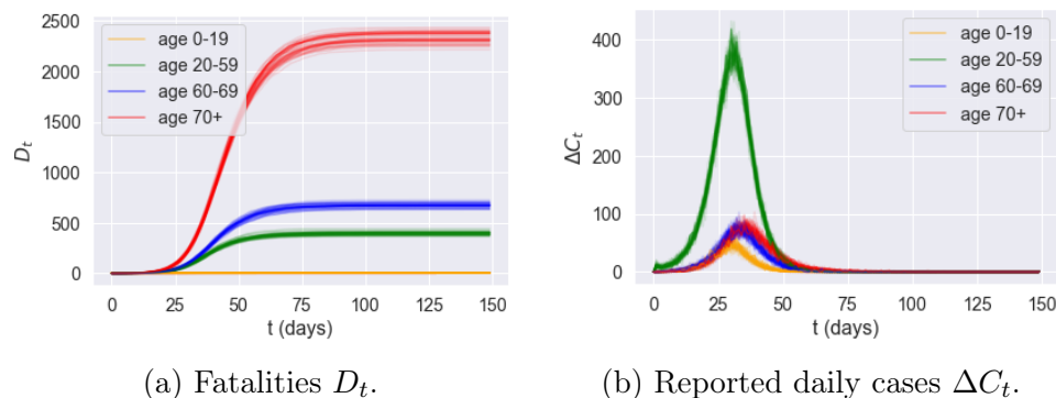
Figure 24: Effect of randomness: variability of outcomes across 50 sample paths for Birmingham (UKG31). (Low symptomatic ratios.)
