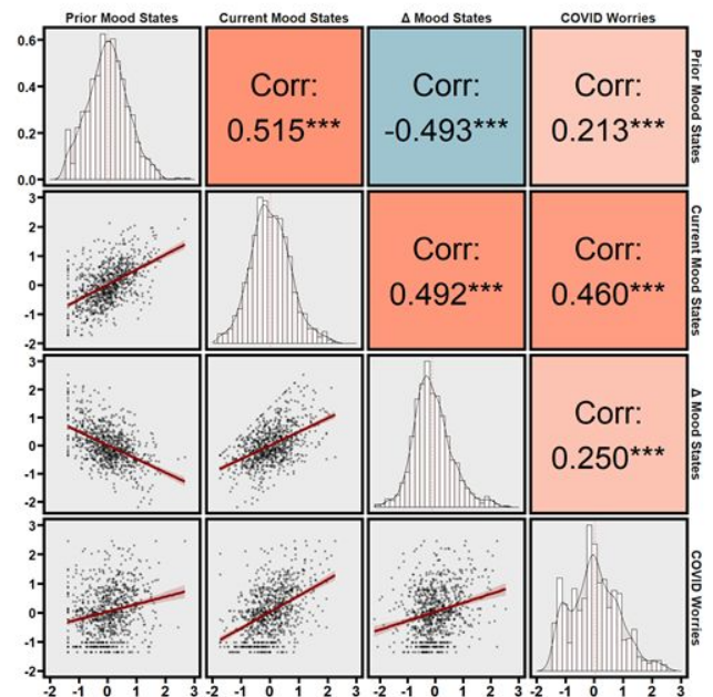
S Figure 2. Correlations between all factors scores (Prior Mood States, Current Mood States, \Delta Mood States, and COVID Worries) across all samples. Lower left panels display matrices of scatter plots of the correlation between the factors. X and Y label values represent a standard loading of -2 at the origin and 3 at the maximum for each of the factors. Corresponding diagonal panels show the histogram distribution of the factor correlations. Pearson correlation coefficient values are presented in the top right panels.
