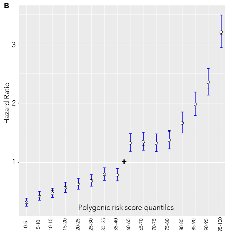
Figure 2. Hazard ratio estimates between quantiles 40-60 of the PC3 PRS and categorized 5% bins in the incident dataset. White dots and blue lines represent empirically estimated hazard ratio estimates and corresponding confidence intervals. Black dashes represent the theoretical hazard ratio for the 5%-quantile bins derived from the hazard ratio of per unit PRS. (A) Estonian Genome Center (B) UK Biobank.
