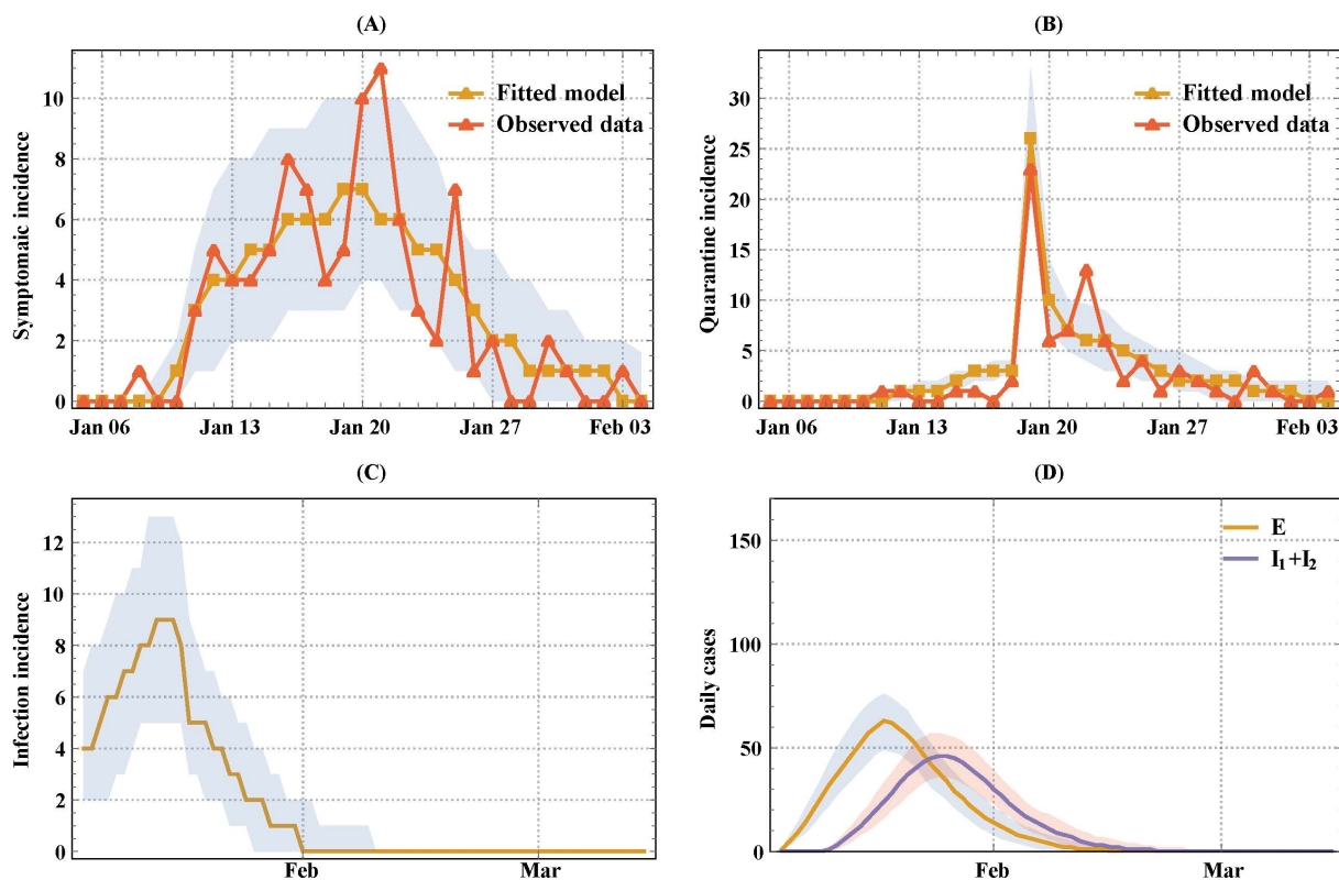
478 479 Figure 2: Model calibration and prediction. Panel A shows the observed and fitted daily incidence 480 of symptomatic cases ( E \rightarrow I_1 ). Panel B shows the observed and fitted daily quarantine cases among 481 HCWs. Panel C shows the predicted infection incidence ( S \rightarrow E ) from the calibrated model. Panel D 482 shows the corresponding predicted daily pre-symptomatic/ asymptomatic cases, E , and symptomatic 483 cases, I_1 + I_2 , respectively. The grey shaded regions are 90% credible intervals.
