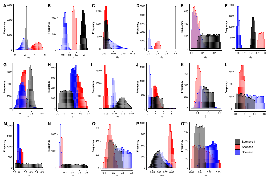
Figure 2: Histogram for each one of the parameters of System 2.1. Black, red and blue bars are related to Scenarios 1, 2, and 3, respectively.
