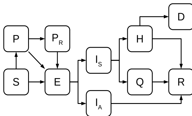
Figure 1: Flow diagram of the mathematical model. S, E, I_A, I_S, H, Q, R, D represent the populations of susceptible, exposed, asymptotically infected, symptomatically infected, hospitalized, quarantined, recovered and dead individuals, respectively. Protected individuals ( P ) get involved in the disease dynamics when mitigation measures are implemented, whereas released population ( P_R ) does so when relaxation of these measures occurs.
