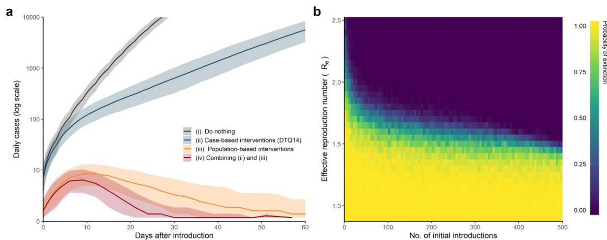
Fig. 4 Projections and joint effects of case-based and population-based interventions on probability of epidemic extinction. (a) The projected epidemic curves with 100 initial introductions under different scenarios regarding the intervention being implemented. The four scenarios included: (i) no intervention, (ii) case-based interventions only, (iii) population-based interventions only, and (iv) combining both case-based and population-based interventions. We assumed a sensitivity of 95% for case detection, an ascertainment probability for contact tracing of 90%, and a 72% reduction in background R_0 by population-based interventions ( R_0 : 2.5, R_p : 0.7). The uncertainty intervals were calculated by the 2.5th and 97.5th percentiles from 1000 replicate simulations. (b) The probability of epidemic extinction using case-based interventions (detection, contact tracing, and 14-day quarantine of close contacts) under different levels of population-based interventions ( R_p ) and initial numbers of introductions. Each cell presents the estimated probability of extinction based on 100 replicate simulations using the stochastic branching model.
