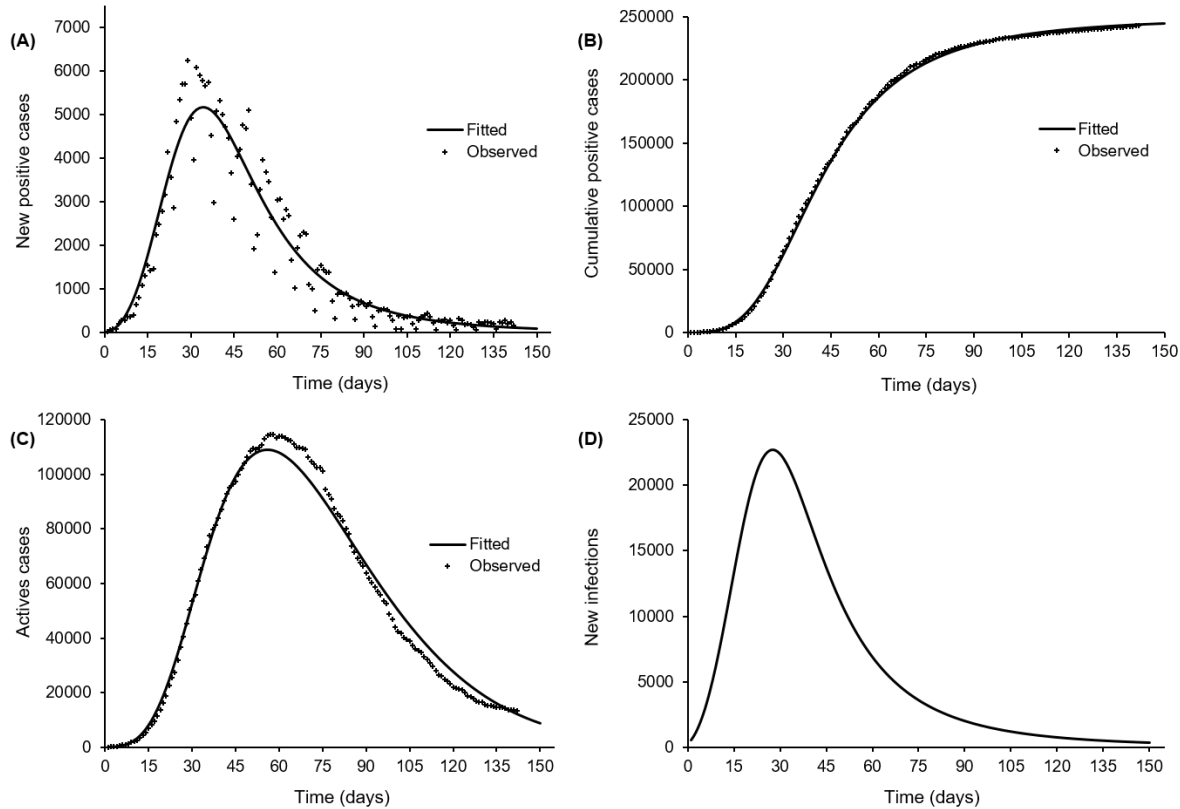
Fig 1. Log-normal fit of Turne’s generic growth curve to the italian COVID-19 daily case reporting data from 2020-02-20 to 2020-07-11 (A), cumul of positive cases (B), active (quarantined) cases (C) and estimated (average) daily new infections based on a detection rate of \delta = 0.033/\text{day} and a lost rate (recovery or death) of non detected cases of \pi = 0.1/\text{day} (D)
