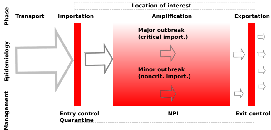
Figure 2: Spatialisation process: transport of cases from other locations; importation into the location of interest; local amplification; exportation to other locations. Red indicates control methods. See A.1 for details.
