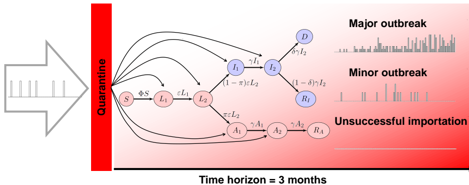
Figure 3: Input-output setting: imports arrive through transport, are potentially funnelled through quarantine, then enter one of the infected compartments. The three types of outcomes considered are shown on the right.
