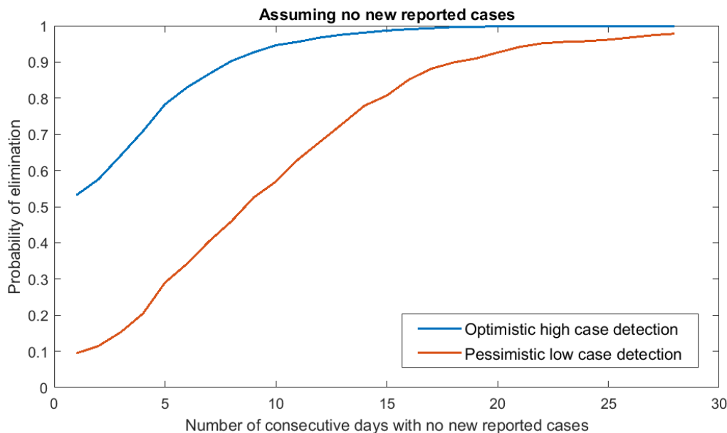
Figure 1: Probability of elimination, P(\text{elim}) , after different numbers of consecutive days with no new reported cases. Optimistic scenario with high detection and reporting of clinical cases ( p_R=75\% ) and moderate effectiveness of Alert Levels 2 ( C(t)=0.75 , \text{Reff}=1.8 ) and 3 ( C(t)=0.4 , \text{Reff}=0.95 ). Pessimistic scenario with low detection and reporting of clinical cases ( p_R=20\% ) and low effectiveness of Alert Levels 2 ( C(t)=0.95 , \text{Reff}=2.3 ) and 3 ( C(t)=0.9 , \text{Reff}=2.2 ).
