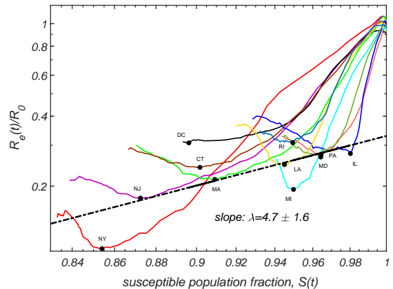
Fig. S3. Time progressions of R_e(t)/R_0 and S(t) for the hardest-hit US states and DC, as reported in Ref. (40). Black dots correspond to absolute minima of transmission and population susceptible fractions. The dashed line with slope \lambda = 4.7 \pm 1.6 is the best power law fit through these black dots.
