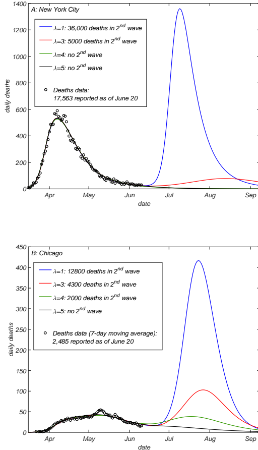
Fig. 3. Projections of daily deaths under the hypothetical scenario in which any mitigation is completely eliminated as of June 15 2020, for (A) NYC and (B) Chicago. Different curves correspond to different values of the immunity factor \lambda = 1 (blue), 3 (red), 4 (green) and 5 (black lines). The model described in Ref. (34) was fully calibrated on daily deaths (circles), ICU occupancy and hospitalization data up to the end of May. See Figs. S4-S5 in SI appendix for additional details, including confidence intervals.
