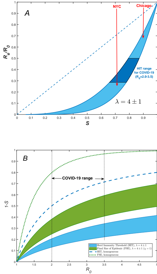
Fig. 1. A) R_e/R vs S dependence for gamma-distributed susceptibility for \lambda = 4 \pm 1 (blue area). The dashed line shows the classical homogeneous result, R_e = R_0 S . Note a substantial reduction of R_e for COVID-19 in both NYC and Chicago, compared to that value. Approximate fractions of susceptible populations, S , for both cities are estimated as of the end of May 2020, by using the model described in Ref. (34). B) Herd Immunity threshold (blue area) and final size of epidemic (FSE, green area) for gamma-distributed susceptibilities. The range of \lambda is the same as in (A). FSE is shown assuming maximum correlation between susceptibility and infectivity ( \chi = 1 ), which corresponds to CV_\alpha^2 ranging from 1 to 2. Notice a substantial reduction of both HIT and FSE compared to the classical results for homogeneous population which are shown as blue dashed and green dotted lines, respectively.
