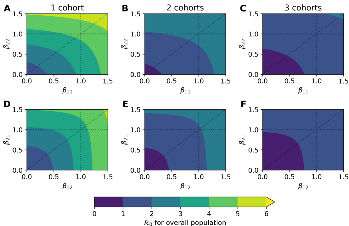
Figure 1: Predicted \mathcal{R}_0 under various density and rotating cohort scenarios. Results are based on a latent period of 3 days ( \sigma_1 = \sigma_2 = 1/3 ) and an infectious period of 4 days ( \gamma_1 = \gamma_2 = 1/4 ). We also assume weak interaction between cohorts ( \alpha_{k\ell} = 0.05 when k \neq \ell ). As the color gradient changes from purple to blue, \mathcal{R}_0 changes from < 1 to > 1 . (A–C) Varying values of \beta_{11} (child-to-child) and \beta_{22} (adult-to-adult) rates, assuming transmission between both is equal ( \beta_{12} = \beta_{21} = 0.5 ). (D–F) Varying values of \beta_{12} (child-to-adult) and \beta_{21} (adult-to-child), assuming transmission within adults is dominant ( \beta_{11} = 0.1 and \beta_{22} = 0.5 ).
