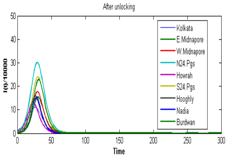
Figure A.43: Infected population when the transportation open within the full network (Time Vs I_i/10000 ). Infected population to reach at its peak for each of the nine districts will range between 23 to 32 days
