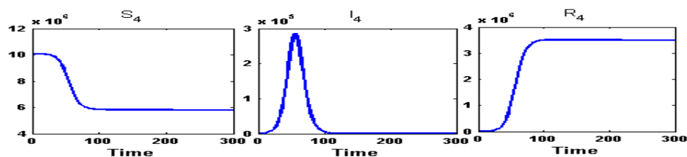
Figure 10: Susceptible ( S_4 ) class, Infected ( I_4 ) class and Recovered ( R_4 ) class people of North 24 Parganas( n_3 ) for intra-district network. During the partial lock-down, the infected population will reach at its peak of an amount of 2,86,100 infected person in 56 days and will go below the initial infected in 122 days.
