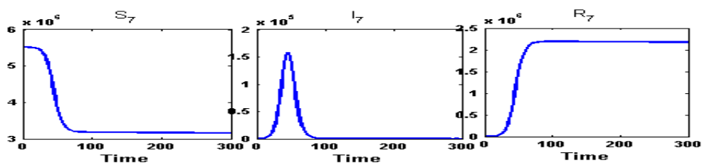
Figure 16: Susceptible ( S_7 ) class, Infected ( I_7 ) class and Recovered ( R_7 ) class people of Hooghly( n_6 ) for intra-district network. During the partial lock-down, the infected population will reach at its peak of an amount of 1,57,900 infected person in 45 days and will go below the initial infected in 98 days.
