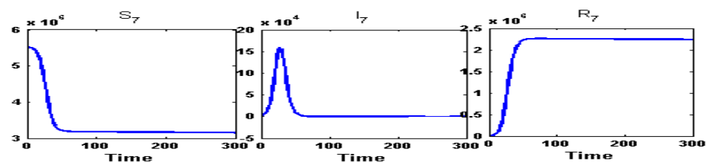
Figure A.36: Susceptible ( S_7 ) class, Infected ( I_7 ) class and Recovered ( R_7 ) class people of Hooghly( n_6 ) for intra-district network. During the partial lock-down, the infected population will reach at its peak of an amount of 1,60,000 infected person in 27 days and will go below the initial infected in 61 days.
