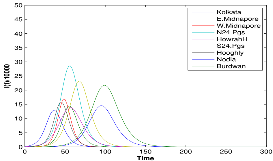
Figure 22: Infected population when the transportation open within their own network (Time Vs I_i/10000 ). Infected population to reach at its peak for each of the nine districts will range between 37 to 100 days
