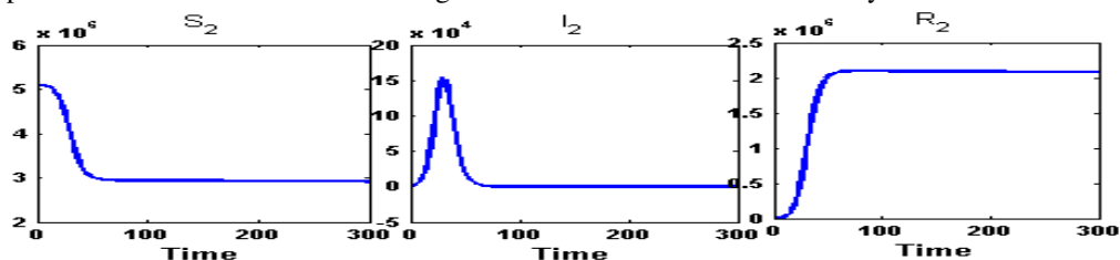
Figure A.27: Susceptible ( S_2 ) class, Infected ( I_2 ) class and Recovered ( R_2 ) class people of East Midnapore( n_1 ) for fully connected network. After the unlocking, within 30 days, the infected population will reach to its peak value at an amount 1,53,800 persons and will reduce down the initial amount of infection in 72 days.
