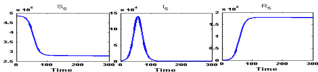
Figure 12: Susceptible ( S_5 ) class, Infected ( I_5 ) class and Recovered ( R_5 ) class people of Howrah( n_4 ) for intra-district network. During the partial lock-down, the infected population will reach at its peak of an amount of 1,39,200 infected person in 56 days and will go below the initial infected in 122 days.
