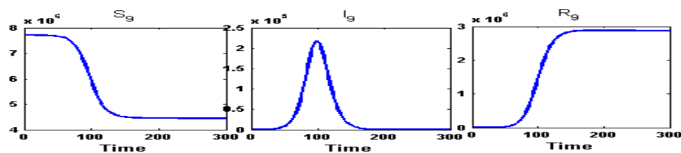
Figure 20: Susceptible ( S_9 ) class, Infected ( I_9 ) class and Recovered ( R_9 ) class people of Burdwan( n_8 ) for intra-connected network. During the partial lock-down, the infected population will reach at its peak of an amount of 2,17,400 infected person in 100 days and will go below the initial infected in 215 days
