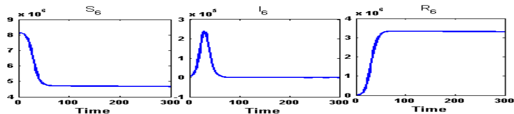
Figure A.35: Susceptible ( S_6 ) class, Infected ( I_6 ) class and Recovered ( R_6 ) class people of South 24 Parganas( n_5 ) for fully connected network. After the unlocking, within 30 days, the infected population will reach to its peak value at an amount 2,40,500 persons and down the initial amount of infection in 68 days.
