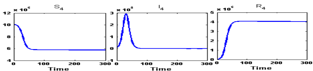
Figure A.30: Susceptible ( S_4 ) class, Infected ( I_4 ) class and Recovered ( R_4 ) class people of North 24 Parganas( n_3 ) for intra-district network. During the partial lock-down, the infected population will reach at its peak of an amount of 2,95,100 infected person in 31 days and will go below the initial infected in 66 days.
