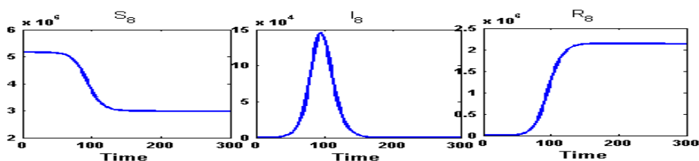
Figure 18: Susceptible ( S_8 ) class, Infected ( I_8 ) class and Recovered ( R_8 ) class people of Nadia( n_7 ) for intra-district network. During the partial lock-down, the infected population will reach at its peak of an amount of 1,45,400 infected person in 96 days and will go below the initial infected in 207 days.
