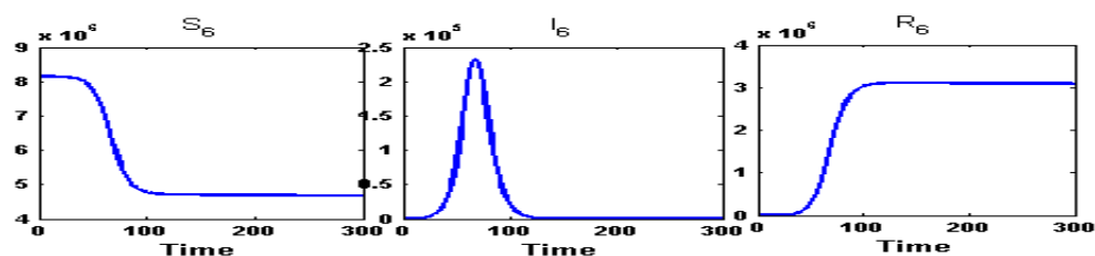
Figure 14: Susceptible ( S_6 ) class, Infected ( I_6 ) class and Recovered ( R_6 ) class people of South 24 Parganas( n_5 ) for intra-district network. During the partial lock-down, the infected population will reach at its peak of an amount of 2,32,400 infected person in 68 days and will go below the initial infected in 147 days.
