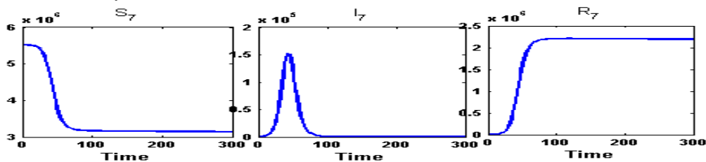
Figure 17: Susceptible ( S_7 ) class, Infected ( I_7 ) class and Recovered ( R_7 ) class people of Hooghly( n_6 ) for fully connected network. After the unlocking, within 43 days, the infected population will reach to its peak value at an amount 1,52,500 persons and down the initial amount of infection in 116 days.
