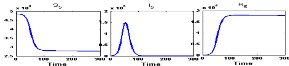
Figure 13: Susceptible ( S_5 ) class, Infected ( I_5 ) class and Recovered ( R_5 ) class people of Howrah( n_4 ) for fully connected network. After the unlocking, within 53 days, the infected population will reach to its peak value at an amount 1,50,100 persons and down the initial amount of infection in 119 days.
