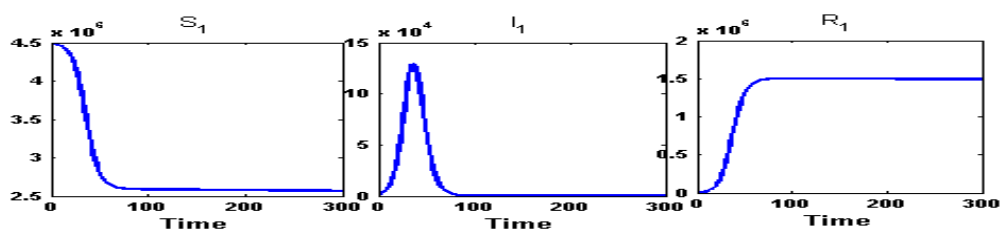
Figure 4: Susceptible ( S_1 ) class, Infected ( I_1 ) class and Recovered ( R_1 ) class people of Kolkata(C) for intra-district network. From an initial infection of an amount 1693 person, during partial lock-down within 37 days the number of infection would have reached at its peak value 1,29,200 and would go below the starting amount at around 79 days.
