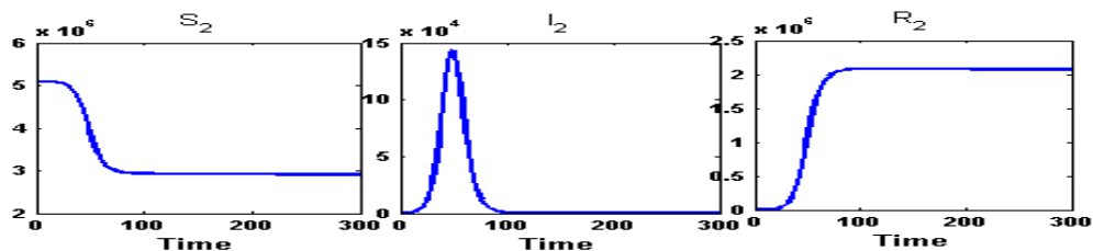
Figure 7: Susceptible ( S_2 ) class, Infected ( I_2 ) class and Recovered ( R_2 ) class people of East Midnapore( n_1 ) for fully connected network. After the unlocking, within 49 days, the infected population will reach to its peak value at an amount 1,43,700 persons and will reduce down the initial amount of infection in 125 days.
