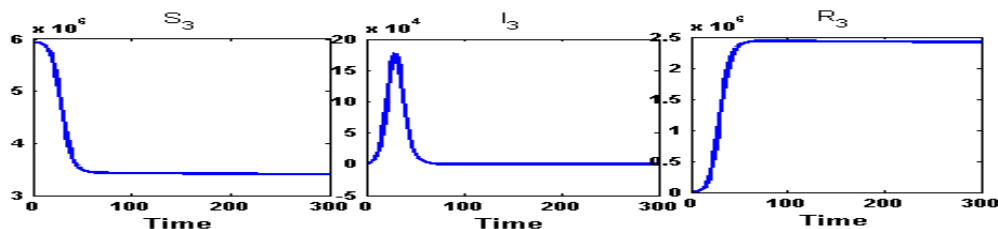
Figure A.29: Susceptible ( S_3 ) class, Infected ( I_3 ) class and Recovered ( R_3 ) class people of West Midnapore( n_2 ) for fully connected network. After the unlocking, within 43 days, the infected population will reach to its peak value at an amount 1,77,300 persons and down the initial amount of infection in 70 days.
