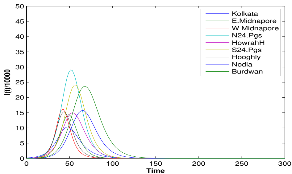
Figure 23: Infected population when the transportation open within the full network (Time Vs I_i/10000 ). Infected population to reach at its peak for each of the nine districts will range between 43 to 69 days
