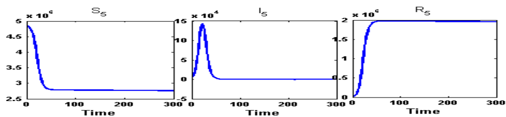
Figure A.32: Susceptible ( S_5 ) class, Infected ( I_5 ) class and Recovered ( R_5 ) class people of Howrah( n_4 ) for intra-district network. During the partial lock-down, the infected population will reach at its peak of an amount of 1,43,300 infected person in 22 days and will go below the initial infected in 48 days.
