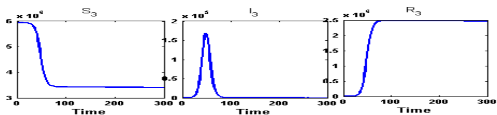
Figure 8: Susceptible ( S_3 ) class, Infected ( I_3 ) class and Recovered ( R_3 ) class people of West Midnapore( n_2 ) for intra-district network. During the partial lock-down, the infected population will reach at its peak of an amount of 1,68,900 infected person in 48 days and will go below the initial infected in 127 days.
