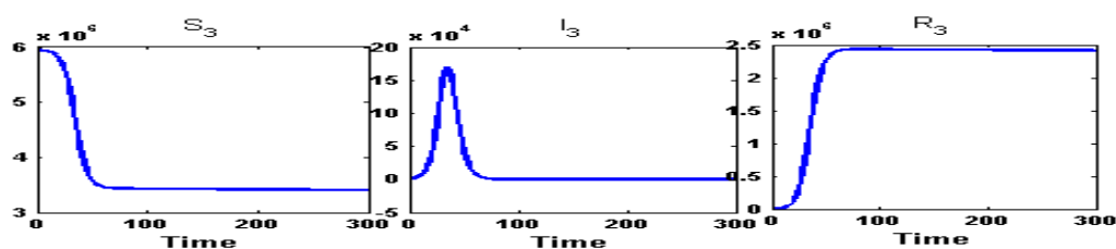
Figure A.28: Susceptible ( S_3 ) class, Infected ( I_3 ) class and Recovered ( R_3 ) class people of West Midnapore( n_2 ) for intra-district network. During the partial lock-down, the infected population will reach at its peak of an amount of 1,70,200 infected person in 35 days from the initial infected population of the amount 683 and will go below the initial infected in 75 days.
