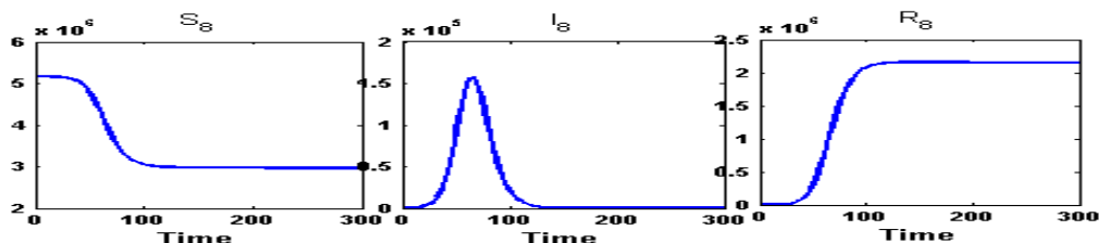
Figure 19: Susceptible ( S_8 ) class, Infected ( I_8 ) class and Recovered ( R_8 ) class people of Nadia( n_7 ) for fully connected network. After the unlocking, within 66 days, the infected population will reach to its peak value at an amount 1,57,100 persons and down the initial amount of infection in 175 days.
