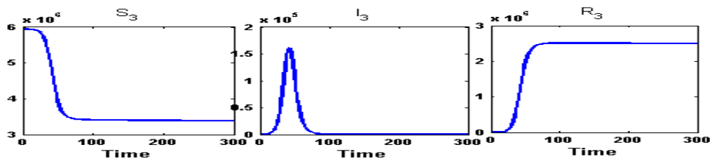
Figure 9: Susceptible ( S_3 ) class, Infected ( I_3 ) class and Recovered ( R_3 ) class people of West Midnapore( n_2 ) for fully connected network. After the unlocking, within 43 days, the infected population will reach to its peak value at an amount 1,61,300 persons and down the initial amount of infection in 128 days.
