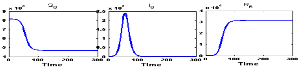
Figure 15: Susceptible ( S_6 ) class, Infected ( I_6 ) class and Recovered ( R_6 ) class people of South 24 Parganas( n_5 ) for fully connected network. After the unlocking, within 58 days, the infected population will reach to its peak value at an amount 2,39,100 persons and down the initial amount of infection in 137 days.
