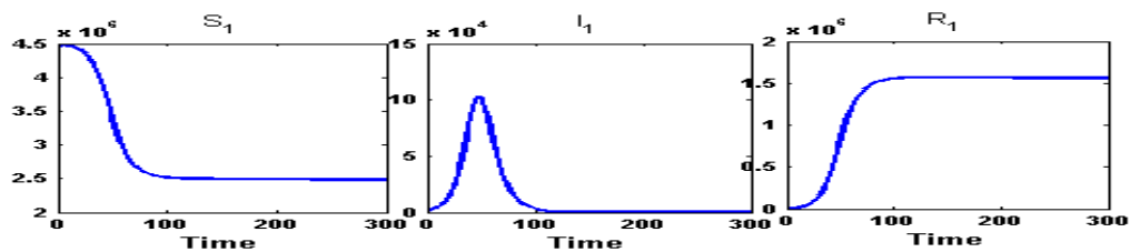
Figure 5: Susceptible ( S_1 ) class, Infected ( I_1 ) class and Recovered ( R_1 ) class people of Kolkata(C) for fully connected network. After the formation of network between these closely related district, the infected population will reach to it's peak value at an amount 1,03,000 person in 47 days and will go down the initial level of infection in 110 days.
