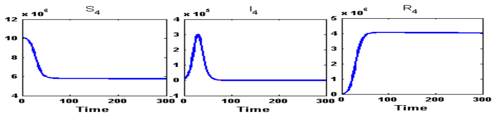
Figure A.31: Susceptible ( S_4 ) class, Infected ( I_4 ) class and Recovered ( R_4 ) class people of North 24 Parganas( n_3 ) for fully connected network. After the unlocking, within 30 days, the infected population will reach to its peak value at an amount 3,00,900 persons and down the initial amount of infection in 64 days.
