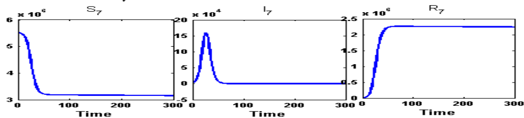
Figure A.36: Susceptible ( S_7 ) class, Infected ( I_7 ) class and Recovered ( R_7 ) class people of Hooghly( n_6 ) for intra-district network. During the partial lock-down, the infected population will reach at its peak of an amount of 1,60,000 infected person in 27 days and will go below the initial infected in 61 days.
