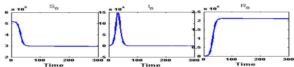
Figure A.38: Susceptible ( S_8 ) class, Infected ( I_8 ) class and Recovered ( R_8 ) class people of Nadia( n_7 ) for intra-district network. During the partial lock-down, the infected population will reach at its peak of an amount of 1,48,400 infected person in 33 days and will go below the initial infected in 70 days.
