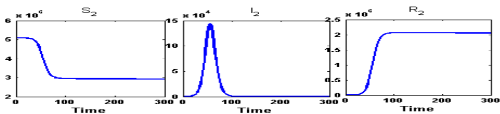
Figure 6: Susceptible ( S_2 ) class, Infected ( I_2 ) class and Recovered ( R_2 ) class people of East Midnapore( n_1 ) for intra-district network. During the partial lock-down, the infected population will reach at its peak of an amount of 1,43,800 infected person in 56 days and will go below the initial infected in 120 days.
