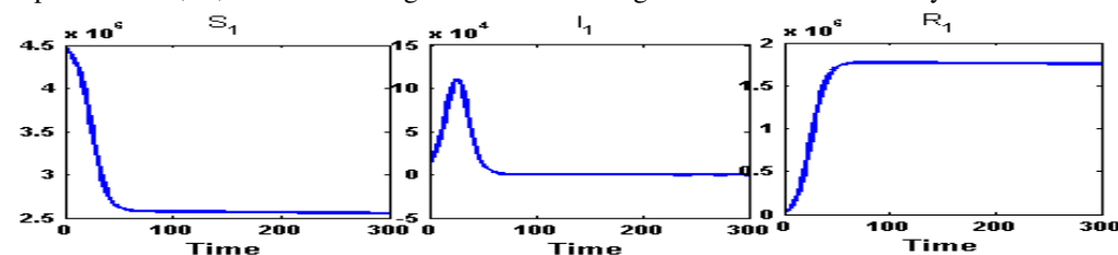
Figure A.25: Susceptible ( S_1 ) class, Infected ( I_1 ) class and Recovered ( R_1 ) class people of Kolkata(C) for fully connected network. After the formation of network between these closely related district, the infected population will reach to it's peak value at an amount 1,10,900 person in 26 days and will go down the initial level of infection in 51 days.
