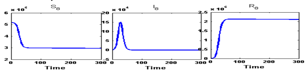
Figure A.39: Susceptible ( S_8 ) class, Infected ( I_8 ) class and Recovered ( R_8 ) class people of Nadia( n_7 ) for fully connected network. After the unlocking, within 28 days, the infected population will reach to its peak value at an amount 1,51,300 persons and down the initial amount of infection in 66 days.
