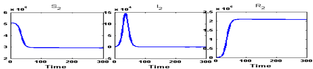
Figure A.26: Susceptible ( S_2 ) class, Infected ( I_2 ) class and Recovered ( R_2 ) class people of East Midnapore( n_1 ) for intra-district network. During the partial lock-down, the infected population will reach at its peak of an amount of 1,46,000 infected person in 37 days from the initial infected population of the amount 765 and will go below the initial infected in 79 days.
