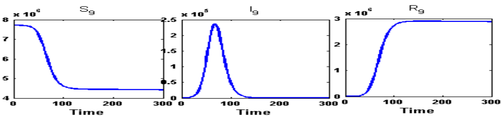
Figure 21: Susceptible ( S_9 ) class, Infected ( I_9 ) class and Recovered ( R_9 ) class people of Burdwan( n_8 ) for fully connected network. After the unlocking, within 69 days, the infected population will reach to its peak value at an amount 2,36,600 persons and down the initial amount of infection in 182 days.
