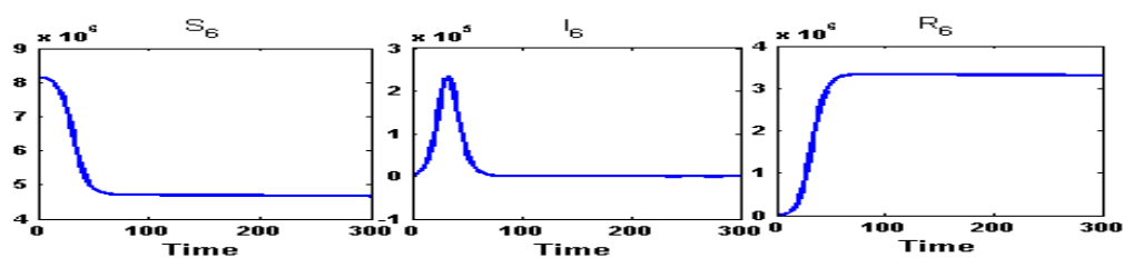
Figure A.34: Susceptible ( S_6 ) class, Infected ( I_6 ) class and Recovered ( R_6 ) class people of South 24 Parganas( n_5 ) for intra-district network. During the partial lock-down, the infected population will reach at its peak of an amount of 2,34,600 infected person in 33 days and will go below the initial infected in 72 days.
