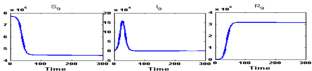
Figure A.40: Susceptible ( S_9 ) class, Infected ( I_9 ) class and Recovered ( R_9 ) class people of Burdwan( n_8 ) for intra-connected network. During the partial lock-down, the infected population will reach at its peak of an amount of 1,60,000 infected person in 27 days and will go below the initial infected in 66 days
