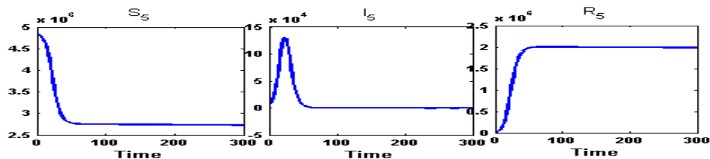
Figure A.33: Susceptible ( S_5 ) class, Infected ( I_5 ) class and Recovered ( R_5 ) class people of Howrah( n_4 ) for fully connected network. After the unlocking, within 53 days, the infected population will reach to its peak value at an amount 1,31,300 persons and down the initial amount of infection in 53 days.
