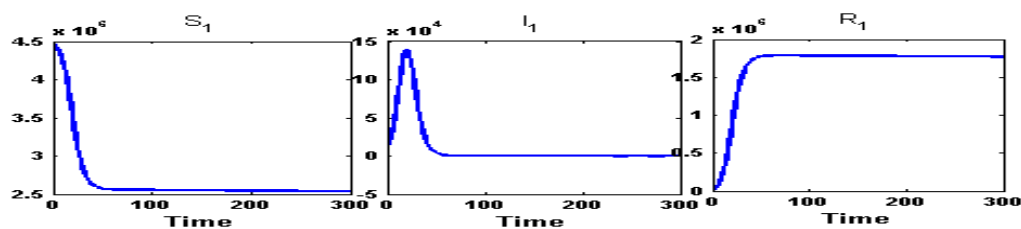
Figure A.24: Susceptible ( S_1 ) class, Infected ( I_1 ) class and Recovered ( R_1 ) class people of Kolkata(C) for intra-district network. From an initial infection of an amount 12682 person on 18th July, during partial lock-down within 21 days the number of infection would have reached at its peak value 1,38,700 and would go below the starting amount at around 44 days.
