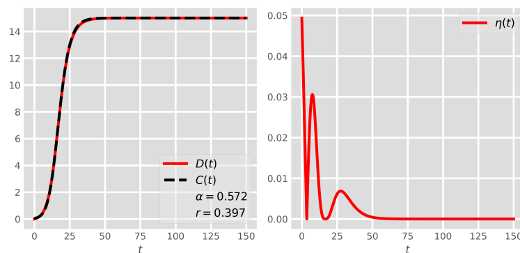
Figure 1: Illustrative picture (left panel) of the map between the Richards model and the SIRD model with constant parameters. The relative error function between the two models is shown in the right panel.
