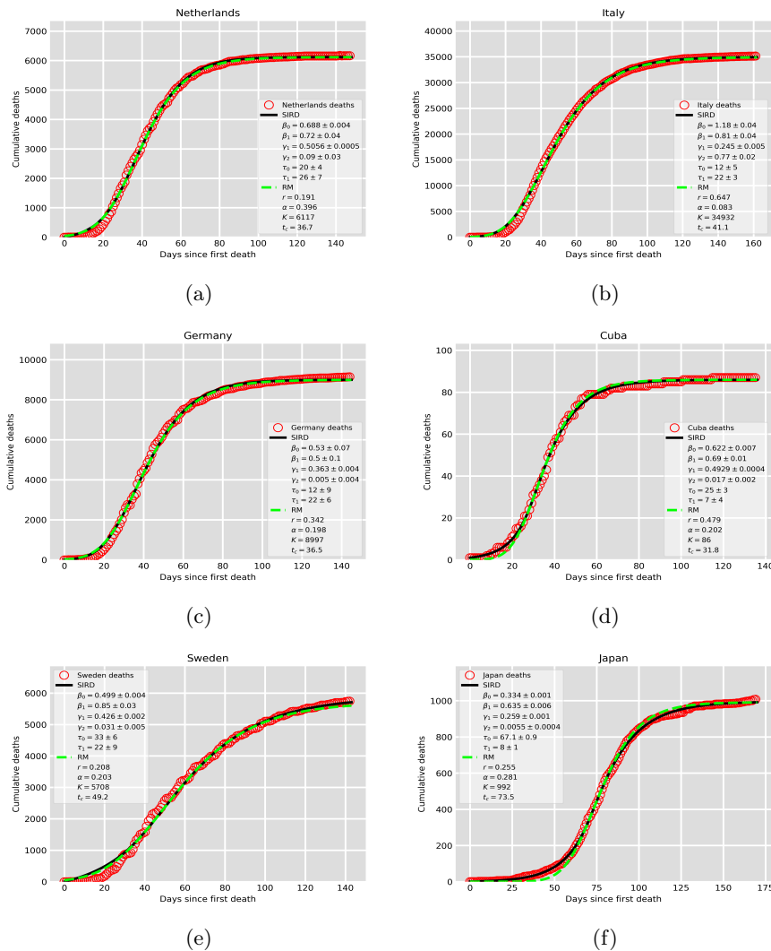
Figure 3: Cumulative number of deaths (red circles) attributed to COVID-19, up to July 30, 2020, for (a) Netherlands, (b) Italy, (c) Germany, (d) Cuba, (e) Sweden, and (f) Japan. The solid black curves are the best fits by the SIRD model with a time-dependent \beta(t) , where the parameter estimates are given in the inset. The bright green dashes curve is the theoretical curve obtained from the Richards model, with the parameters computed from the numerically determined parameters of the SIRD model via the map (3.19) and (3.20).
