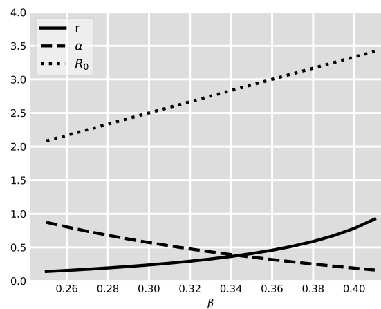
Figura 2: Behavior of the Richards parameters ( r, \alpha ) and R_0 as a function of the parameter \beta of the SIRD model.
