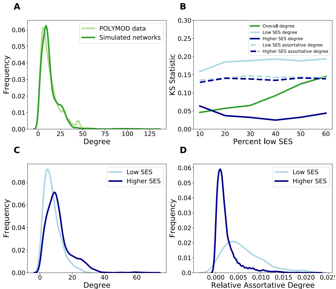
Figure 1: The network characteristics of the networks generated from the ERGM model based on POLYMOD data. A: The degree distribution of the POLYMOD data (light green) compared to the simulated networks (dark green). B: The Kolmogorov-Smirnov (KS) statistic to evaluate the dissimilarity of the ERGM-simulated networks to the POLYMOD data as additional low education individuals are added to the network. KS statistics compare the dissimilarity of the overall degree distribution (dark green), the degree distribution of low SES nodes (light blue, solid), the degree distribution of higher SES nodes (dark blue solid), the assortative degree (e.g. the low SES contacts of low SES nodes) for low SES nodes (light blue, dashed), and the assortative degree for higher SES nodes (dark blue, dashed). Low KS values indicate similar distributions. C: The degree distribution of low SES nodes (light blue) and higher SES nodes (dark blue). D: The relative assortative degree distribution (e.g. number of low SES contacts of low SES nodes/number of low SES nodes) of low SES nodes (light blue) and other SES nodes (dark blue).
