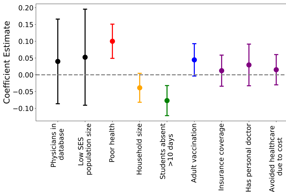
Figure 4: Mean model coefficient estimates and credible intervals. Points are colored by what process each covariate represents (black: measurement bias, red: susceptibility, orange: social contact differences, green: sickness absenteeism, blue: vaccination, purple: healthcare utilization).
