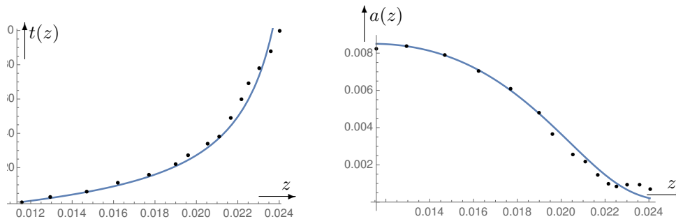
Figure 4: Left figure: reported data \{z_n, t_n\} for Germany and associated fit curve t(z) . Right figure: curve a(z) calculated from t(z) with Eq. (17) together with the reported data \{z_n, a_n\} .
