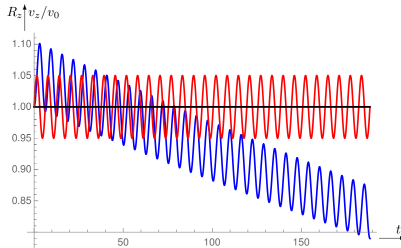
Figure 6: The horizontal curve is R_z(t) , the top-down curve v_z(t)/v_0 .
