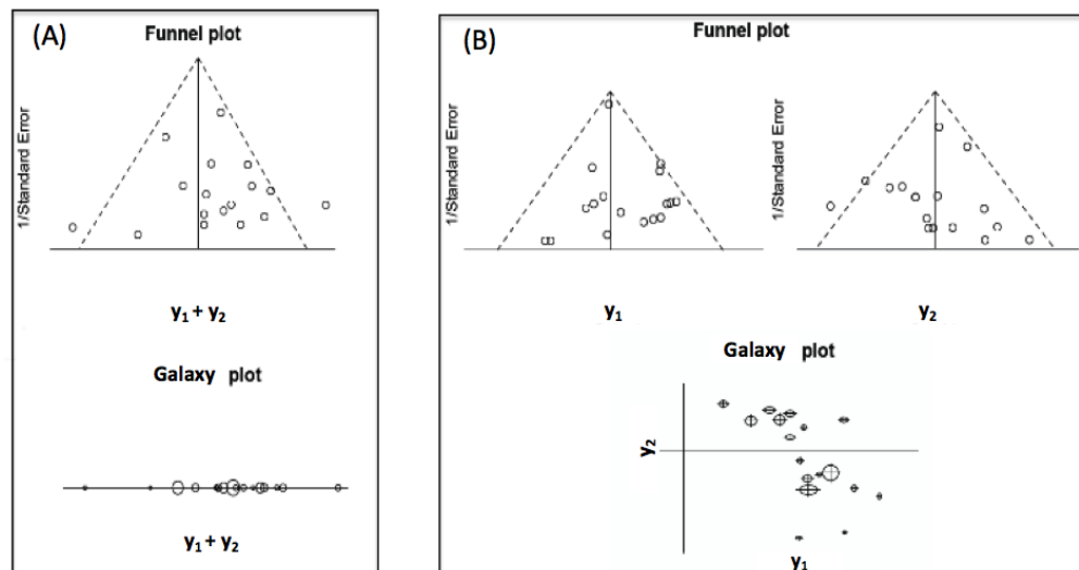
Figure 1. (A) The upper panel is the funnel plot for a univariate meta-analysis. The lower panel shows the galaxy plot reduced to a one-dimensional space, which retains all information of the funnel plot as the standard error is represented by each study's circle radius. (B) The upper panel shows two separate funnel plots for the two outcomes in a bivariate meta-analysis. They can be integrated into the galaxy plot in a two-dimensional space in the lower panel.
