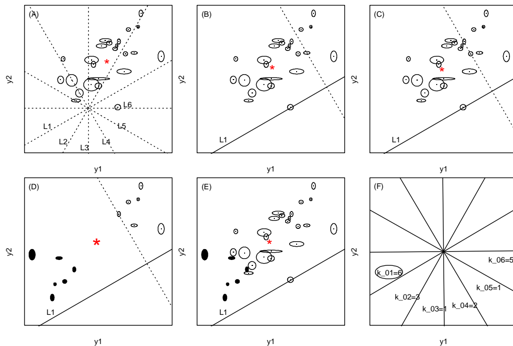
Figure 2. Bivariate trim and fill method to identify and correct for small-study effects in the galaxy plot of a bivariate meta-analysis. (A) The galaxy plot shows 24 simulated studies and the dashed lines represent M=6 directions. The red star is the center. (B) For the first direction L_1 , the first iteration trims 4 studies with the largest weighted scores, using the univariate trim and fill method. The red star represents the updated center using the 22 studies. (C) The second iteration trims two more studies and the red star represents the updated center using the 20 studies. No more studies are trimmed in the next iteration so the number of trimmed studies is k_{01} = 6 . (D) 6 studies are filled by point symmetry about the center, with equal standard errors. (E) The center is estimated based on the 30 fully augmented studies. (F) Repeated steps as in (B)–(E) for other directions with \{k_{0m}, m = 2, \dots, M\} , implying that L_1 is the optimal direction since k_{01} is the largest.
