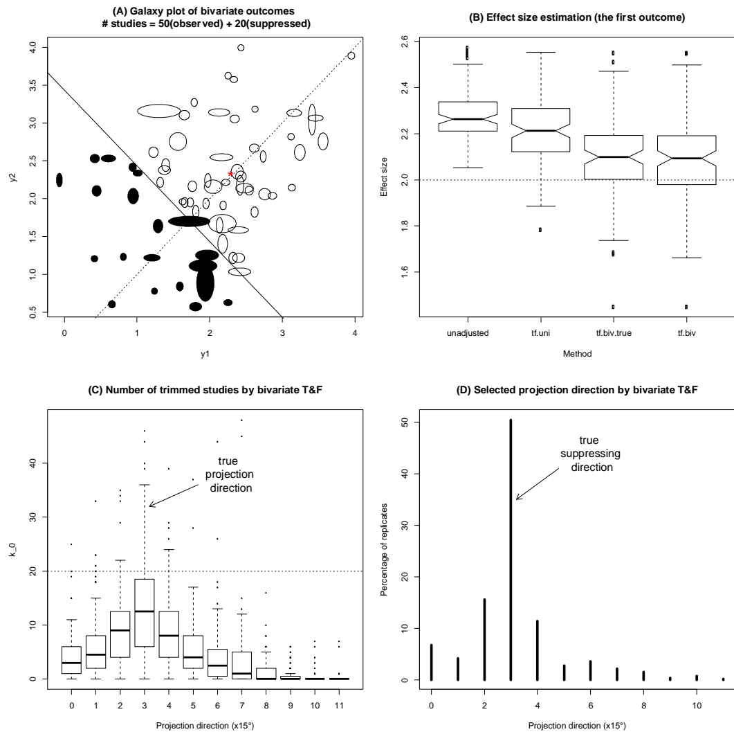
Figure 3. Simulation study results of 200 replicates of meta-analyses, each containing 50 observed studies after suppressed 20 studies. (A) The galaxy plot showing a typical simulated bivariate meta-analysis dataset according to a random-effect model. The 70 studies are projected to the true projection line (dashed line, 45^\circ to the x axis) among which 20 studies with the smallest projected values (to the lower left of the solid line) are suppressed and the other 50 studies (to the upper right of the solid line) are observed. (B) The effect size estimation of the unadjusted multivariate meta-analysis (unadjusted), the univariate T&F (tf.uni), the bivariate T&F along the true projection direction (tf.biv.true) and the bivariate T&F using the searching algorithm (tf.biv). (C) The estimation of the number of suppressed studies ( k_0 ) along each of the candidate projection directions. The true value is 20. (D) The selected projection direction by the searching algorithm. Lines represent the percentages of times each direction was selected (with the most studies been trimmed) among the 200 replicates.
