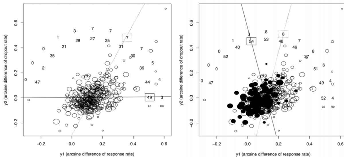
Figure 4. The number of trimmed studies by the proposed bivariate T&F method in the antidepressant meta-analysis of Cipriani et al [16]. The two outcomes are the arcsine differences of response rate and dropout rate between antidepressants and placebo. The 288 published studies are presented in the galaxy plot in the left panel while 89 “grey literature” studies (colored) are additionally included in the right panel. The number of trimmed studies along the 12 directions of projection are shown, where the inner and outer circles are for L_0 and R_0 estimators respectively. The direction with maximum number of trimmed studies is selected.
