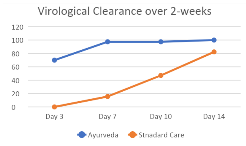
Figure 1: comparing virologic clearance over the two weeks
