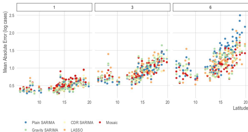
Figure 6. Mean absolute error for the best model in each class at t+1 , t+3 , and t+6 forecasting horizons for all provinces. The mean absolute error (y-axis) on the prediction (i.e., log) scale of the best model for each class for all provinces (x-axis). Provinces are ordered by latitude (x-axis, right is more northerly). There is a general decline in predictive power at farther forecasting horizons and at more northerly provinces; however, no single model or class of model performs best across all areas and all prediction horizons.
