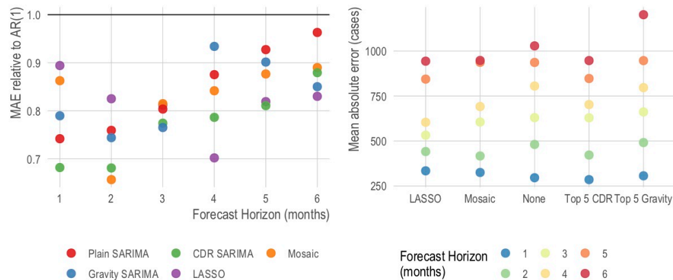
Figure 5. Comparing the best models for Bangkok, by model type. Focusing only on the best performing model for each model type and each time horizon, we show the relative mean absolute error (left panel) and the mean absolute error (right panel). On the left, the baseline of comparison is the traditional AR(1) model and the y-axis can be interpreted as the improvement over this baseline — i.e., a value of .9 indicates a 10% improvement. We show that both the Plain SARIMA (red) and CDR SARIMA (green) models perform better than the LASSO model at earlier forecasting horizons but perform worse at later horizons.
