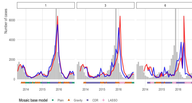
Figure 7. Mosaic model vs AR(1) for Bangkok at t+1, t+3, and t+6 forecasting horizons. We show the predictions for a simple mosaic model at t+1, t+3, and t+6 forecasting horizons for Bangkok in blue. For comparison, we show predictions from an AR(1) in red and observed cases in grey bars. Under each bar, we indicate the base model selected by the mosaic ensemble using a winter-takes-all approach based on the previous three out-of-sample prediction months.
