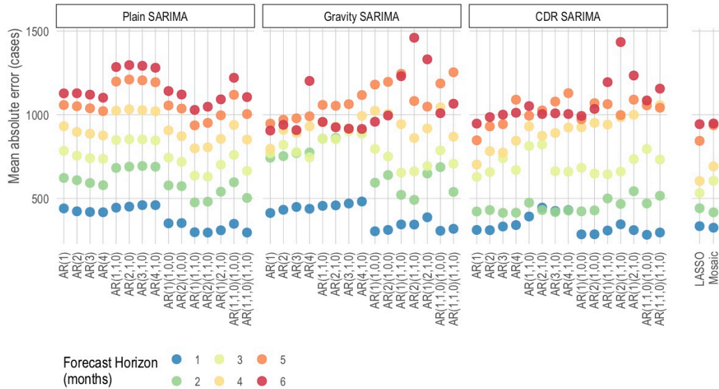
Figure 4. Mean absolute error (MAE) for all Bangkok models. The mean absolute error (y-axis) expressed as number of cases for each model (x-axis) and for each forecast. Models are grouped as SARIMA with no exogenous variables (Plain), SARIMAs with the top 5 most connected regions based on the predicted trips from a gravity model (Gravity SARIMA), and SARIMAs with the top 5 most connected regions based on CDR data (CDR SARIMA). The rightmost models show a data-driven network model, denoted as LASSO, since it is based on a least absolute shrinkage and selection operator prediction model, and mosaic model.
