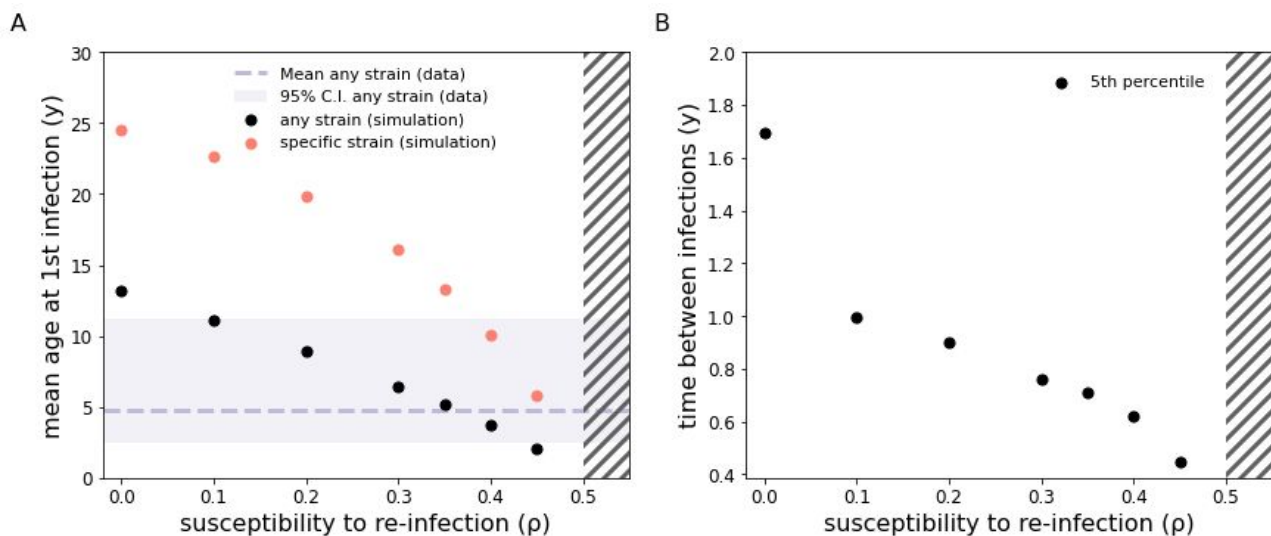
Figure 2: Impact of \rho on eHCoV dynamics and emergent strain hospitalisation rates. (A) Mean age at first infection with any eHCoV (black dots) and with a specific strain (red dots) as a function of \rho . The dashed line and band represent respectively the mean and 95% C.I. for the age at first infection with any eHCoV obtained from a pooled estimate (42). (B) 5th percentile of the time between consecutive infections by the same strain. Hatches indicate the \rho > 1/R_0 region (for R_0 = 2 ) where the dynamics are SIS-like (whereas for \rho < 1/R_0 we observe epidemic behaviour). It should be noted that for \rho = 0 reinfection still occurs in our model because of external introductions, which we have assumed for simplicity to ignore pre-existing immunity to reinfection. Nonetheless, reinfection events induced by external
