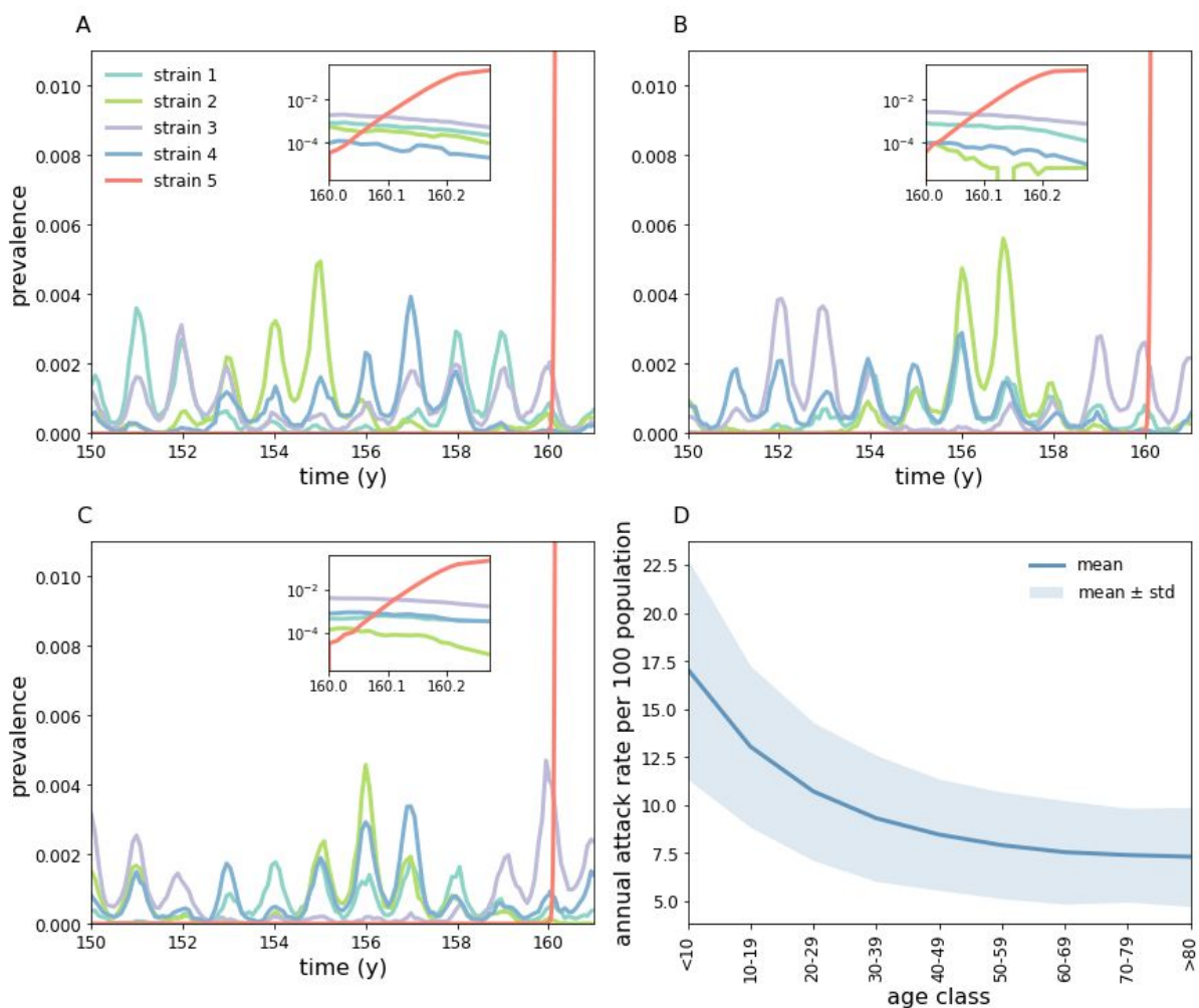
Figure 1: Simulated transmission of eHCoVs. (A-C) Stochastic realisations of the multi-strain model obtained using baseline parameters. At time t = T_{inv} = 160 y we randomly infect 10 individuals with the emergent strain (red). Insets: zoom on the first 100 days after introduction of the emergent strain. (D) Annual attack rate per 100 population by age class for all four eHCoVs. The attack rate decreases and plateaus with age since individuals accumulate immunity through consecutive infections with different eHCoVs.
