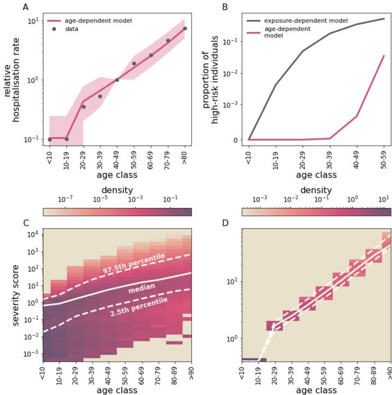
Figure 5: Implications of HCoV-exposure- and age-dependent-severity. (A) A model where disease severity depends only on age (the age-dependent model) is able to explain hospitalisation rates in EU/EEA countries and the UK (dots). Line and filled area represent mean and 95% C.I., respectively. Here, we set a_{age} = 0.4 , b_{age} = 0.052 y^{-1} and A_0 = 20 y . Results are averaged over 100 samplings from each of 50 different simulations. (B) Individual risk of developing severe symptoms under exposure-dependent (black) and the age-dependent severity (fucsia). (C,D) Severity score distribution within each age class under exposure-dependant and age-dependent severity, respectively. Solid and dashed lines indicate the median score and the 95% percentile range, respectively. Please note that C,D have different scales. To estimate individual risk in (B), we first selected \bar{N} = 3 \cdot 10^4 individuals completely at random in a single simulation (that is, we assume uniform infection rates across all age ranges) and then sampled a fraction \pi = 0.05 of these \bar{N} cases according to the sampling scheme outlined in the Methods section. This operation was repeated 2 \cdot 10^3 times. Finally, we computed the proportion of high-risk individuals as the fraction of sampled cases whose risk is larger than the 25th percentile in the >60 years age range. In C,D, the score distribution is computed from a single simulation at the time of the introduction of the emergent strain. We set epidemiological parameters to their baseline values and a = 1.5 , b = 0.5 , r = 0.05 y^{-1} .
