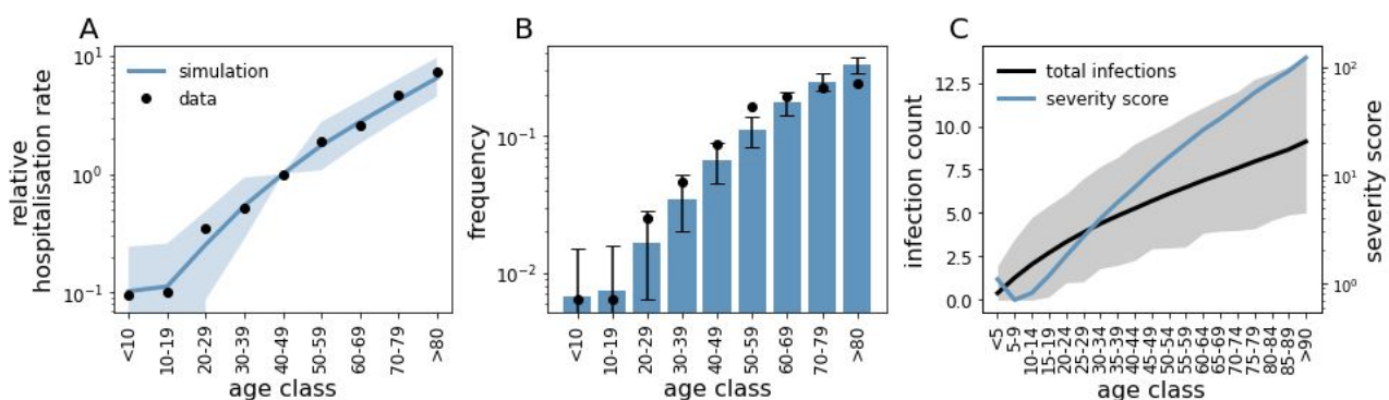
Figure 4: Comparison between model predictions and hospitalisation data for EU/EEA countries and the UK. (A) Simulated hospitalisation rates (blue line) and data (dots). The value corresponding to the 40-49y age range has been set to 1 for convenience and remaining values have been scaled accordingly. The shaded area indicates the 95% C.I. from simulations. (B) Age distribution of hospitalised cases in EU/EEA countries and the UK (dots) and mean distribution from simulations (bars). Error bars indicate the 95% C.I. from simulations. (C) Mean number of cumulative infections and severity score as a function of age (black and blue lines, respectively), at the time of the introduction of the emergent strain. Shaded area indicates the 95% C.I. from simulations. Here, we set \pi = 0.05 , a = 1.5 , b = 0.5 , r = 0.05 \text{ y}^{-1} . Because our aim is mainly to illustrate the role of disease enhancement and cross-protection, we did not attempt to fit parameters a (baseline risk), b (boosting factor) and r (waning of cross-protection). Rather, we manually adjusted parameters in order to obtain a good visual agreement between data and simulations. Goodness of fit for chosen parameters was measured at R^2 = 0.98 . Results are averaged over 100 samplings from each of 50 different simulations. Other parameters are set to baseline values.
