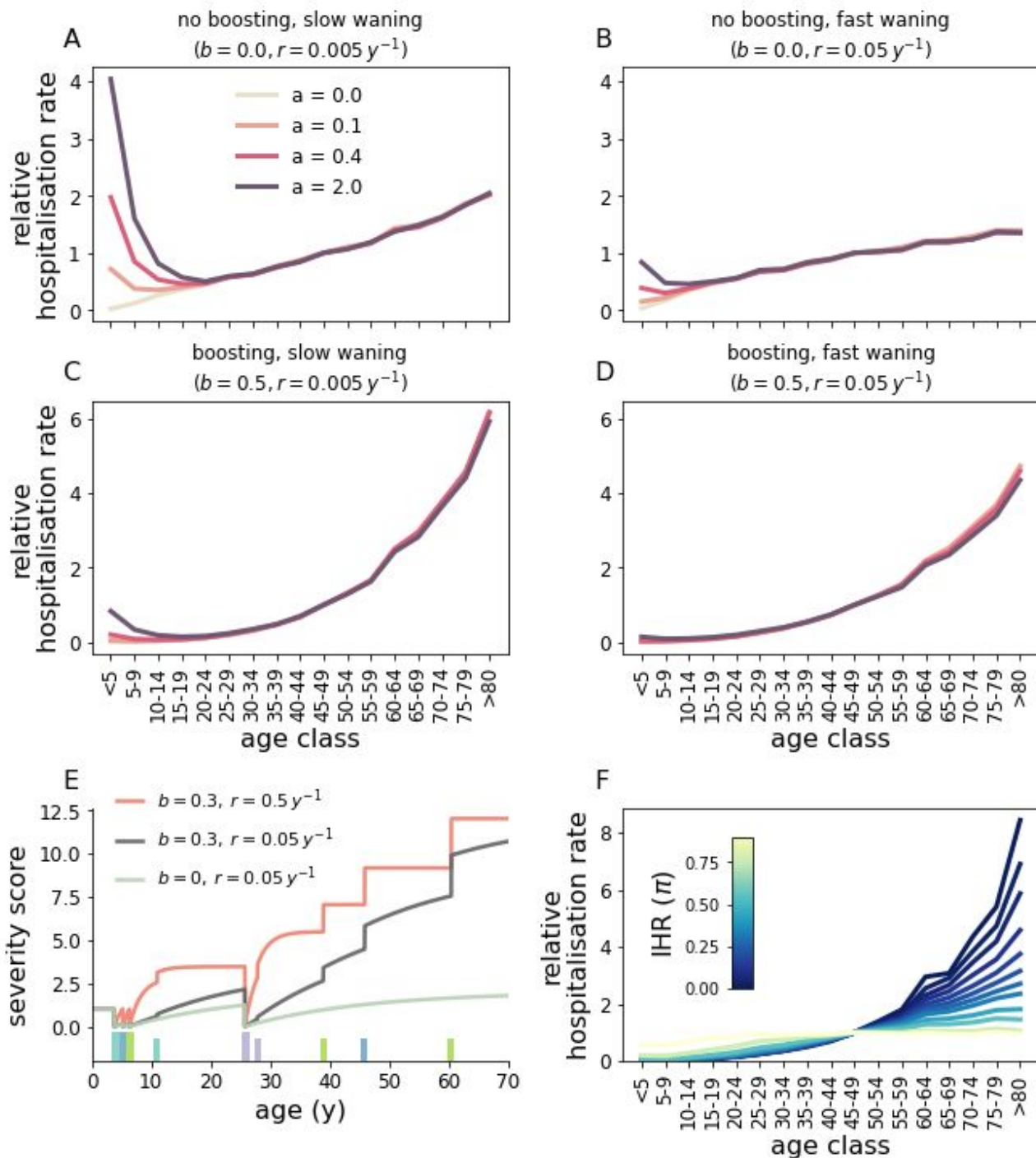
Figure 3: Impact of b (boosting factor), r (waning of cross-protection), a (baseline risk) and \pi (IHR) on age-specific hospitalisation rates. Panels (A-D) correspond to different combinations of parameters b and r . Within each panel, different curves correspond to different values of a . Here we assumed that a fraction \pi = 0.1 of all cases are hospitalised. For visualisation purposes, the rate corresponding to the 45-49y age range is set to one and the remaining rates are re-scaled accordingly. (E) Temporal evolution of the severity score for a single host under different combinations of b , r and a = 1 . We considered three scenarios corresponding to no boosting and slow waning of cross-protection (green line, b = 0, r = 0.05 \text{ y}^{-1} ), boosting and slow waning of cross-protection (black line, b = 0.3, r = 0.05 \text{ y}^{-1} ), boosting and fast waning of cross-protection (red line, b = 0.3, r = 0.5 \text{ y}^{-1} ). Bars indicate infection events, with each color corresponding to a different eHCoV. At birth, the score is identically equal to a . The score drops to 0 after encountering a new strain (thicker and taller bars), but increases thereafter at rate r . Secondary infections with the same eHCoV (smaller bars) do not provide any additional protection and only increase the score for b > 0 . In panel (F) we set a = 0.4, b = 0.5, r = 0.05 \text{ y}^{-1} and explore \pi . In all panels, epidemiological parameters are set to baseline values. Results are averaged over 50 samplings obtained from each of 5 different stochastic simulations (the impact of stochasticity on hospitalisation rates is further explored in Figure S2).
