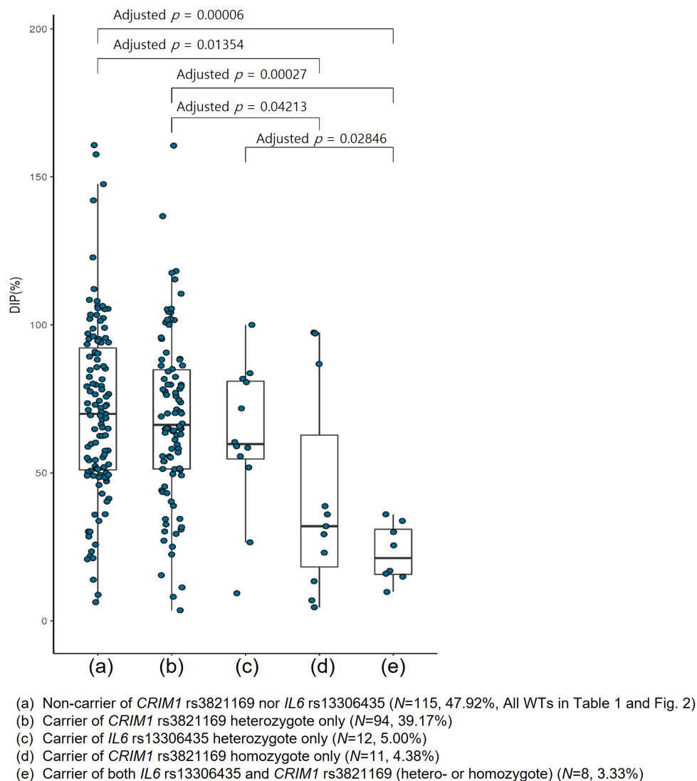
Figure 1. Distribution of the tolerated last-cycle 6-MP DIPs (%) of CRIM1 rs3821169- and/or IL6 rs13306435-variant carrier vs. non-carrier subgroups among 240 pediatric ALL subjects with both NUDT15 and TPMT WTs.
