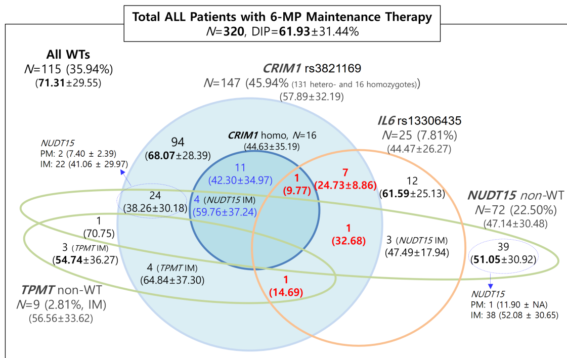
Figure 2. Distribution of the last-cycle 6-MP DIP of pediatric ALL patients according to NUDT15 , TPMT , CRIM1 and IL6 pharmacogenetic subgroups (N=320). Green circles depict NUDT15 and TPMT metabolizer phenotypes and blue and orange circles represent CRIM1 rs3821169 and L6 rs13306435 genotype subgroups, respectively. Of the 320 patients, 115 with no pharmacogenetic variants exhibited higher 6-MP DIPs (71.31%) than 72 NUDT15 (47.14%), 9 TPMT (56.56%), 147 CRIM1 (57.89%), and 25 IL6 (DIP=44.47%) non-WTs. Subjects with both CRIM1 and IL6 variants (N=10, 3.13%) exhibited the lowest DIPs (9.77~32.68%, in red numbers). Numbers are number of subjects and 6-MP DIPs (mean±S.D.). ALL: Acute Lymphoblastic Leukemia, WT: Wild Type, non-WT: non wild-type, i.e., poor or intermediate metabolizers for NUDT15 and TPMT , DIP: Dose Intensity Percentage.
