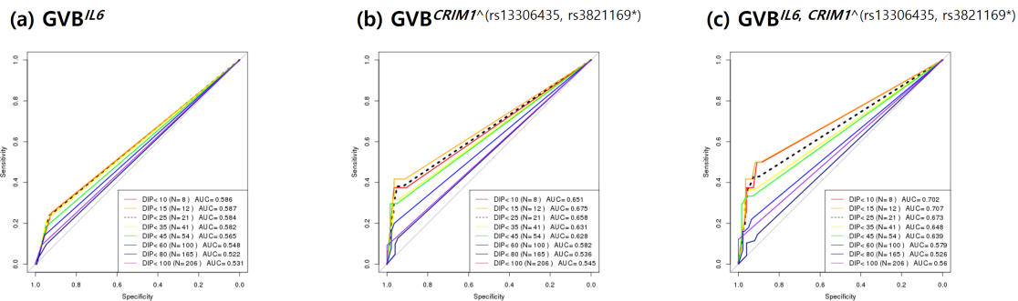
Figure 3. ROC analysis of IL6 , CRIM1 , and their combined prediction accuracies for thiopurine intolerance among pediatric ALL subjects with both wild-type NUDT15 and TPMT genes (N=240).
