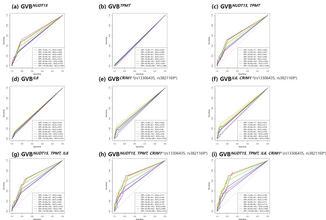
Figure 4. Prediction accuracy profile of single- and multi-gene models for thiopurine intolerance in the whole pediatric ALL subjects (N=320). Single-gene prediction models of (a) NUDT15 and (b) TPMT were outperformed by (c) the two-gene combined model and of (d) IL6 and (e) CRIM1 by (f) IL6-CRIM1 combined model. Three-gene models of NUDT15, TPMT and (g) IL6 and (h) CRIM1 were outperformed by (i) all four-gene combined model. Overall the final (i) four-gene combined model outperformed other models for predicting thiopurine intolerance at all DIP levels in pediatric ALL subjects (N=320). AUCs for predicting the last-cycle 6-MP DIP (%) were measured at 8 cutoff levels of ( \leq 10\% , \leq 15\% , \leq 25\% , \leq 35\% , \leq 45\% , \leq 60\% , \leq 80\% , and \leq 100\% ). ALL: Acute Lymphoblastic Leukemia, DIP: Dose Intensity Percentage, AUC: Area under the Receiver Operating Characteristics Curve, GVB: Gene-wise Variant Burden.
