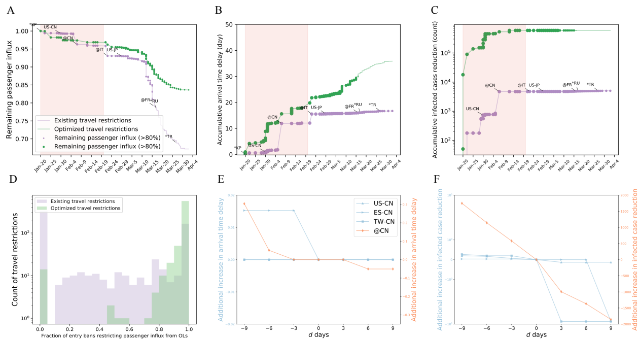
Figure 5: Effectiveness of optimized travel restrictions, and time sensitivity of travel restrictions' effectiveness. (A)(B)(C) Remaining passenger influx (A), arrival time delay (B), and infected case reduction (C) caused by optimized travel restrictions. Each optimized travel restriction, which comprises a set of entry bans, is the non-dominated solution with NSGA-II. (D) Distribution of optimized travel restrictions' fraction of entry bans restricting passenger influx from outbreak locations (OLs). (E)(F) Additional increases in arrival time delay (E) and additional increases in infected case reduction (F), if travel restrictions' occurrence dates are randomized with d days before or after the original occurrence date.
