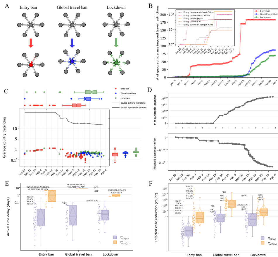
Figure 2: Country distancing , outbreak locations (OLs), and three types of travel restrictions (i.e., entry ban, global travel ban, lockdown) from Jan-20 to Apr-4. (A) Illustration of how the entry ban, global travel ban, and lockdown reduce airline passenger influx. When the colored areas (in red, blue, and green) enforce the entry ban, the global travel ban, or the lockdown, the passenger influx on corresponding links are reduced (solid links change to dotted links). (B) Number of geographic areas that imposed travel restrictions as of Apr-4. The embedding subplot presents the number of geographic areas that imposed entry bans to the main five areas. (C) Average country distancing ( D_{G|(N_I(t_s), F(t_s))} ). Here, D_{G|N_I(t_s)} (black line) is the average country distancing resulting from OLs, and D_{G|F(t_s)} (colored dots) is the average country distancing resulting from travel restrictions. (D) Growth of outbreak locations |N_I(t_s)| , and the decline of passenger influx F(t_s) caused by travel restrictions s \in \mathbb{S} . (E) Arrival time delay (ATD) caused by travel restrictions. (F) Infected case reduction (ICR) caused by travel restrictions. In (E)(F), ATD and ICR are visualized for two groups, that is, the average of ATD ( T_{G|F(t_s)}^* ) / ICR ( I_{G|F(t_s)}^* ) for the world, and the ATD ( T_{n_s|F(t_s)}^* ) / ICR ( I_{n_s|F(t_s)}^* ) of geographic area n_s which imposed s^{th} travel restriction. Among the marks, for example, "US-CN" represents the entry ban imposed by US to CN (mainland China); "*KP" represents the global travel ban imposed by North Korea; "@CN" represents the lockdown imposed by mainland China. For clear visualization, geographic areas are presented by two-letter code.
