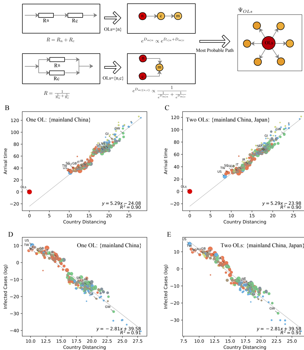
Figure 1: Understanding the country distancing and its correlation with arrival times and infected cases in the presence of one and multiple outbreak locations. (A) Description of series and parallel laws. (B)(D) Correlation between country distancing and simulated arrival times (B) and correlation between country distancing and simulated infected cases in log transformation (D) when the defined OL set ( N_I ) is {mainland China}. The arrival times and infected cases are simulated with the meta-population susceptible-infected-recovered (SIR) model (31) with the given epidemiological parameters of COVID-19 (32) (see supplementary text). (C)(E) Correlation between country distancing and arrival times (C) and correlation between country distancing and infected cases (E) when the defined OL set ( N_I ) is {mainland China, Japan}. Geographic areas are represented by circles. Those in the same continent are filled in the same color.
