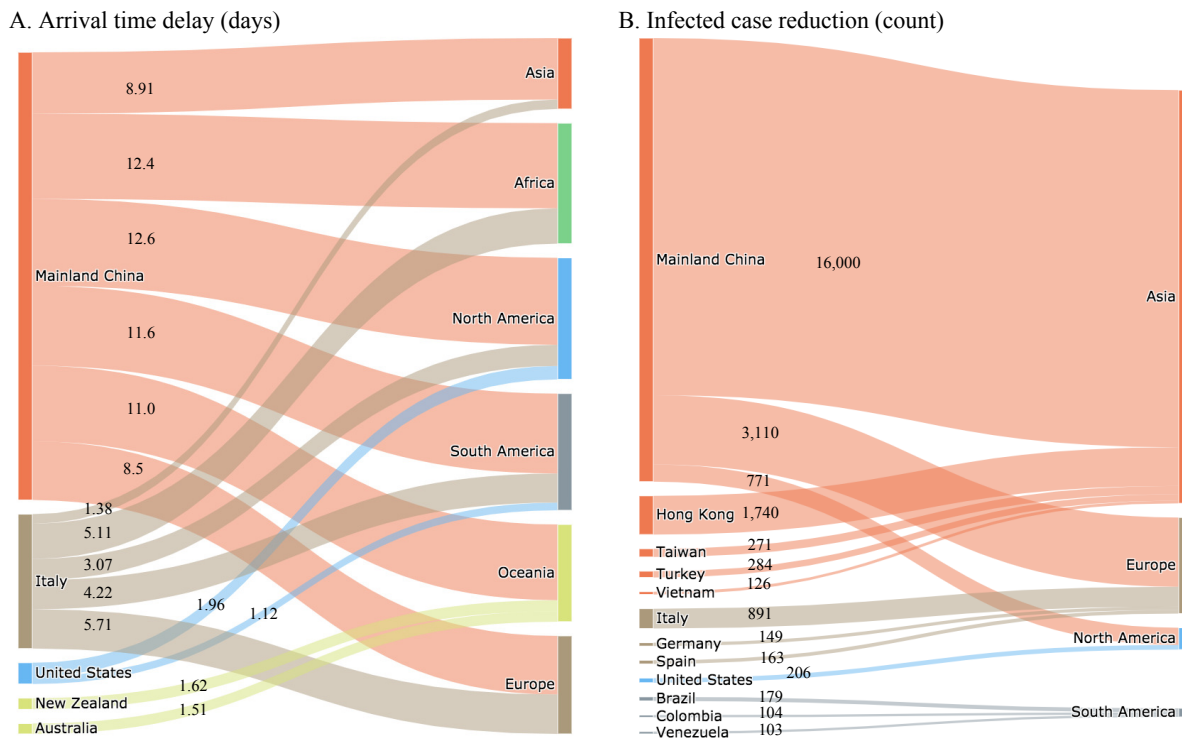
Figure 4: Geographic areas' contribution in arrival time delay (ATD) and infected case reduction (ICR) to different continents till Apr-4. (A) Arrival time delay (ATD). (B) Infected case reduction (ICR). The flow from the left to the right reflects the ATD/ICR ( \sum_{m \in N^c, n_s} T_{m|F(t_s)}^* / |N^c|, \sum_{m \in N^c, n_s} I_{m|F(t_s)}^* / |N^c| ) of the right continents for travel restrictions imposed by the left areas ( n_s ). The notation N^c denotes the set of geographic areas in the six continents and c \in \{\text{Asia, Africa, North America, South America, Oceania, Europe}\} . For clear visualization, only the flows with ATD > 1 and ICR > 100 are presented.
