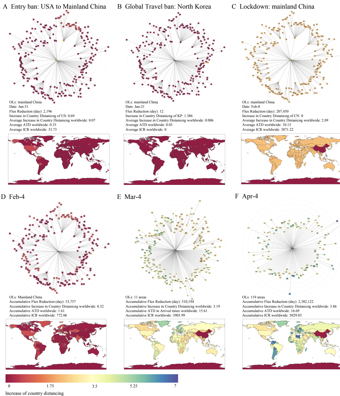
Figure 3: Visualizations of shortest-path tree \Psi_{OLs} for the examples of travel restrictions and snapshots of geographic areas with an increase in country distancing till Feb-4, Mar-4, and Apr-4 (DEF). (A) Entry ban imposed by the US to mainland China on Jan-31. (B) Global travel ban imposed by North Korea on Jan-21. (C) National lockdown imposed by mainland China on Feb-8. (D)(E)(F) Geographic areas with an increasing in country distancing as of Feb-4 (D), Mar-4 (E), and Apr-4 (F). Notably, OLs represent the set node of outbreak locations. The radius differs in each shortest path tree.
