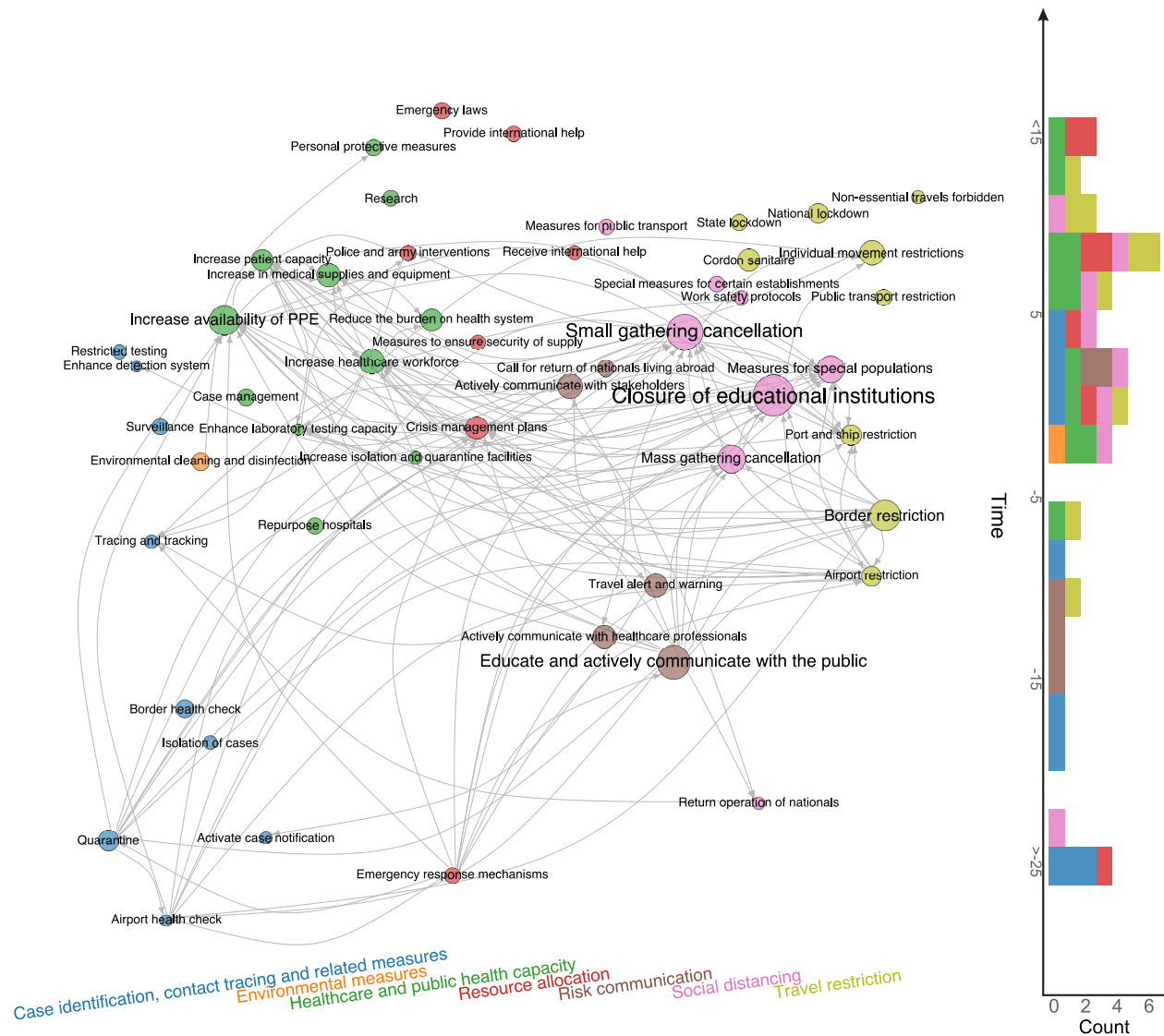
Figure 3: Time-ordered NPI co-implementation network across countries. Nodes are categories (L2) with colour indicating the theme (L1) and size being proportional to the average effectiveness of the intervention. Arrows from nodes i to j represent that countries which have already implemented intervention i tend to implement intervention j later in time. Nodes are positioned vertically according to their average time of implementation (measured relative to the day where the country reached 30 confirmed cases) and horizontally according to their L1 theme.
