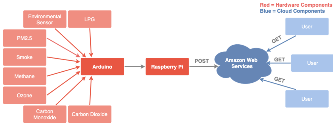
Fig. 3. System architecture chart: Red denotes hardware components while blue represents cloud computing components
