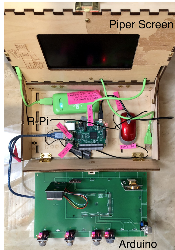
Fig. 1. System hardware, including a monitor in a Piper Kit box, a Raspberry Pi, an Arduino, and a PCB.
