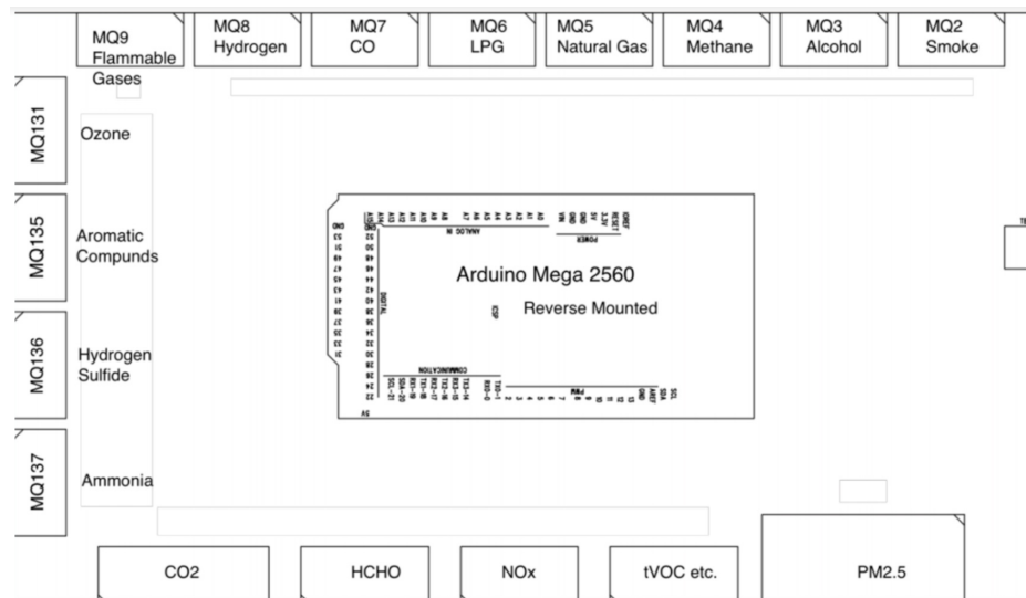
Fig. 2. Circuit diagram of the PCB. , This board holds the Arduino and 17 environmental sensors.
