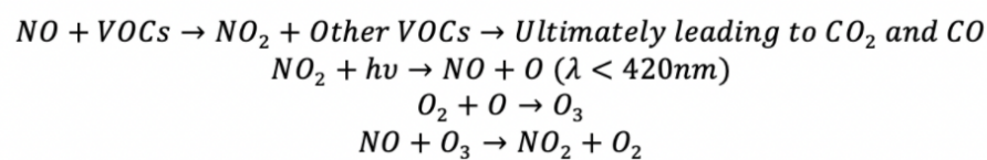
Fig. 15. Ground Ozone Creation: Chemical reactions showing VOCs reacting with Nitrogen Oxides to create ground-level ozone.
